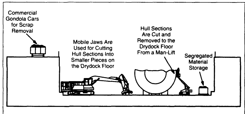
Figure 2.3: Schematic of Submarine Hull Dismantlement in a Dry Dock
