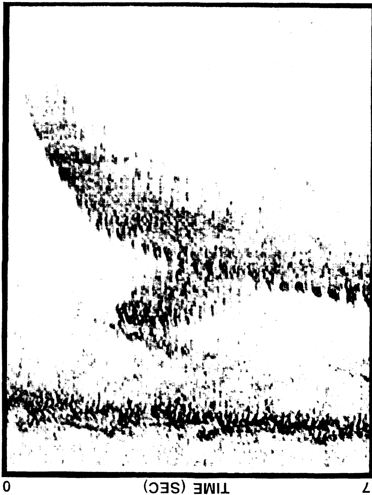
BEARDED SEAL, TRILLS FROM TWO (AFB-15 Hz)
