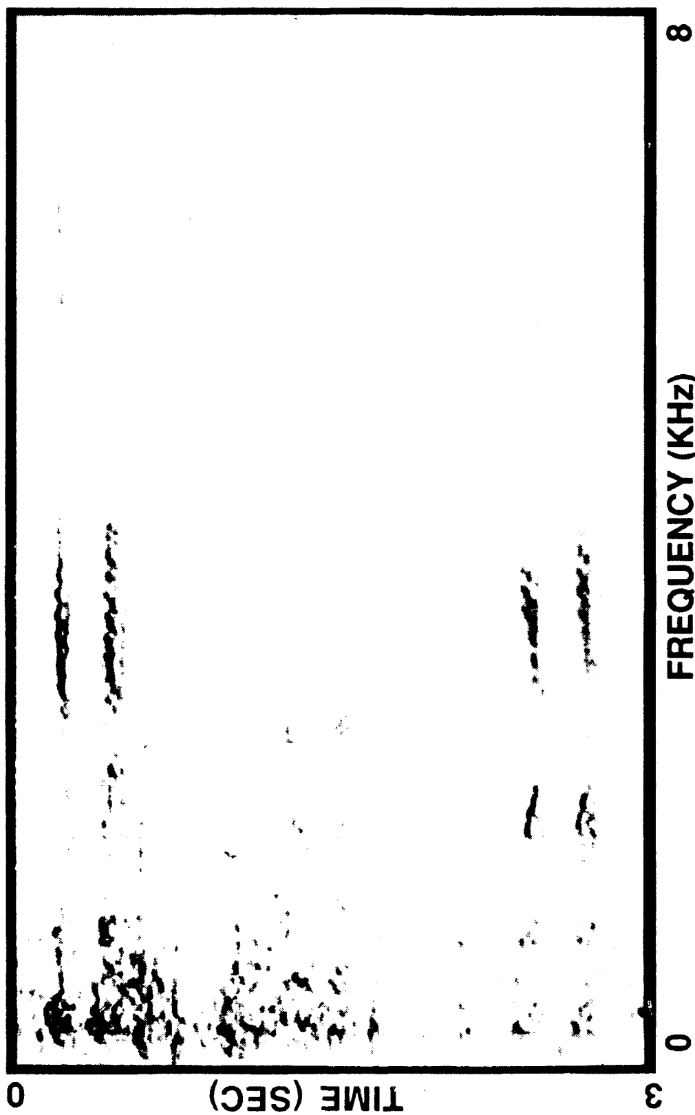
HARP SEAL, QUACKS, 3 PAIRS (AFB-30 Hz)
