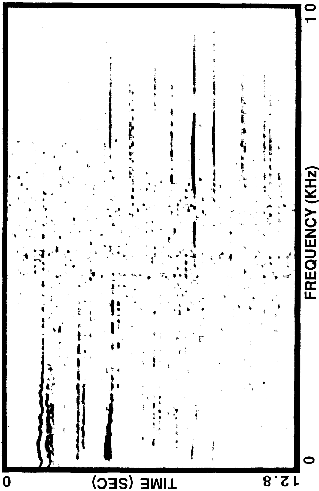
ICE STRESS CRACKS (AFB-37.5 Hz)
