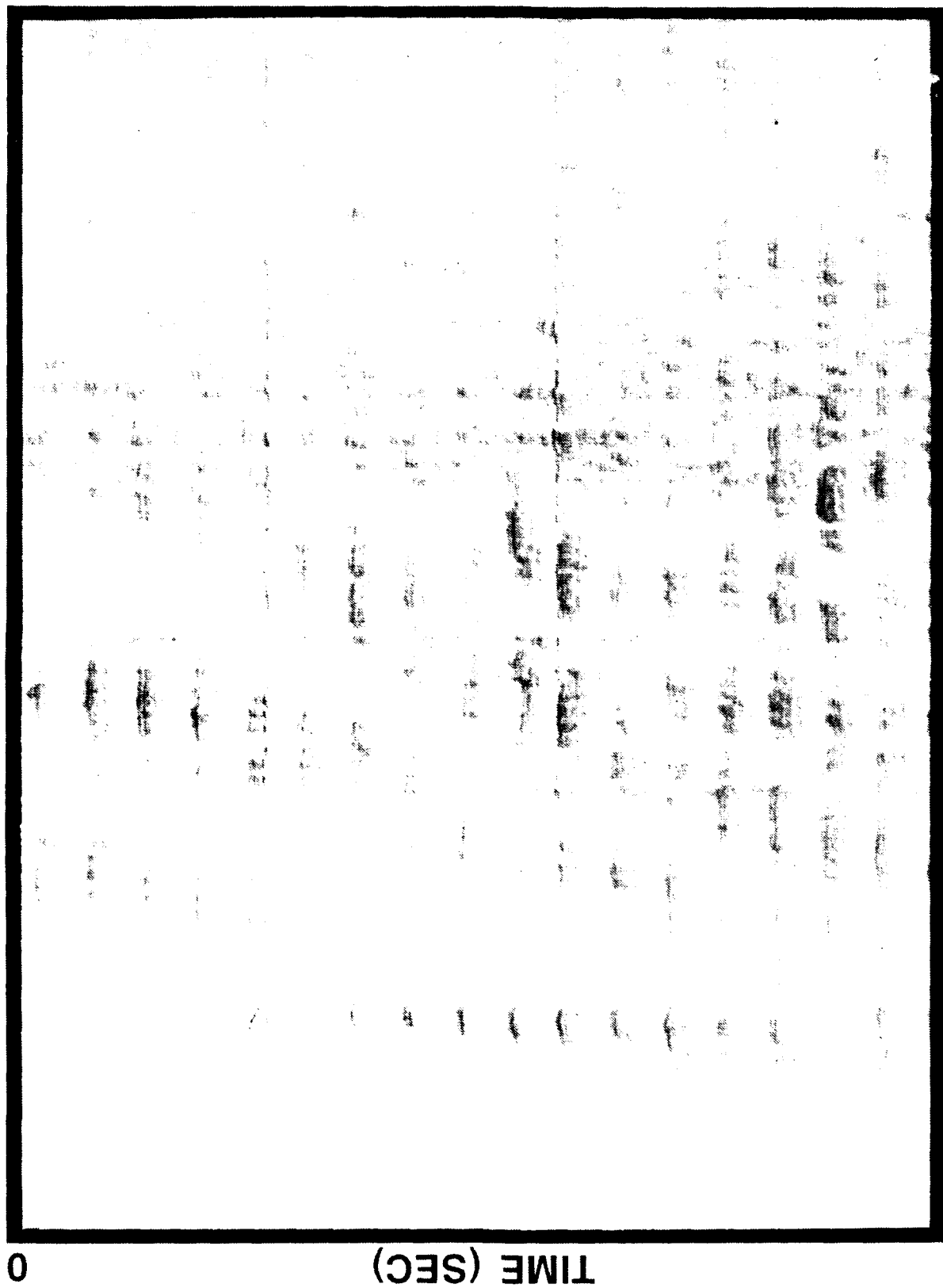
FREQUENCY (KHz) MINKE WHALE PULSE TRAIN (AFB-3.75 Hz)
