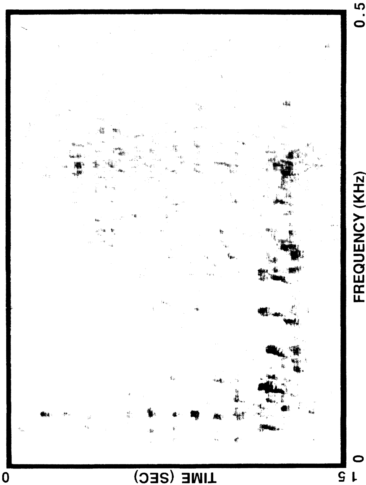
HUMPBACK WHALE GRUNTS. MOAN (AFB-1.88 Hz)
