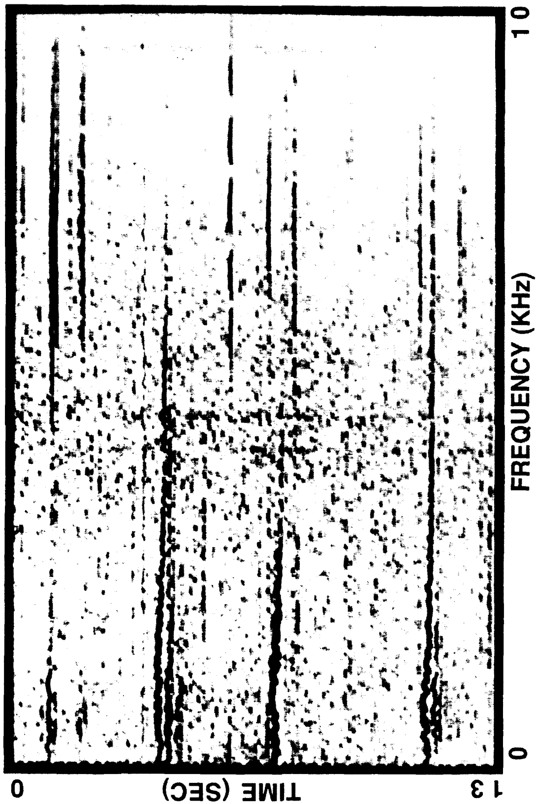
ICE STRESS CRACKS (AFB-37.5 Hz)
