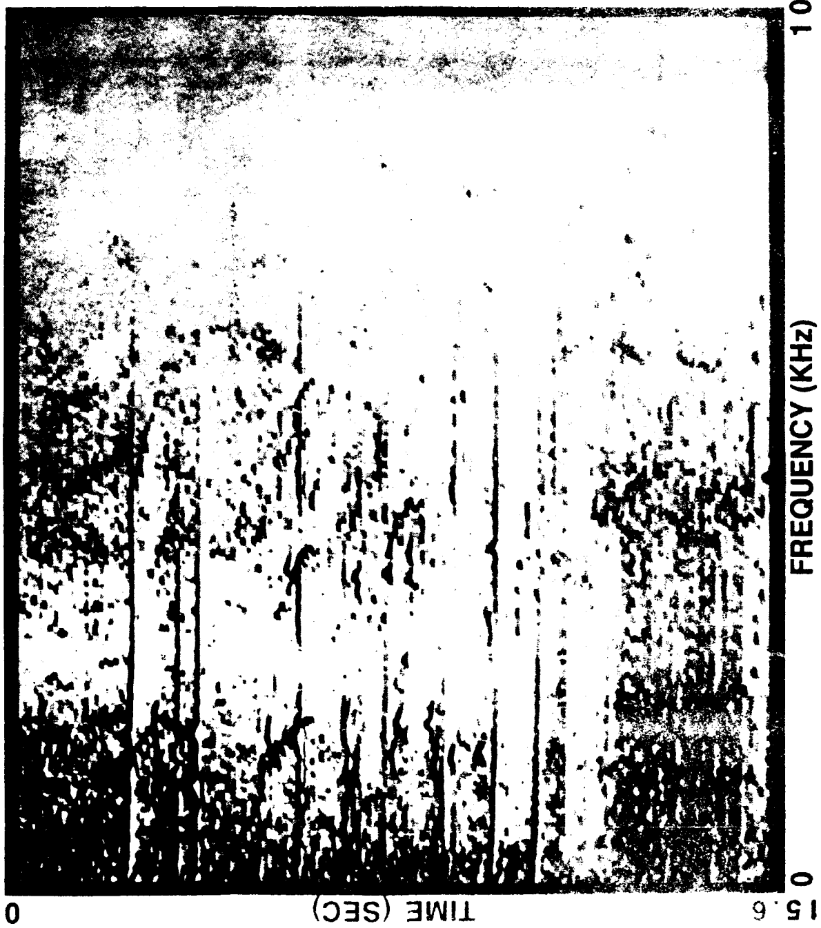
BELUGA CHIRPS, WHISTLES (AFB-37.5 Hz)
