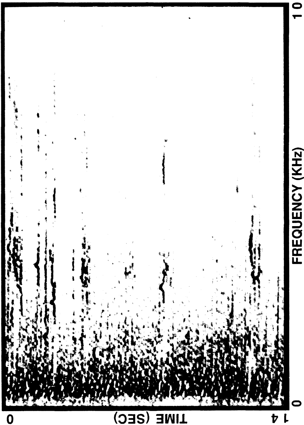
LONGFIN PILOT WHALE CLICKS, CHIRPS (AFB-37.5 Hz)
