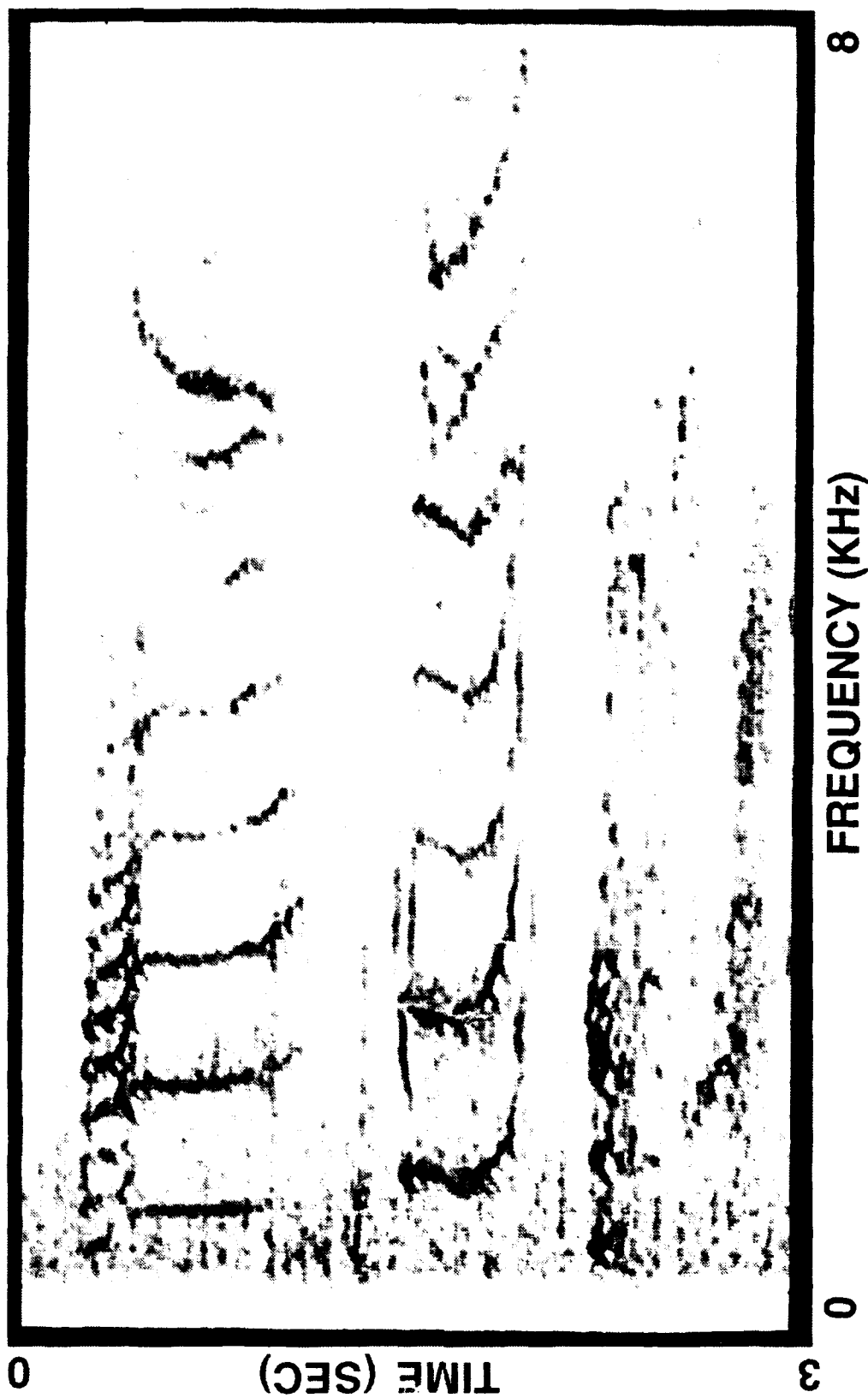
KILLER WHALE COMPLEX SCREAM (AFB-30 Hz)
