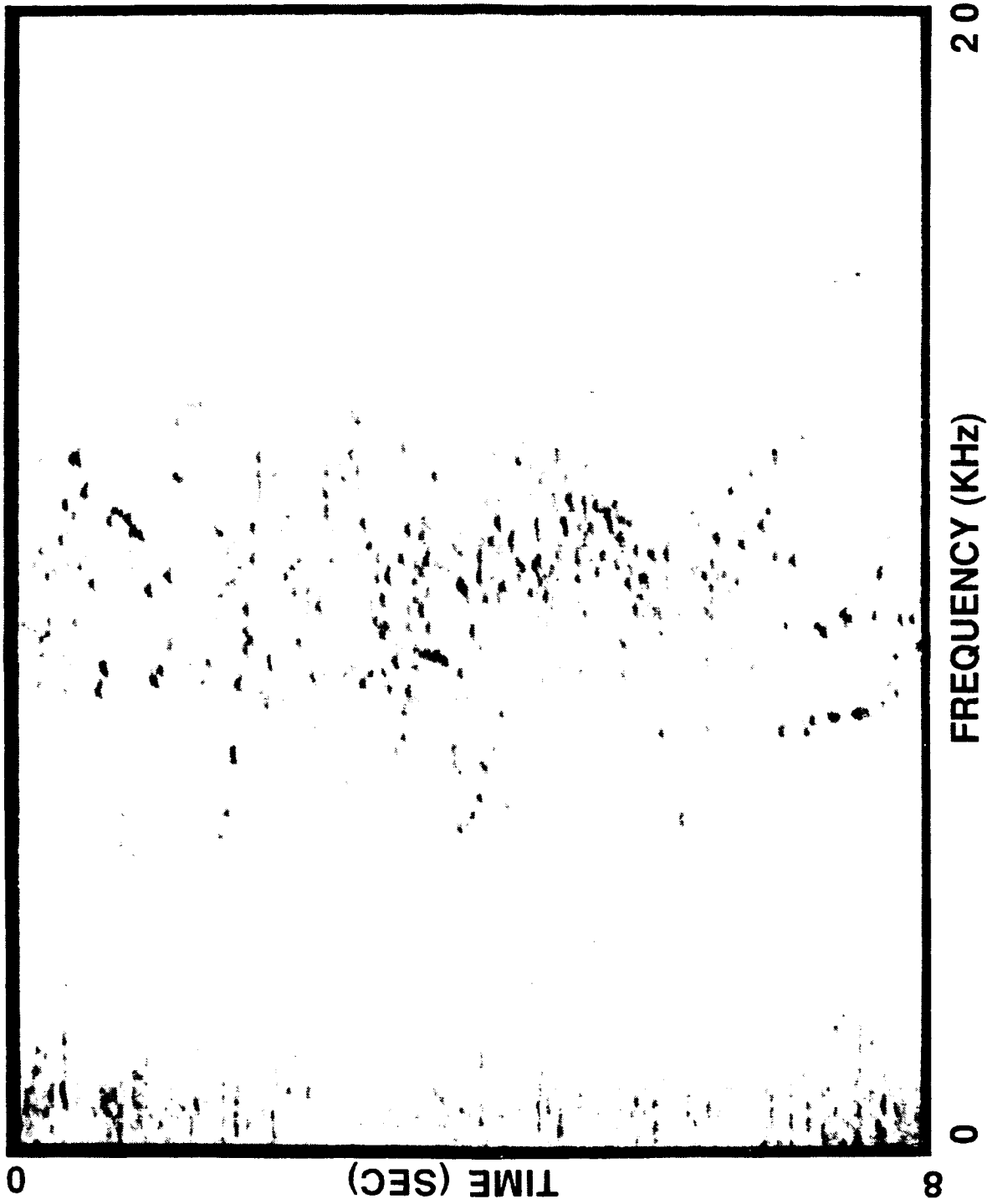
STRIPED PORPOISE WHISTLE CHORUS (AFB-75Hz)
