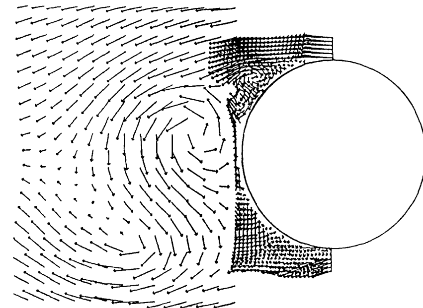
(a) Measured velocity field (Ref. 26)
