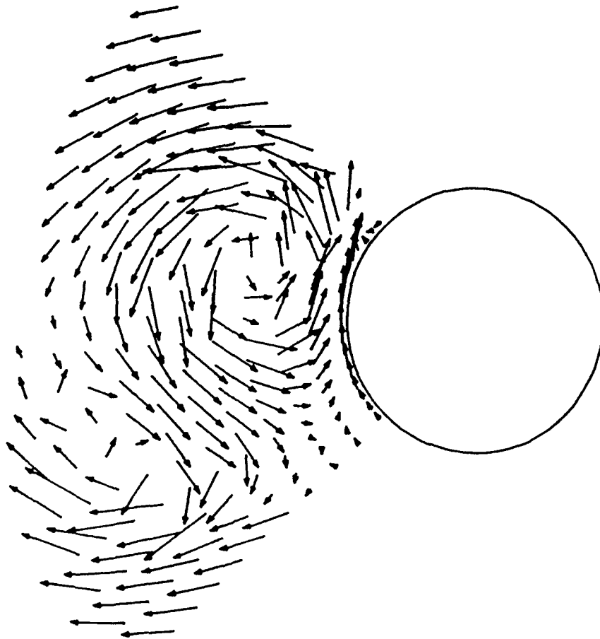
(b) Predicted velocity field
