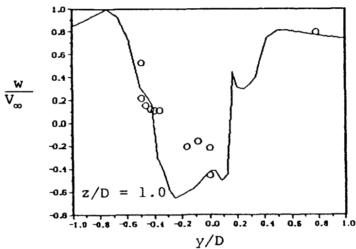
Figure 26.- Measured and predicted velocity field at x/D = 4.9 on the lee side of an ogive-cylinder at \alpha = 37.5^\circ .
