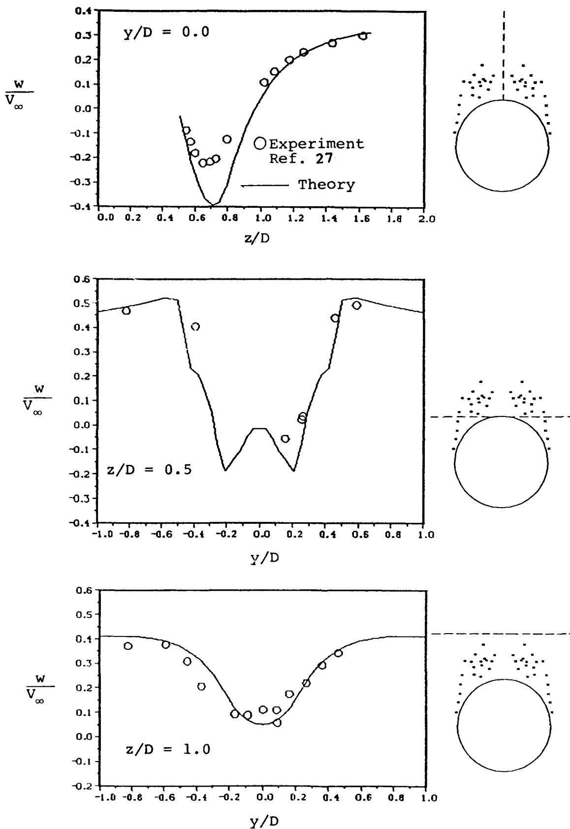
Figure 25 .- Measured and predicted velocity field at x/D = 4.9 on the lee side of an ogive-cylinder at \alpha = 22.4^\circ
