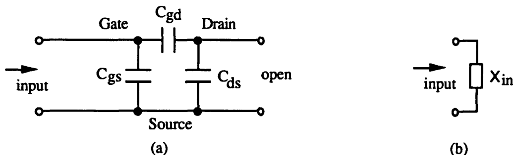
Fig. 2.6 (a) Using the reactive MESFET in one-port circuit (b) Equivalent circuit of (a)
