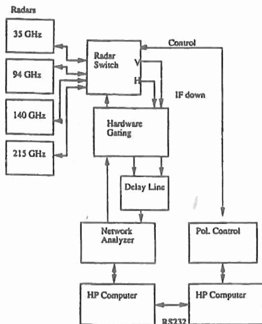
Fig. 1. Block diagram of MMW radar system.
