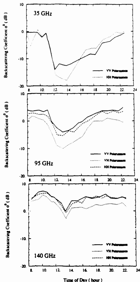
Fig. 6. Backscattering variation measured at 35, 95, and 140 GHz on March 1, 1990. The incidence angle was 40^\circ . The snowpack density was 0.32 \text{ g/cm}^3 , depth was 12 cm, and other parameters are given in Figure 5.
