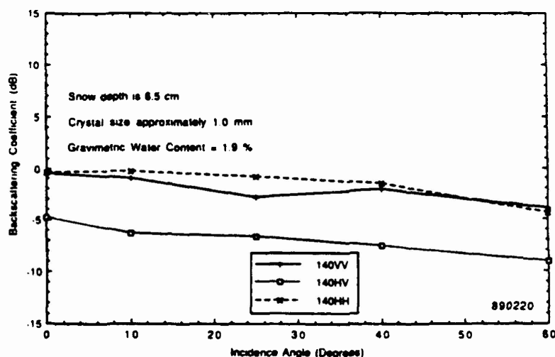
Fig. 10. Angular response of backscatter from fresh wet unmetamorphosed snow at 140 GHz.
