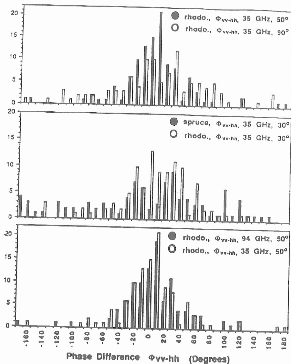
Figure 2: Distributions of \Phi_{vv-hh} at 35 and 94 GHz.
