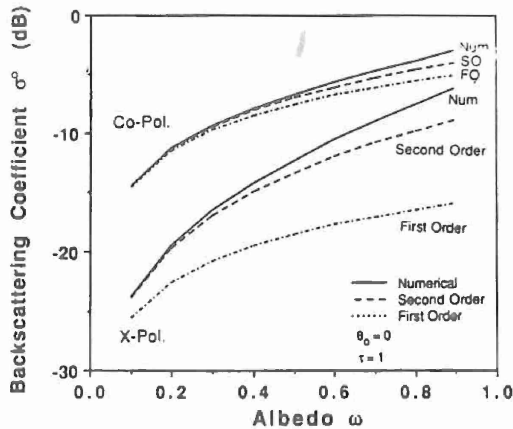
Fig. 7. Backscattering coefficient as a function of albedo at normal incidence, computed with the first-order, second-order, and numerical solutions.
