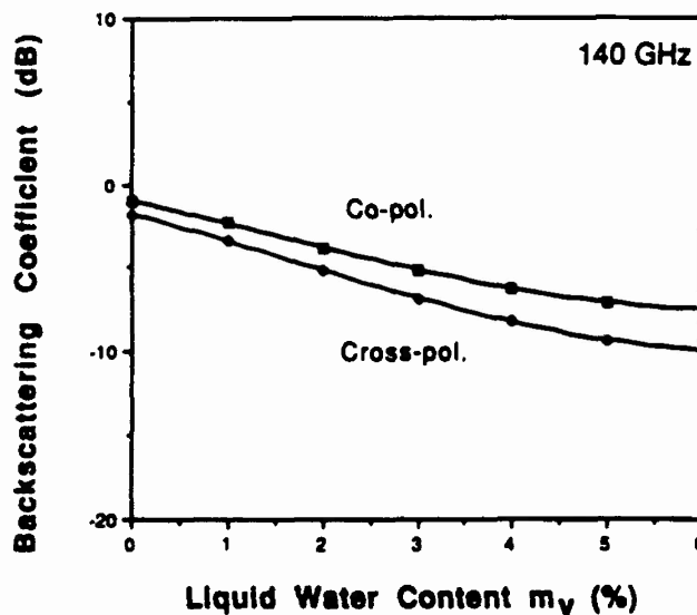
Fig. 4. Backscattering coefficient \sigma_{vs} versus m_v at 95 and 140 GHz. Symbols are the calculated values based on the radiative transfer theory. Solid lines are third-order polynomial curve fits to calculated results. The incident angle is \theta_o = 40^\circ and the incident wave is horizontally polarized.
