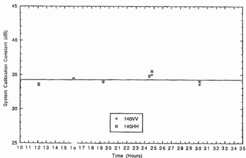
Fig. 4. System calibration constant over diurnal cycle, February 27, 28, 1989 (starting 10 A.M.).
