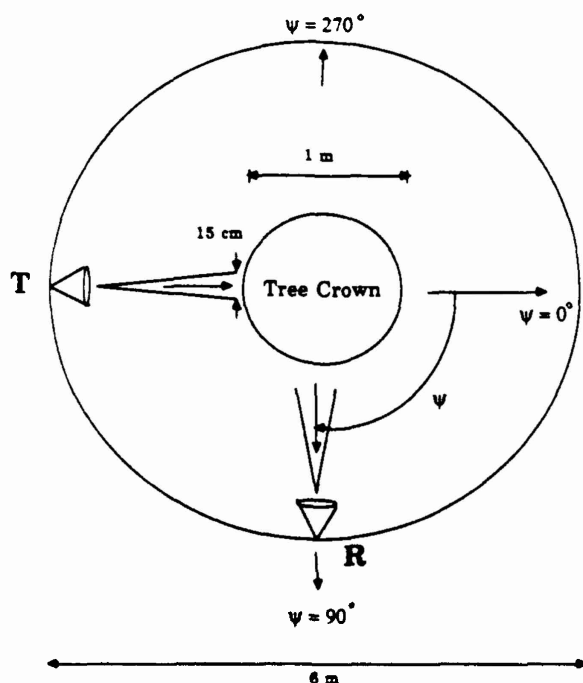
Fig. 1. Configuration used for measuring bistatic scattering from tree foliage. The tree was placed on a rotating platform, the transmitter was in a fixed location, and the receiver could be set at any angle \psi .
