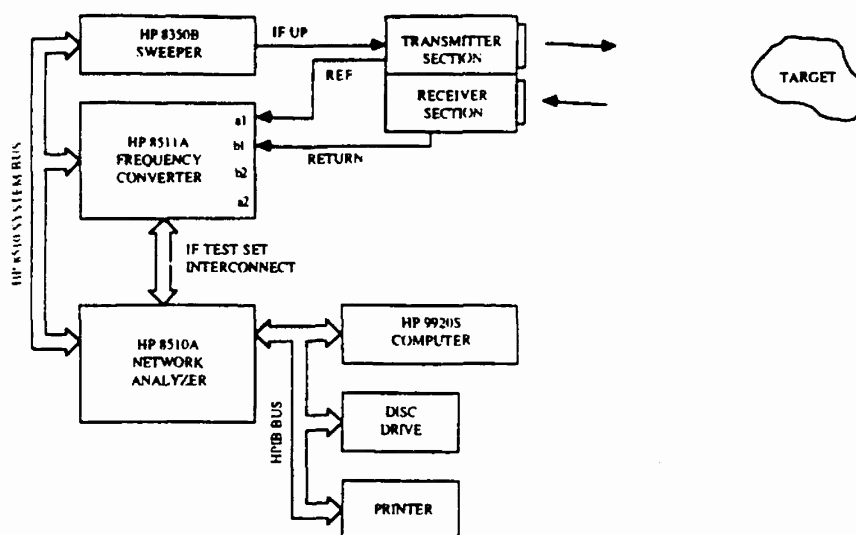
Fig. 1. Millimeter-wave scatterometer system.
