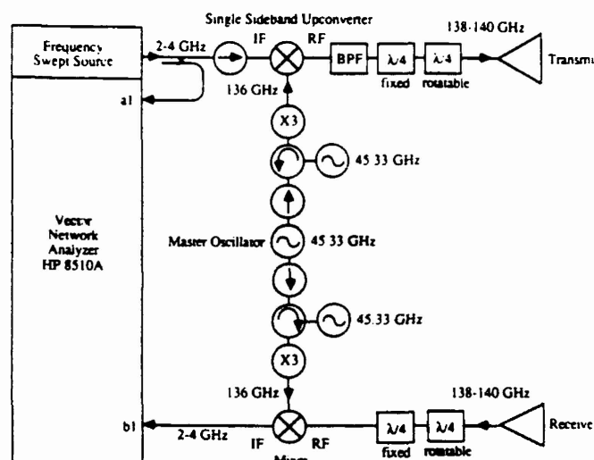
Fig. 2. 140-GHz scatterometer front end.
