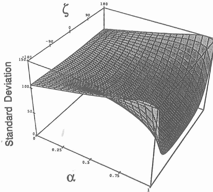
Figure 4: The standard deviation of the co-polarized phase difference as a function of \alpha (degree of correlation) and \zeta (coherent-phase-difference).
