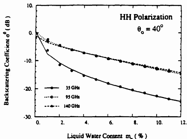
Fig. 10. Numerical fits using the form given by (1).
