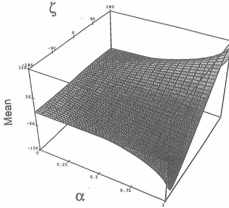
Figure 3: The mean value of the co-polarized phase difference as a function of \alpha (degree of correlation) and \zeta (coherent-phase-difference).
