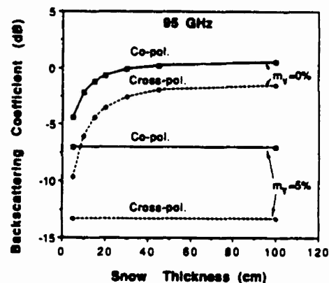
Fig. 6. Backscattering coefficient \sigma_{vs} versus snow thickness. The incident angle is \theta_o = 40^\circ and the incident wave is vertically polarized.
