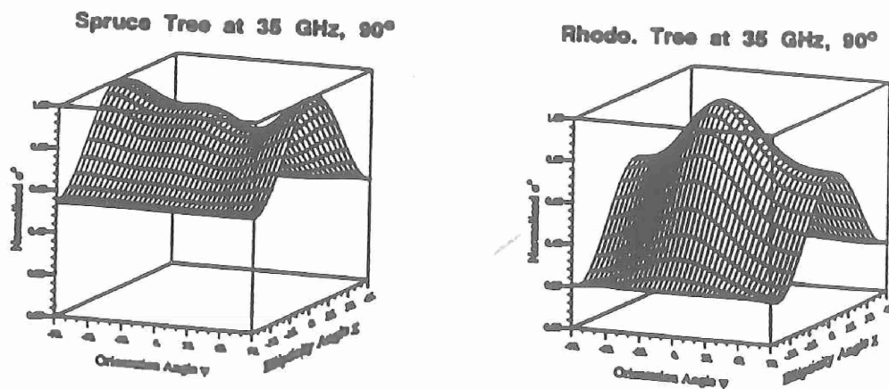
Figure 3: Co-polarized signatures at 35 GHz and 90° incidence angle.
