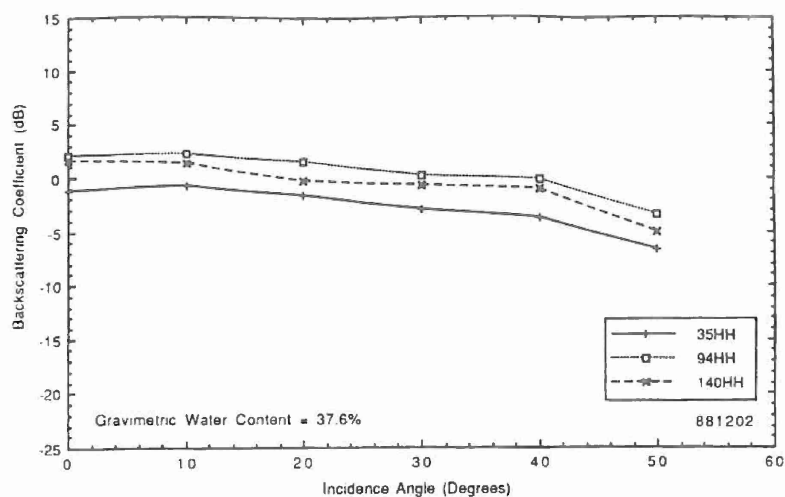
Fig. 6. Measured angular response of pigweed grass at 35, 94, and 140 GHz for HH polarization.
