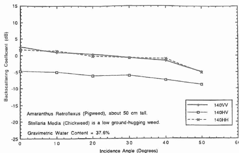
Fig. 5. Measured backscatter angular response of pigweed ( Amaranthus retroflexus ) grass over Stellaria media at 140 GHz.
