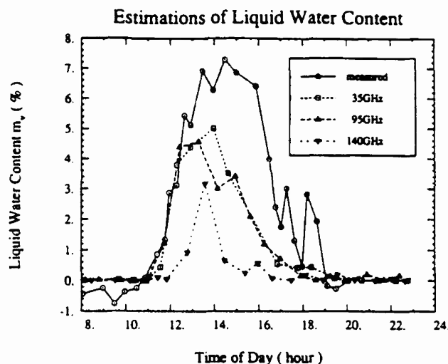
Fig. 8. Diurnal variation of liquid water content. The plot labeled "measured" refers to the value of m_v of the top 5-cm layer as measured by the freezing calorimeter. The other three plots refer to m_v as predicted by the model using the radar observations at the noted frequencies (with hh polarization and \theta_0 = 40^\circ ).
