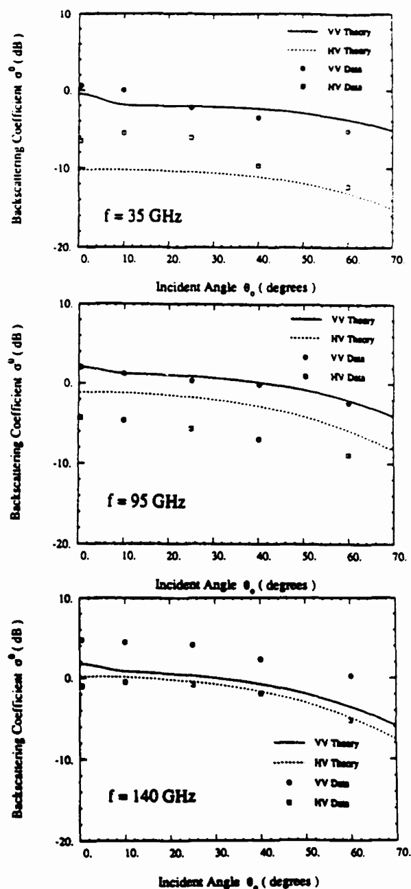
Fig. 1. Measured and calculated backscattering coefficient for a dry snowpack with the following parameters: depth, 12 cm; snow density, 0.2 \text{ g/cm}^3 ; mean crystal diameter, 1 mm; and rms surface slope, 0.07.
