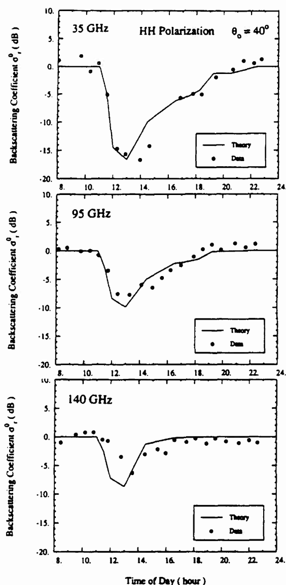
Fig. 11. Comparison of the diurnal variation of the measured backscattering coefficient (relative to dry snow) with that using the hybrid first-order—numerical model.
