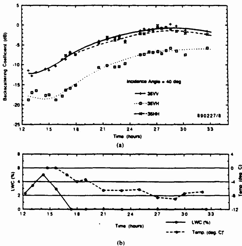
Fig. 12. Diurnal measured temporal variation: (a) 35-GHz radar backscatter, and (b) air temperature and snow gravimetric liquid water content (top 5-cm layer).
