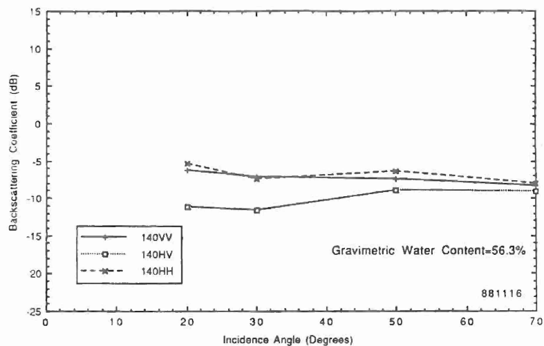
Fig. 7. Measured angular response of white cedar trees at 140 GHz.
