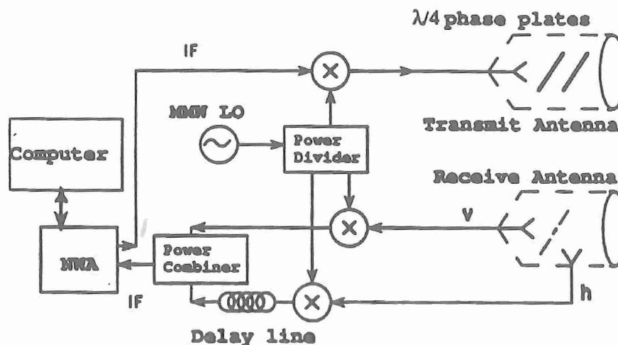
Figure 1: Block diagram of the COR system
