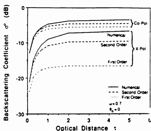
Fig. 8. Variation of backscattering coefficient with optical thickness \tau .
