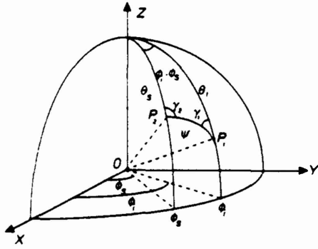
Fig. 5. Coordinate system showing the incident and scattered angles, (\theta_i, \phi_i) and (\theta_s, \phi_s) , and their relation to \psi .
