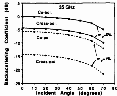
Fig. 5. Backscattering coefficient \sigma_{vs} versus incidence angle at 35 GHz for a 0.45-m-thick layer.
