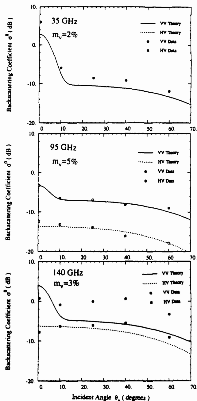
Fig. 2. Measured and calculated backscattering coefficient for a wet snowpack with the following parameters: depth, 27 cm; snow density, 0.4 \text{ g/cm}^3 ; mean crystal diameter, 1 mm; and rms surface slope, 0.07.
