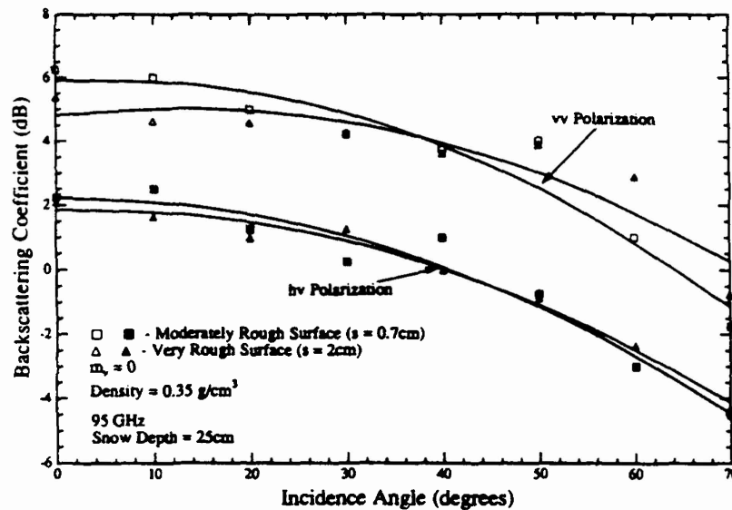
Fig. 3. Measured backscattering coefficient of a dry snowpack at 95 GHz under two different surface roughness conditions.
