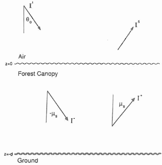
Fig. 6. Geometry of the scattering problem.
