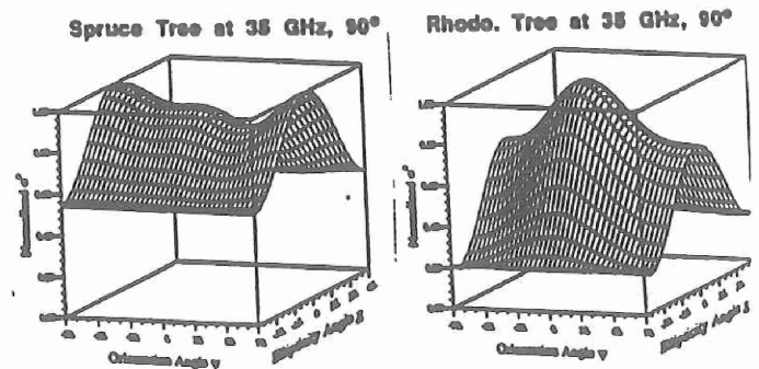
Fig. 7. Co-polarized signatures at 35 GHz and 90° incidence angle.
