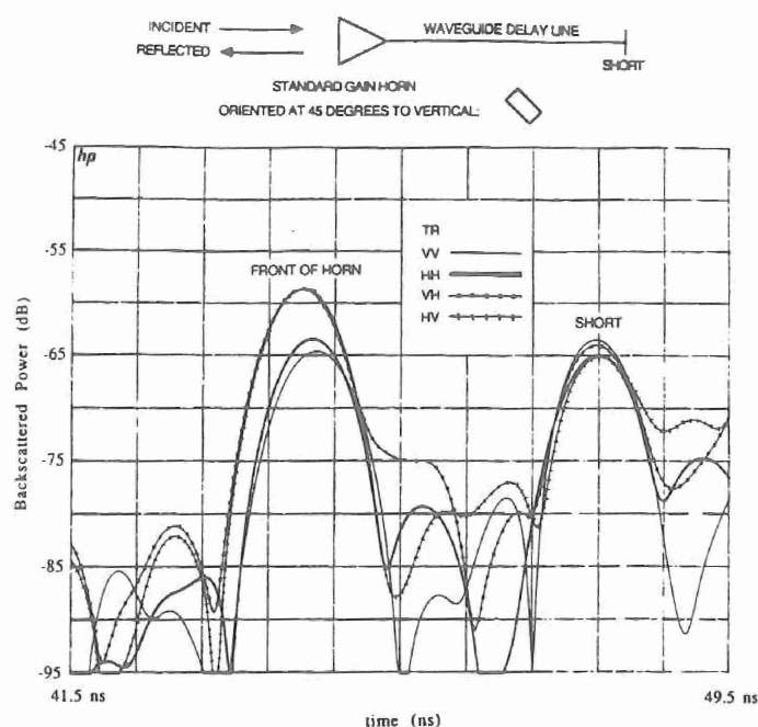
Fig. 3. Measured backscatter response of 140-GHz system when observing pyramidal horn antenna connected to short through 38.1-cm-long waveguide section.
