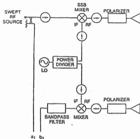
Fig. 3. Block diagram of 140 and 215 GHz radars.
