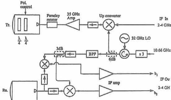
Figure 2 Block Diagram of the 35 GHz Radar Frontend.
