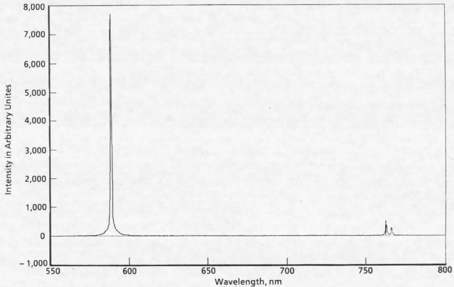
Figure 11. Spectral emission data taken above a stainless steel tube placed in a H 2 -air flame.
