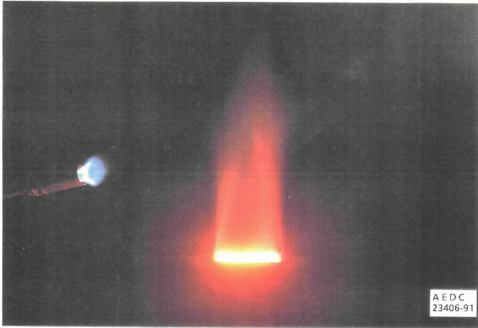
Figure 7. Non-filtered photograph of H_2 -air flame on flat flame burner.
