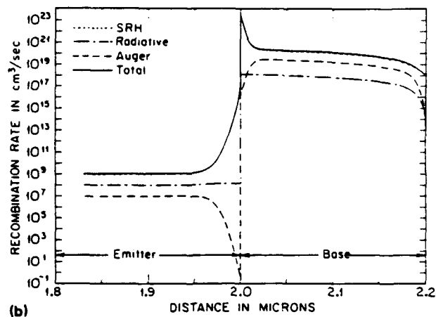
FIG. 1. Calculated (a) energy-band diagram and (b) recombination rate near the heterojunction of a typical N -InP/ p^+ -In 0.53 Ga 0.47 As/ n -In 0.53 Ga 0.47 As HPT, biased at V_{CE} = 2 V and illuminated by P_i = 10 nW, 1.3- \mu m wavelength light. The intrinsic quasi-Fermi level ( \phi_i ), and the electron (hole) quasi-Fermi level \phi_n ( \phi_p ), are also indicated in (a).
