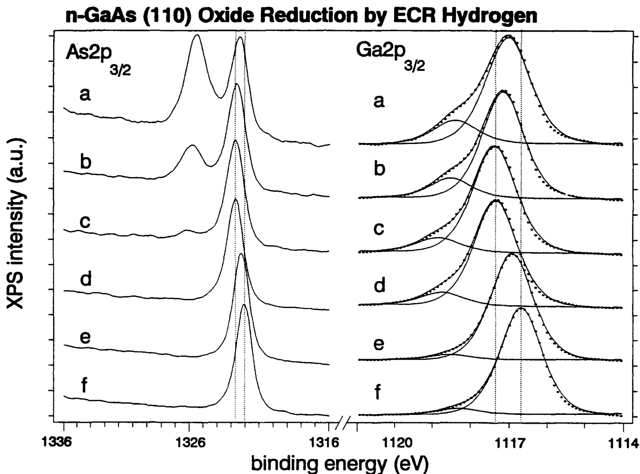
Figure 2. XPS spectra of the As 2p 3/2 and Ga 2p 3/2 core levels from n-GaAs (110): (a) for the initial surface prepared by 50% NH 4 OH (1 min.) after solvent cleaning; (b) after ECR hydrogen plasma processing for 20 min. at room temperature; (c) with an additional 20 min. exposure at room temperature; (d) after further processing for 15 min. at room temperature; (e) after an additional 20 min. processing at 300°C sample temperature; (f) final 20 min. processing at 300°C sample temperature.
