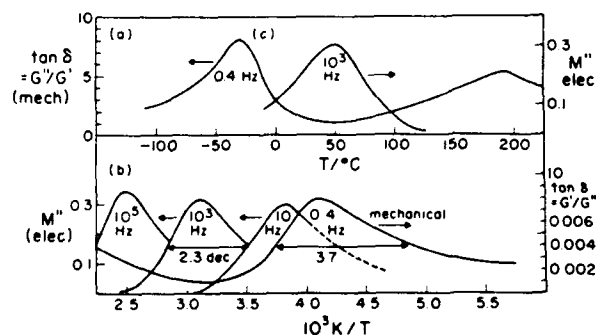
Fig. 11. (a) Comparison of electrical relaxation at 10^3 Hz and mechanical relaxation 0.4 Hz for \text{Na}_2\text{O} \cdot 3\text{SiO}_2 glass during temperature scans. (b) Reciprocal temperature representation of the data of part (a) to permit comparison of spectral shapes and halfwidths. Both electrical and mechanical spectra show KWW form though mechanical spectrum is considerably broader.
