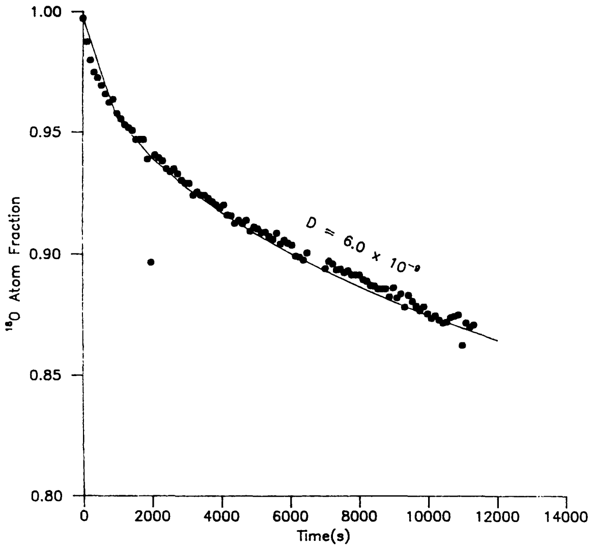
FIGURE F.6. [ 18 O] vs Time Curve for Zr 2.98 Sc .01 La 4 O 12 at 1135°C
