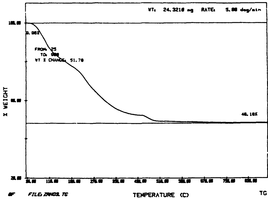
FIGURE B.5. Thermogram for Zirconyl Nitrate
