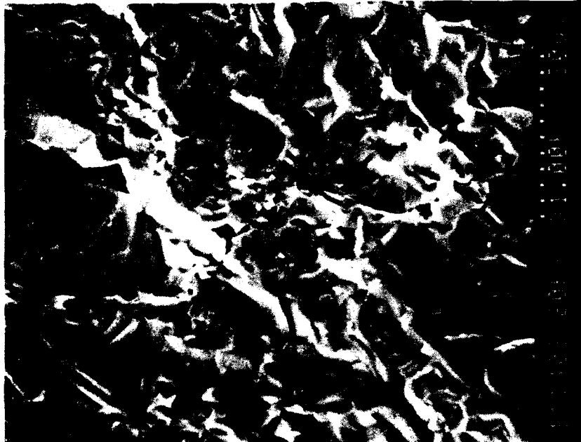
FIGURE A.2. Micrograph of "As Hot-Pressed" Zr_3Y_4O_{12}
