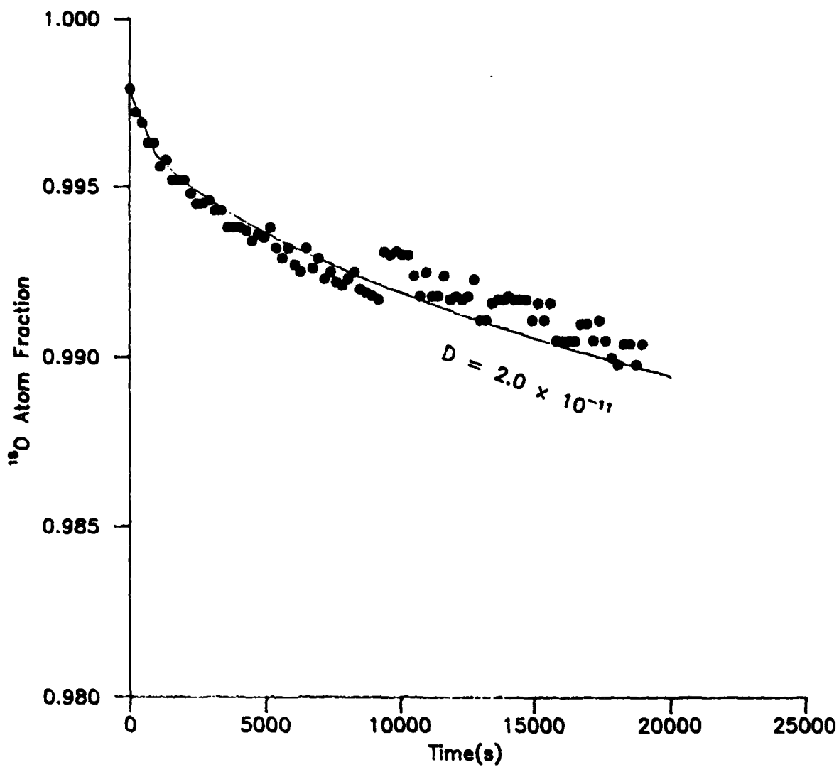
FIGURE F.14. [ ^{18}\text{O} ] vs Time Curve for \text{Y}_2\text{O}_3 at 975°C
