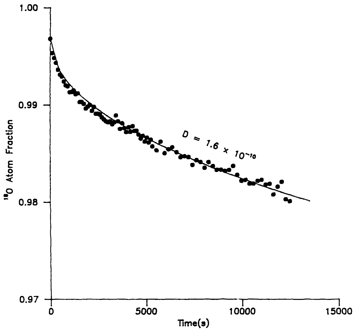
FIGURE F.12. [ 18 O] vs Time Curve for at Y 2 O 3 at 1135°C
