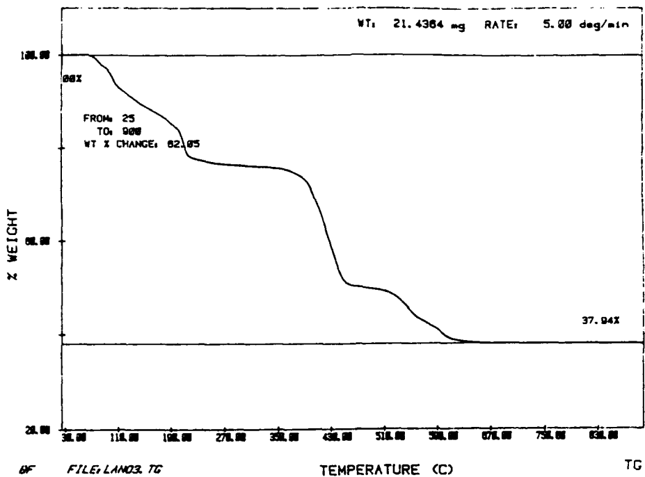
FIGURE B.3. Thermogram for Lanthanum Nitrate Hexaahydrate
