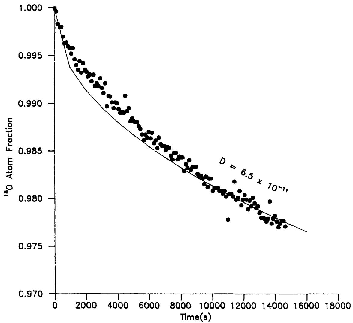
FIGURE F.2. [ ^{18}\text{O} ] vs Time Curve for \text{Zr}_3\text{Sc}_6\text{O}_{12} at 1080^\circ\text{C}
