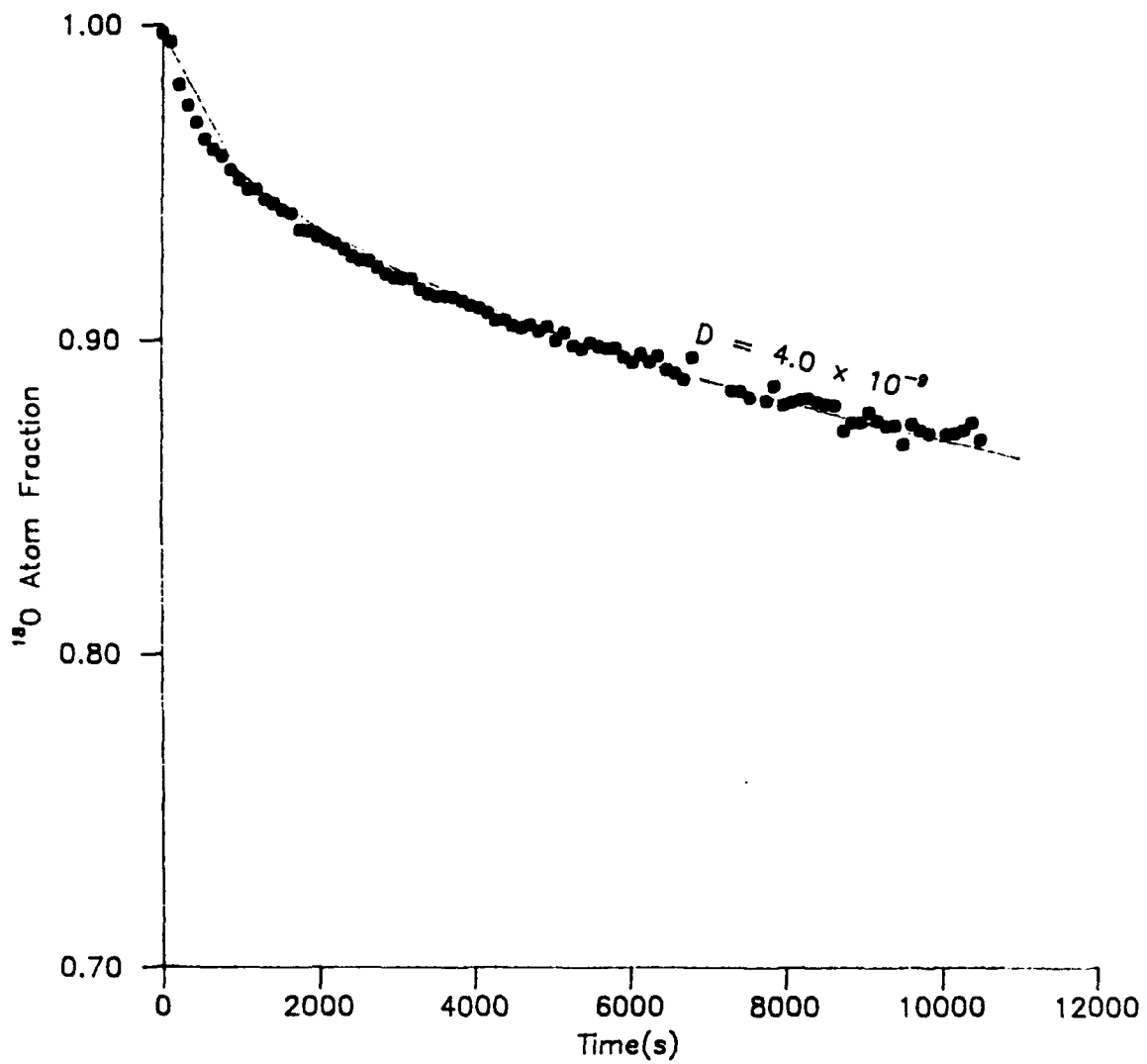
FIGURE F.8. [ ^{18}\text{O} ] vs Time Curve for \text{Zr}_{2.7}\text{Sc}_{.15}\text{Ta}_{.15}\text{La}_4\text{O}_{12} at 1135^\circ\text{C}
