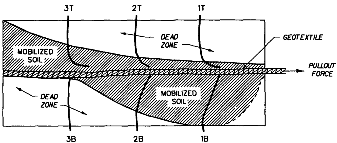
Figure 22. Schematic of sand shafts shown in Figure 21
