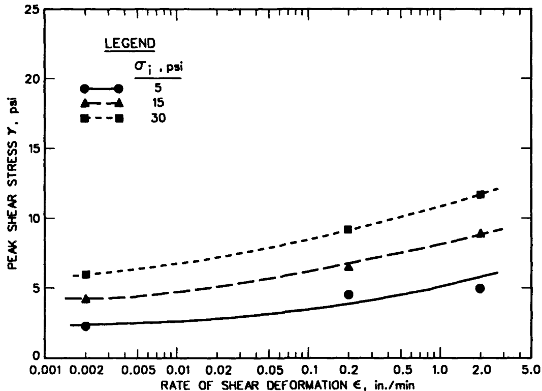
Figure 19. Relationship between the shear stress \tau and the rate of shear deformation at interface of soil and rubber
