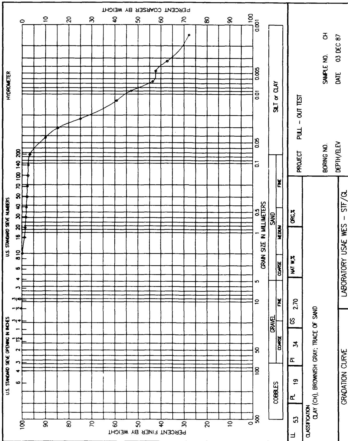
Figure 12. Hydrometer analysis of phase 1 soil
