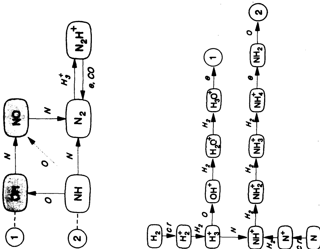
Figure 5 - Chemical pathways for the gas-phase synthesis of NO
