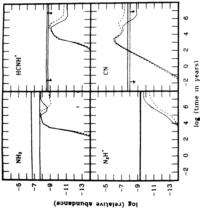
Figure 2 - The observed abundance for NH 3 in L134N is higher than predicted by any of our models. This may be due to grain-surface chemistry which is not considered in our models. On the other hand, TMC's observed abundance is not higher than predicted, perhaps implying that grain-surface chemistry for this molecule in this cloud is not as important. TMC-1 shows very high abundances of the cyanopolynes (HC n N) relative to L134N, perhaps implying that L134N is in a later stage of evolution than TMC-1, since all of these molecules undergo a steep drop in abundance after 10 5 years.
