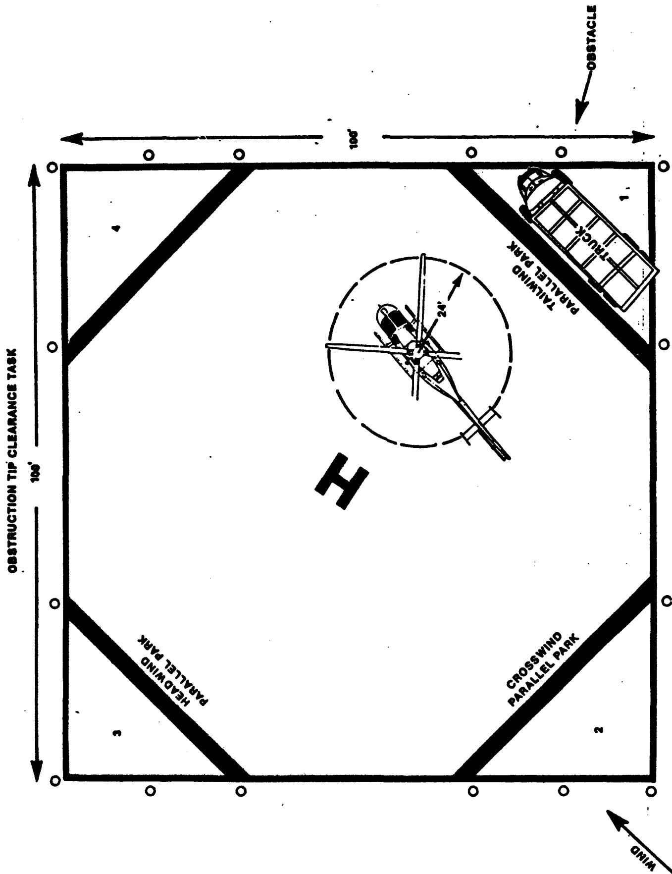
FIGURE 2. HELIPORT LAYOUT FOR PARKING TESTS
