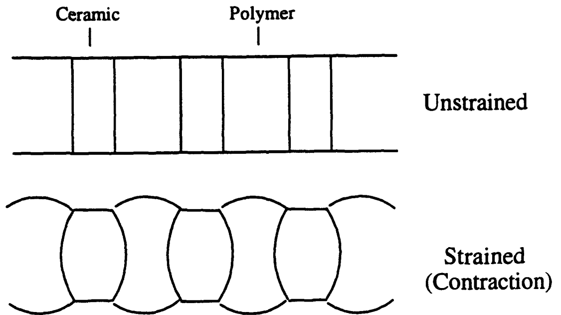
Figure 37 Exaggerated illustration of anti-phase motion resulting from positive Poisson's ratio in ceramic and polymer phases.
