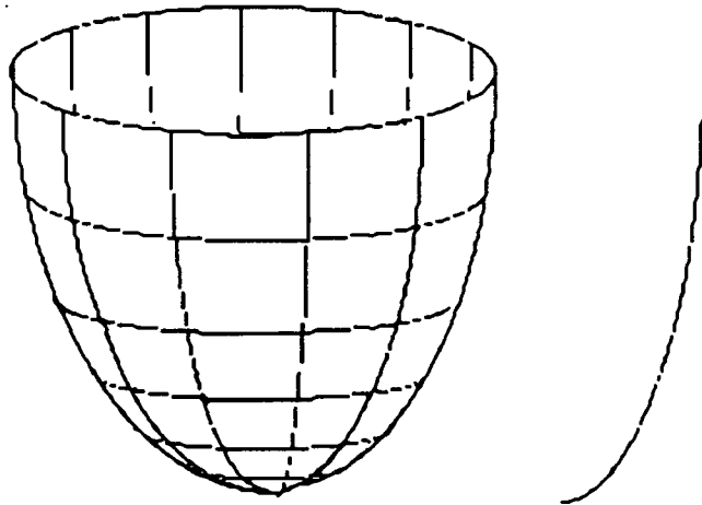
Figure 13: A Surface of Revolution. The curve used to generate the surface has been shifted to the right of the mesh; it was rotated about a line (not visible) inside the surface. The curve at right lies in the drawing plane.
