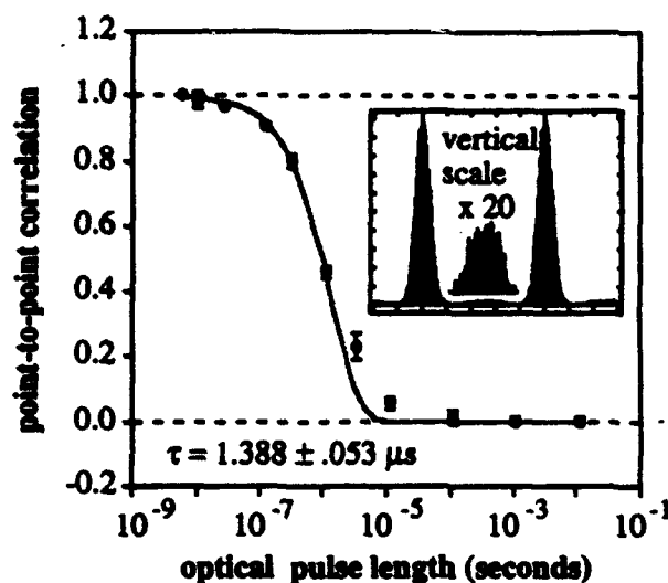
Fig 3 Fit of data to conditional probability function.
