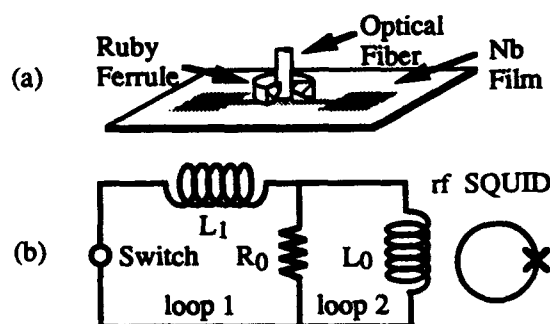
Fig. 1 (a) Laser driven switch. (b) Test circuit for switch. L_0 = 2.24 \mu\text{H} , R_0 = 2 \Omega , L_1 = 0.4 \mu\text{H} , R_{\text{switch}} = 250 \Omega .
