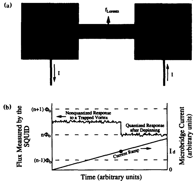
FIG. 2. (a) Current produces a Lorentz force on vortex. (b) SQUID response to vortex depinning by a current ramp through the chip (simulation).
