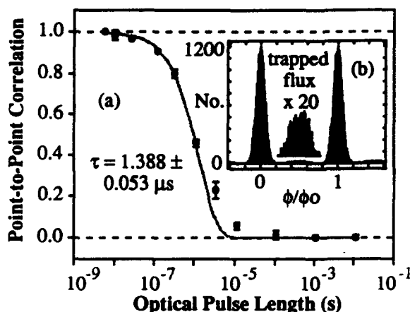
Fig. 2 (a) Point-to-point correlation of flux states with best exponential fit to Eqn. 2. (b) Histogram of 20 000 points of flux data plotted modulo \phi_0 . Inset: trapped flux points magnified \times 20 .
