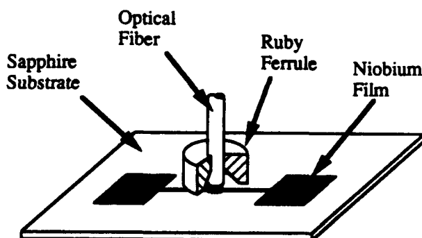
Figure 2. Positioning of the optical fiber over the meander.
