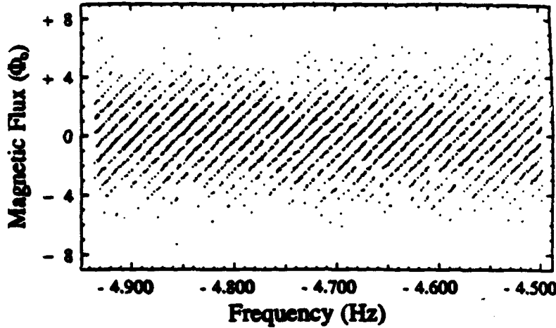
Fig 4 Flux quantum data during slow ramp of spin speed.
