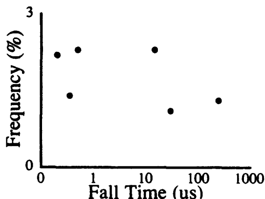
Figure 11. Frequency of trapped flux versus laser pulse fall time.
