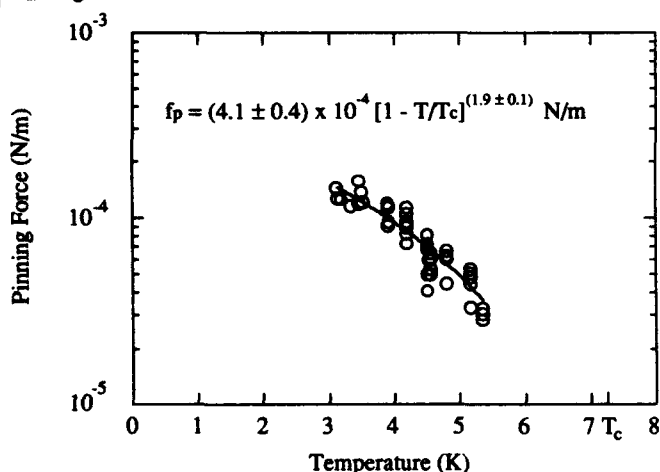
FIG. 3. Pinning force measurements with best fit by empirical model.
