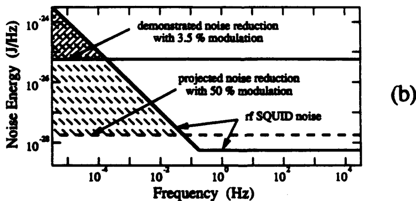
Fig 7 (a) Schematic of input circuit modulation. (b) Noise energy spectra from demonstration run with chip in Fig 6a.
