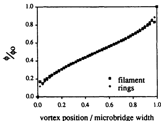
Figure 5. Fractional flux coupled to the SQUID due to the vortex. The two models are in good agreement except at the edges, where the large current gradient causes the discrete model to break down.
