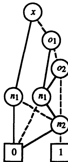
Figure 18: Symbolic representation of non-deterministic finite state machine. The number of variables grows logarithmically with the number of states.
