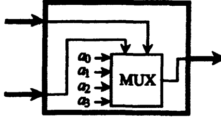
Figure 10: Universal function block. By assigning different values to the variables \vec{a} , an arbitrary 2-input operation can be realized.
