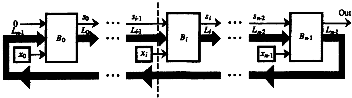
Figure 5: Linear Arrangement of Within- K Ring Circuit. As shown by the dashed line, the circuit has forward cross section 2 + \lceil \log_2 K \rceil and reverse cross section \lceil \log_2 K \rceil .
