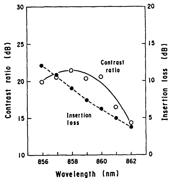
Fig.3. Contrast ratio and insertion loss as a function of bias wavelength for photonic gate arrays.
