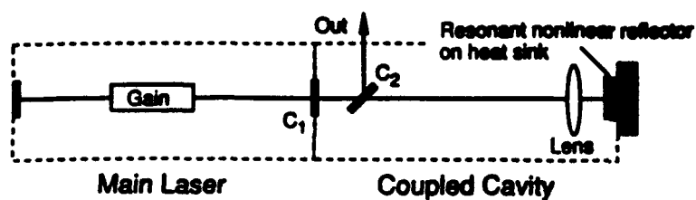
Fig. 1: RPM Laser
