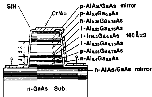
Fig.1 Device structure
