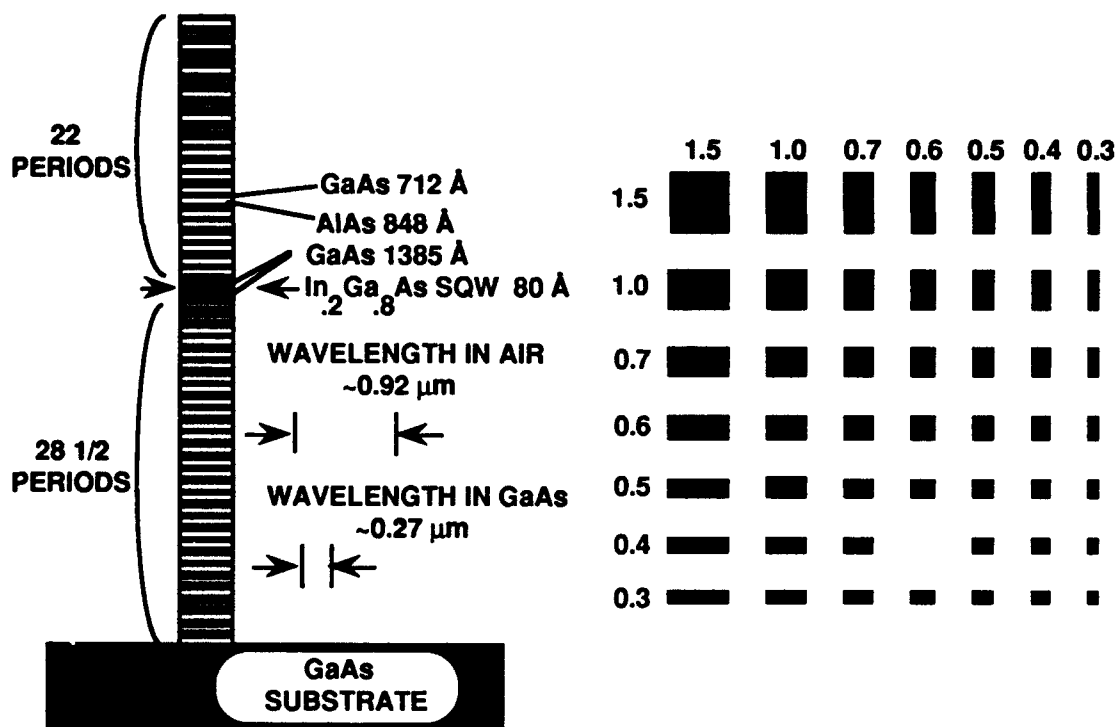
Fig. 1. Scale diagram of a 0.5 \mu\text{m} wide micro-resonator showing the MBE layer design.
