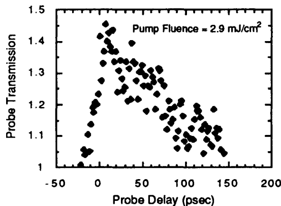
Fig. 3. Saturating absorption in multiple quantum wells. The transmission, at 820 \text{ nm} , recovers quickly as built-in fields sweep carriers from the wells.
