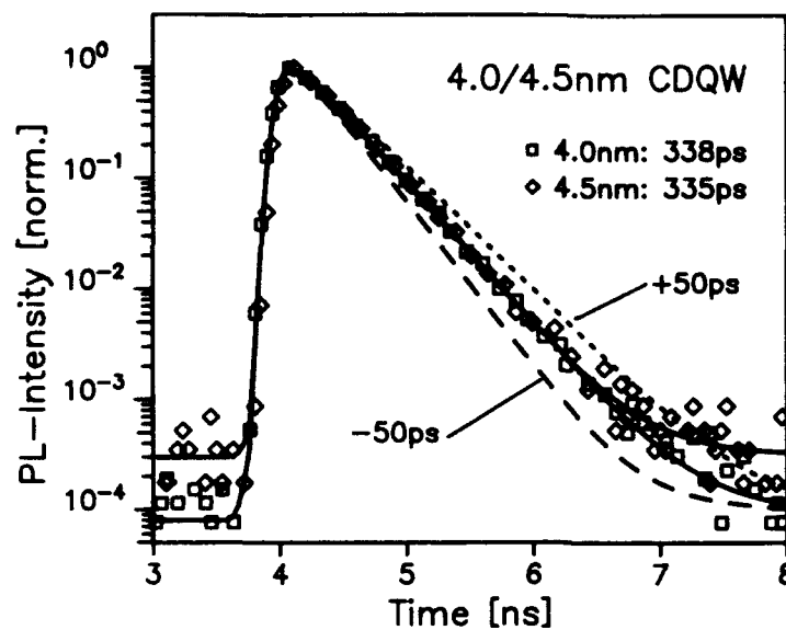
Fig. 4: Time resolved PL from the two components of the CDQW at an applied voltage of -2.0V . Squares: 40\text{\AA} -well, diamonds: 45\text{\AA} -well, solid lines: fits to the experimental data (almost undistinguishable in the figure). Also shown: calculated decay with \tau=388\text{ps} (dots) and \tau=288\text{ps} (dashed).
