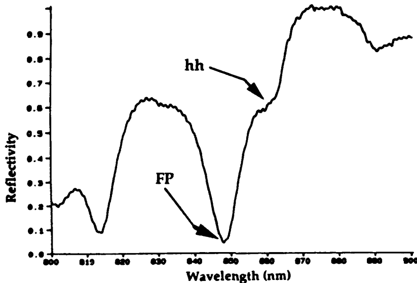
Figure 1 :- This shows a typical 0V reflection spectra for the original wafer. The heavy hole (hh) exciton is at 862nm while the Fabry-Perot resonance has clearly been misplaced to 848nm. Thus the hh is to the wrong side to permit modulation.
