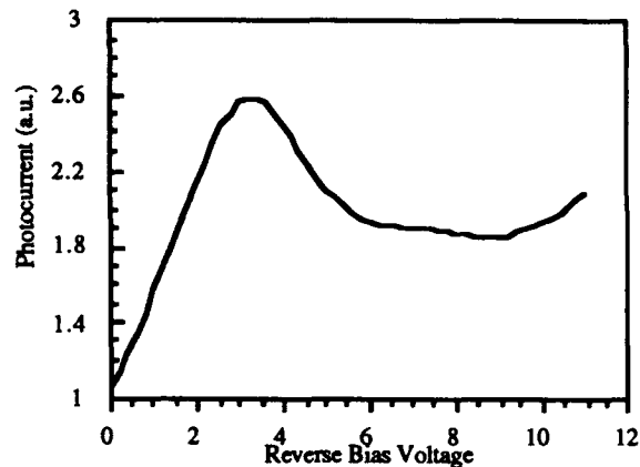
FIG. 4. Photocurrent resulting from the illumination of the modulator under 8264 Å light as a function of reverse bias voltage. The large negative photoconductivity causes bistability in SEED configurations.
