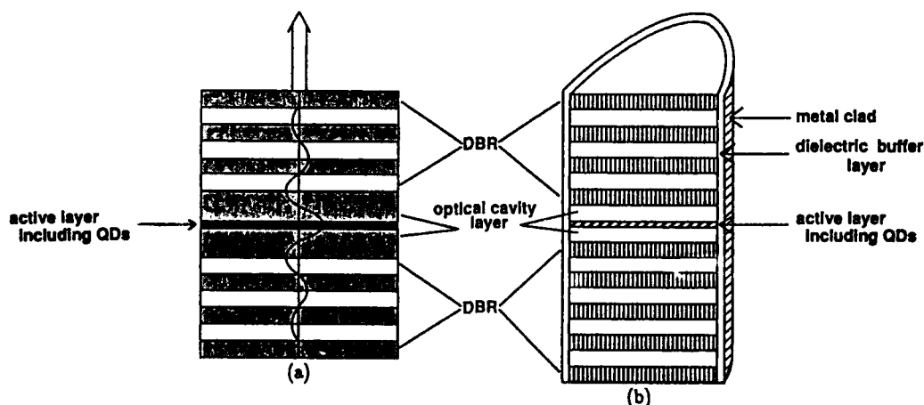
Fig.2 (a) A planar microcavity structure for modifying the radiation pattern. (b) A metal clad waveguide microcavity structure for modifying the radiation pattern.
