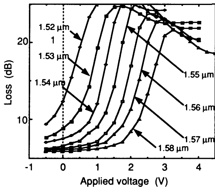
Fig.4 The modulation characteristics for several wavelengths.
