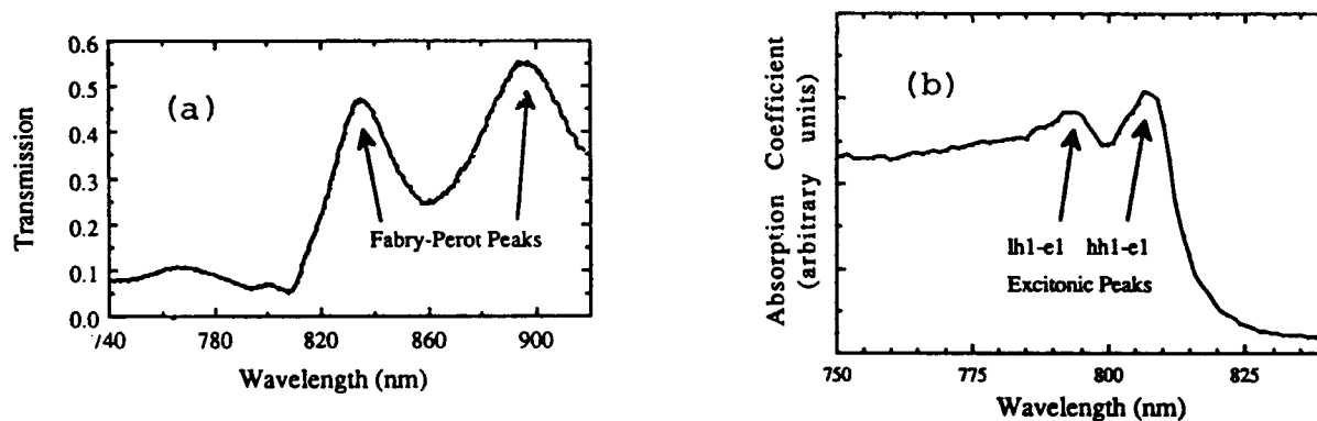
Fig. 2 (a) The transmission of the hetero n-i-p-i. Fabry-Perot oscillations due to multiple reflections from the sample surfaces are indicated. (b) The absorption coefficient deduced from (a). The n=1 heavy (hh1-e1) and light (lh1-e1) hole excitons of the weakly coupled wells are at the same wavelengths as for isolated 48 Å wells.
