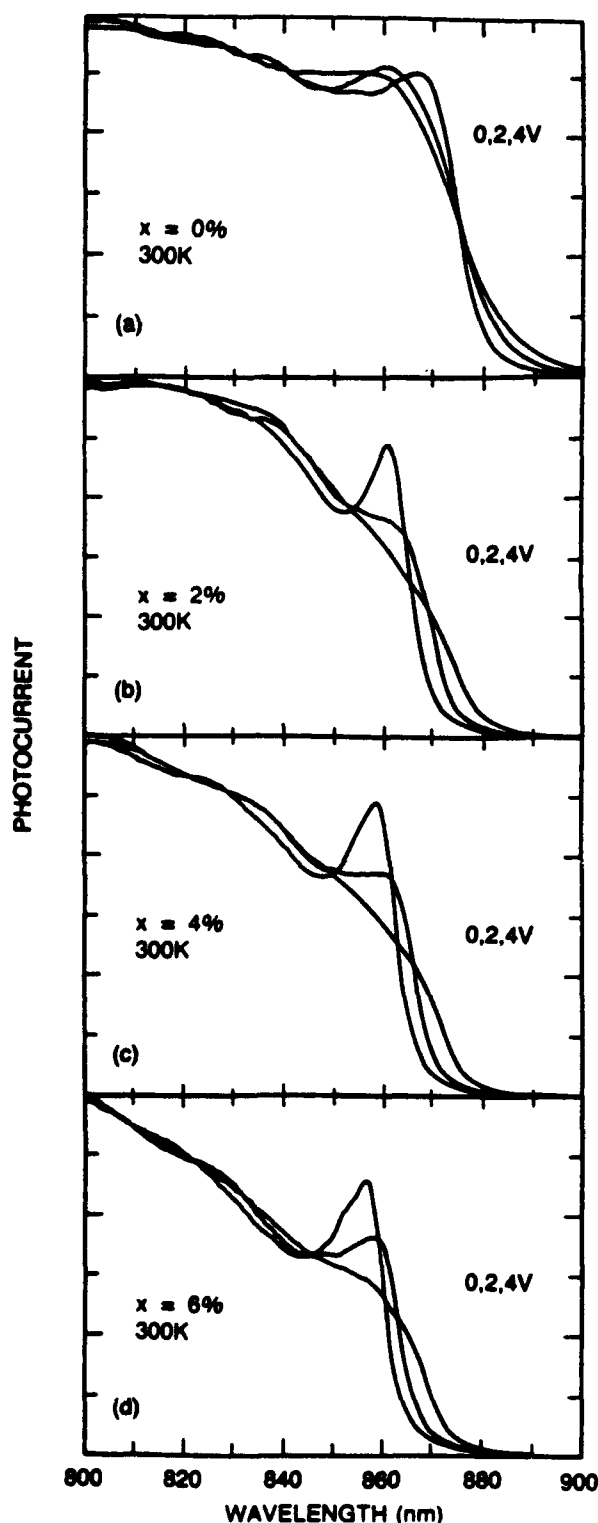
Fig. 1: Photocurrent measurements of samples with quantum well barrier height ranging from zero, showing that only an infinitesimal barrier is needed to retain an exciton at room temperature.
