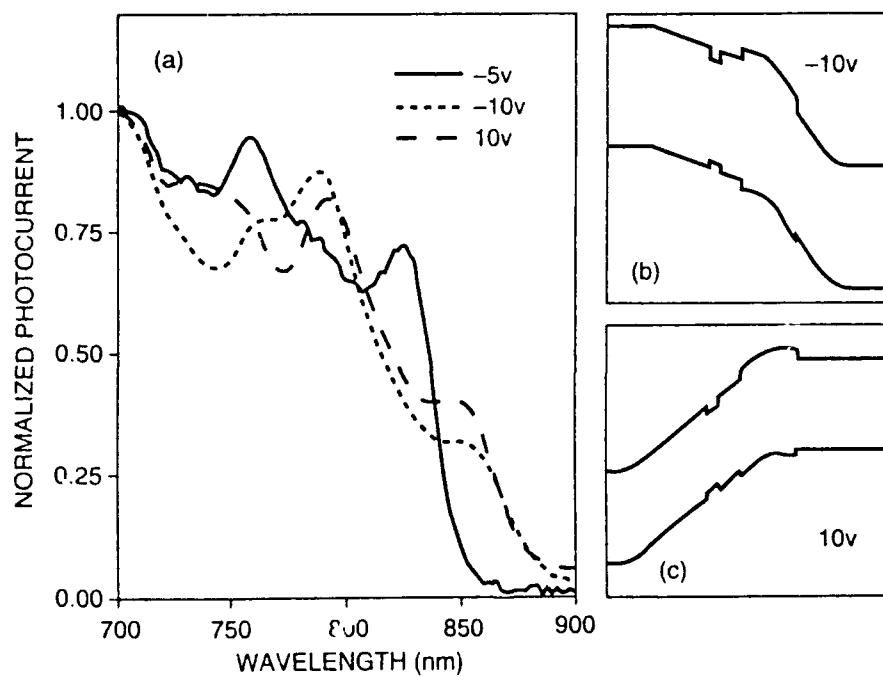
Fig. (3) (a) Normalized photocurrent spectrum for -V_{app} = -10V , -5V and 10V . Calculated energy band diagrams for (b) V_{app} = -10V , (c) for V_{app} = 10V .
