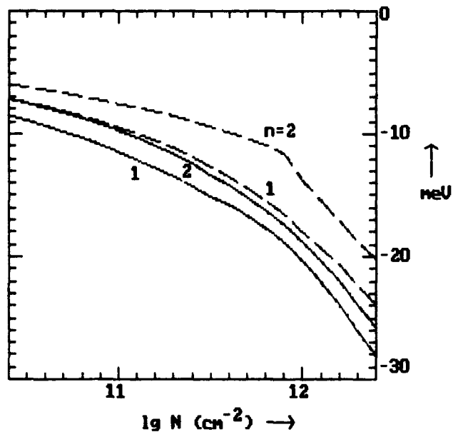
Fig.1 Calculated band gap renormalization of the first (e1-HH1) and second (e2-HH2) sublevel transition in an AlGaAs/GaAs single quantum well ( L_z = 20 nm, x = 0.30 ) at a temperature of 10K. Full curves - optical excitation, dashed - n-doping.
