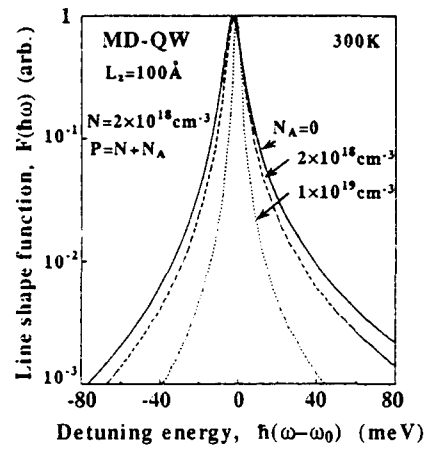
Fig. 3 Line shape functions of p-type modulation doped (MD) QW structures.
