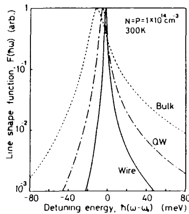
Fig. 5 Line shape functions at low carrier density.
