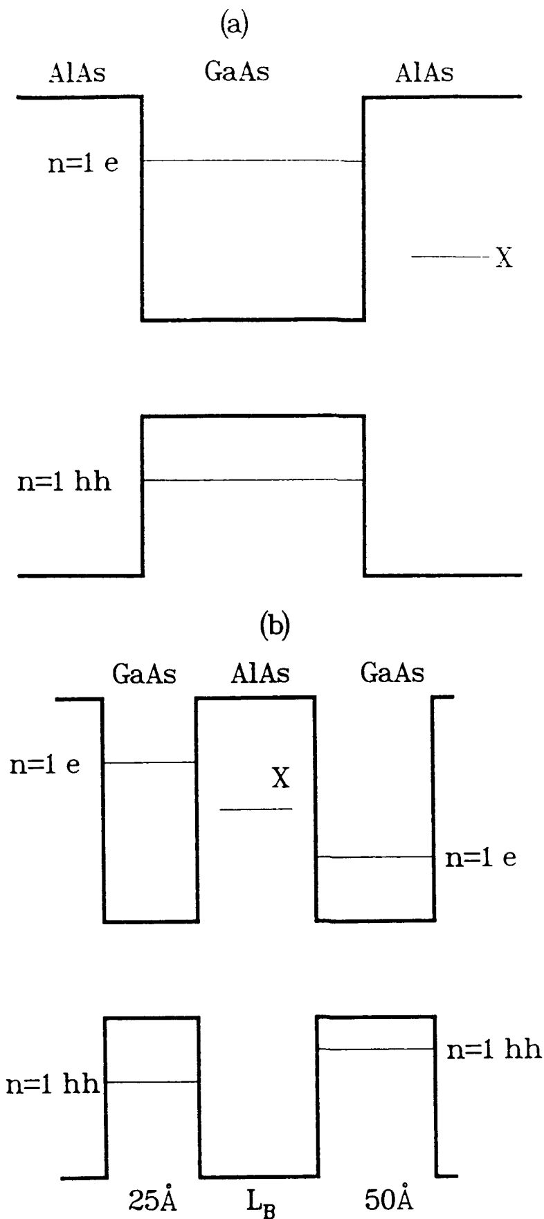
Figure 1: (a) conventional type II band alignment heterostructure (b) mixed type I/type II band structure
