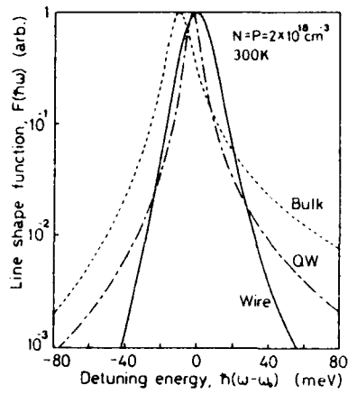
Fig. 2 Line shape functions at high carrier density.
