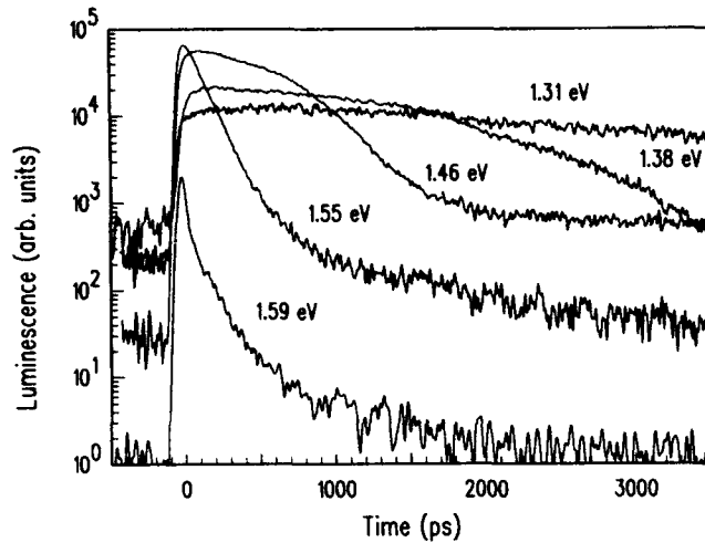
Fig. 2 - Luminescence of the \delta -doped superlattice photoexcited with 5 \times 10^{12} \text{ cm}^{-2} electron-hole pairs. Time dependence of above bandgap luminescence (1.59-1.55 eV) and sub bandedge luminescence (1.46-1.31 eV) on a short time scale.
