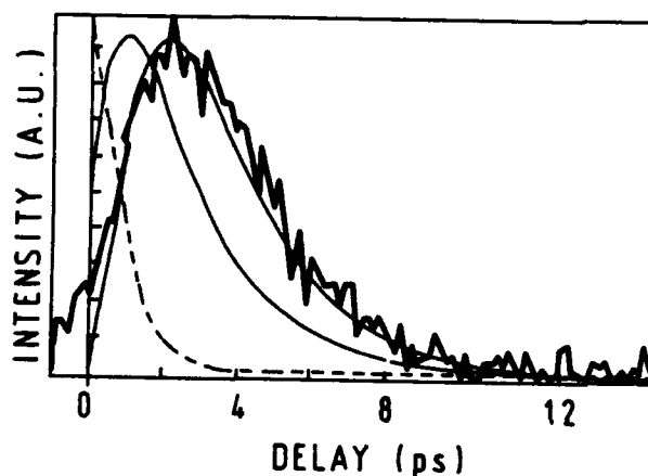
Fig.2: Decay time of the CL luminescence in a L-GRINSCH structure, together with different fits: (--) instantaneous capture by the well, (-.-) 1 ps capture time, (—) same with intervalley scattering.
