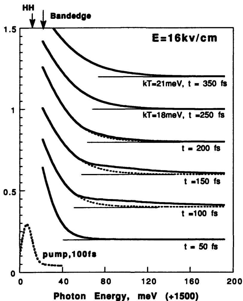
Fig.3 Distribution Functions extracted from the experiment by fitting
