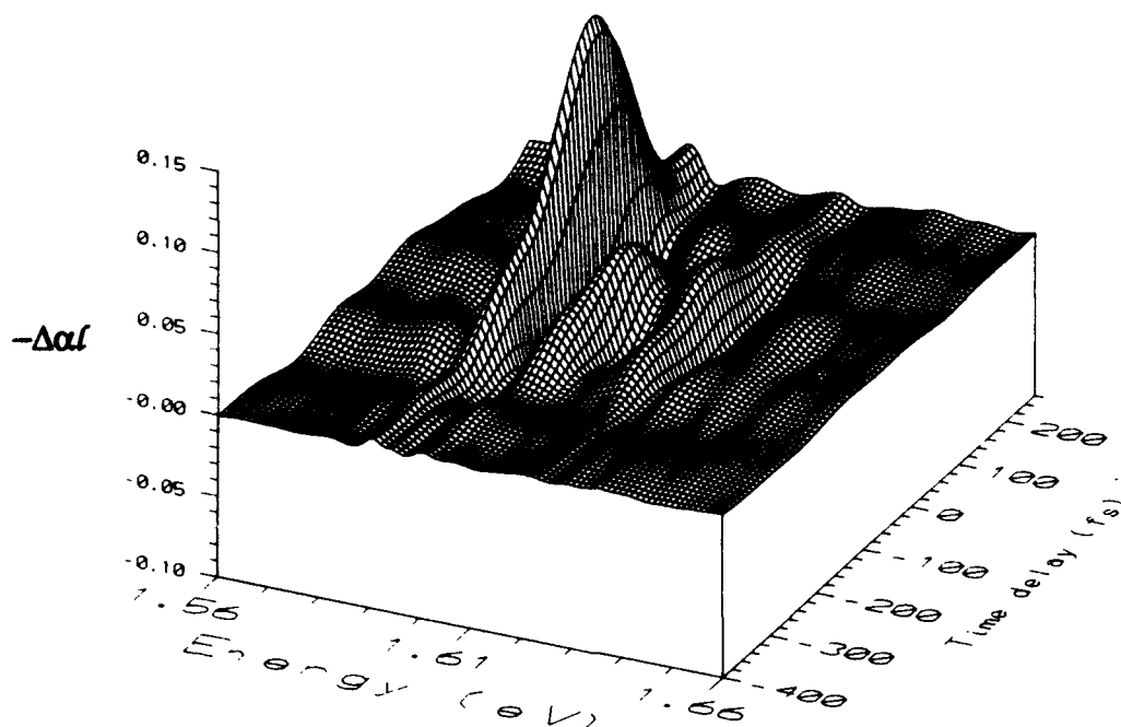
Figure 3 Differential transmission from the optical Stark effect of 12 T magneto-excitons. Energy shifts are seen at the 1shh, 1slh and 2shh resonances. Three points are interpolated between each pair of data points to make the surface profile clear.
