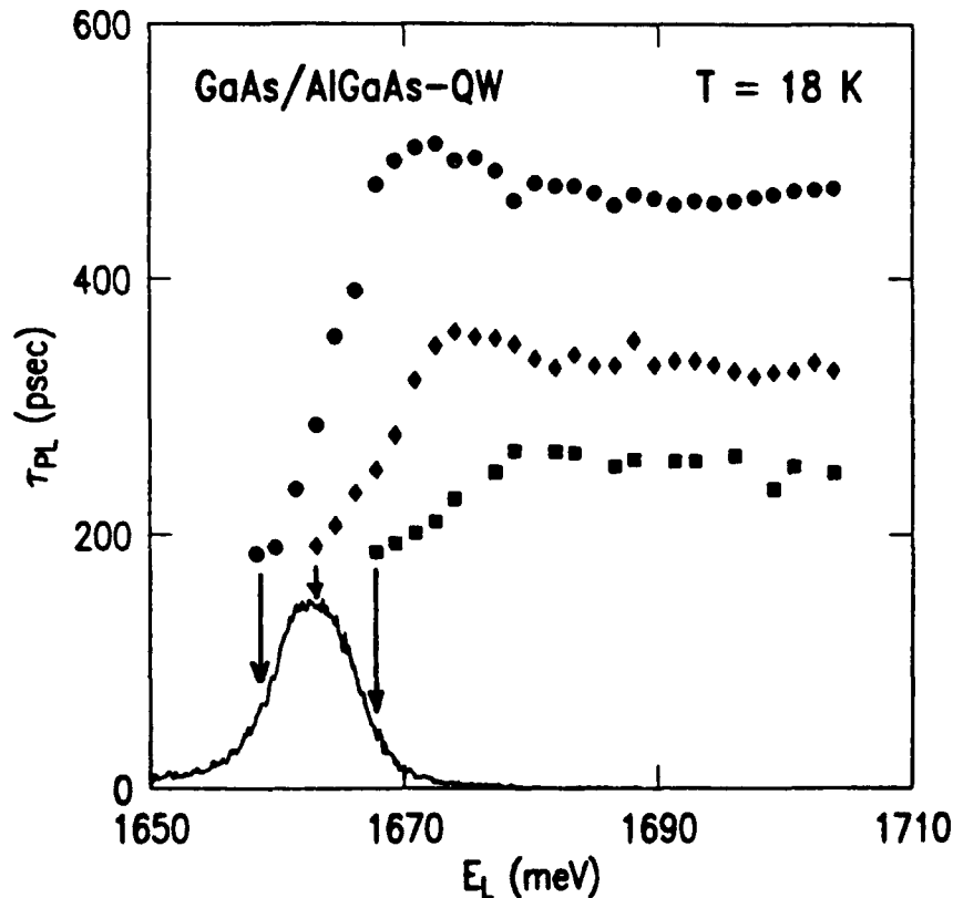
FIG. 2. Photoluminescence decay times vs. excitation energy for three different detection energies given by the arrows. The time-integrated photoluminescence spectrum is shown for comparison. The experimental conditions are the same as in FIG. 1.
