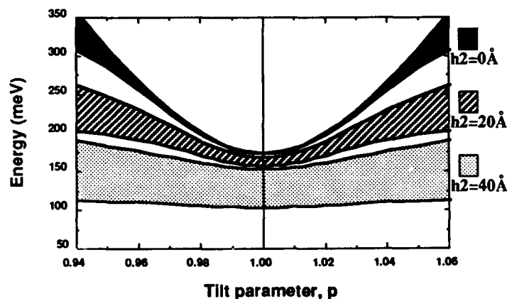
Fig.5. Miniband variation of the lowest conduction band subband vs tilt parameter p .
