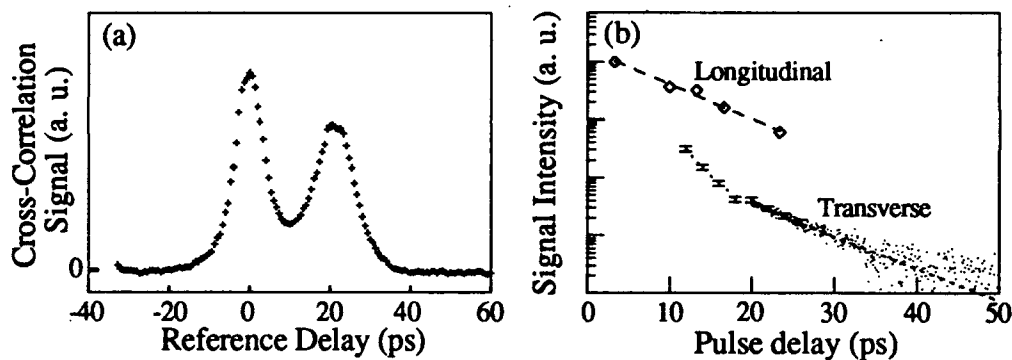
Figure 4. (a) Time resolved emission showing the presence of both a FPD signal (at delay time = 0) and a SPE signal (at delay time = 20 ps). (b). Measurement of \gamma_l and \gamma_t for the FPD emission.
