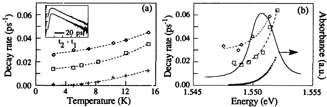
Figure 3. The TFWM response. \gamma_l (diamonds), \gamma_t (squares), and \gamma_{ph} (crosses) as function of temperature (a) and excitation energy (b). Inset: Upper curve is decay time integrated signal due to longitudinal relaxation as a function of \tau=t_3-t_2 . Lower curve is decay due to dephasing as a function of \tau=t_2-t_1 . The decay rate for \gamma_t(\gamma_l) is 4 (2) times the measured time-integrated decay of the signal.
