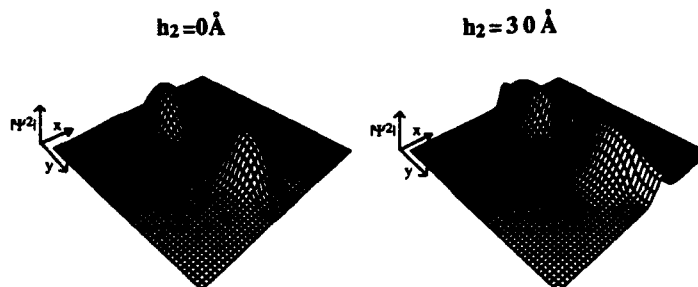
Fig.1.(c) Conduction band electronic wavefunctions for two different confinement levels.
