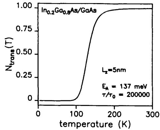
Fig.3 Part of the excitons emitted into the barrier versus T for a quantum well with x=0.2 and L_z=5\text{nm}
