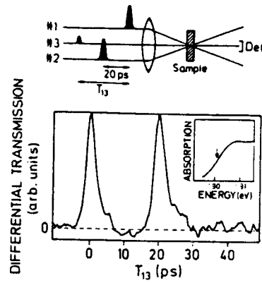
Fig.2 Pump and probe experiment of the type-II (Al 0.37 Ga 0.63 As) 68 (AlAs) 36 sample using two pump pulses separated by 20 ps.
