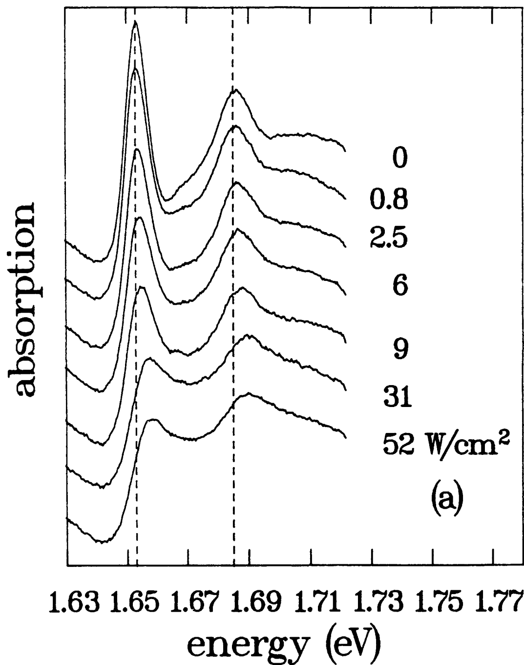
Figure 2: Nonlinear absorption spectra for the mixed type I/II samples having the 80Å barrier around the 50Å band edge. Annotated numbers indicate the cw power density
