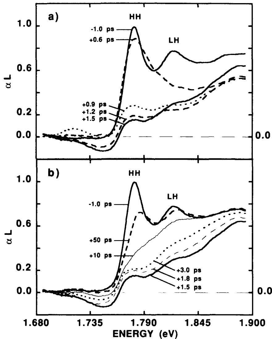
Figure 1. Time-dependent nonlinear absorption/gain spectra for pump/probe delays (a) \leq 1.5 ps and (b) > 1.5 ps ( E_{\text{exc}} = 1.96 eV, P_{\text{exc}} = 180 \mu\text{W} , pump diameter = 120 \mu\text{m} , f = 8.2 kHz, T = 15 K).
