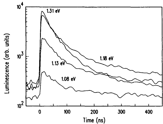
Fig. 3 - Time resolved luminescence for emission energies from 1.08 eV to 1.31 eV showing the slow nonexponential decay of the low energy transitions.
