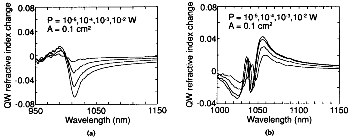
Fig.4. Spectral QW refractive index change calculated from fig.3. (a) Sample A, (b) Sample B.
