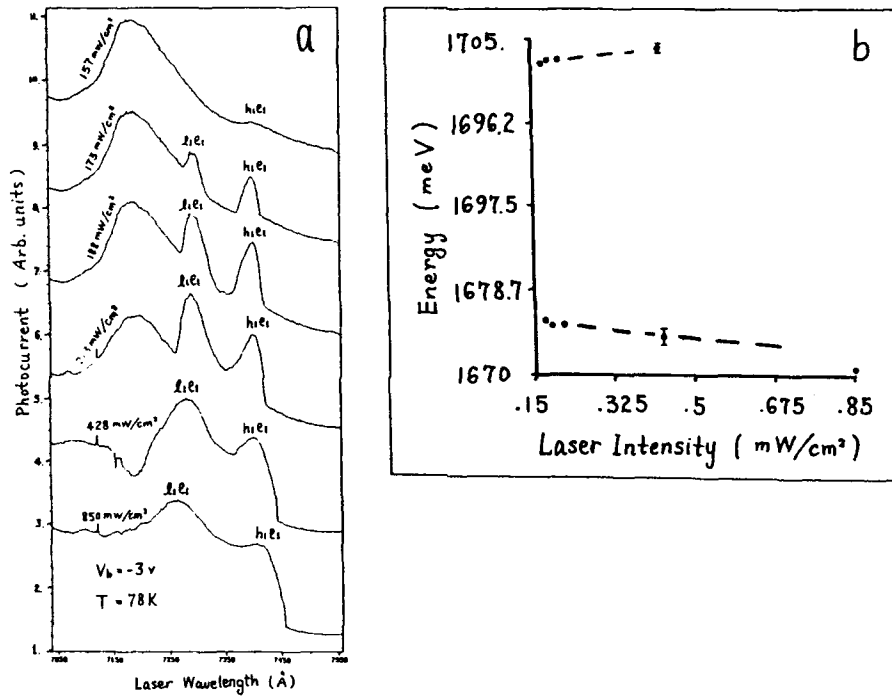
Fig. 3 (a) measurement of photocurrent spectra is shown at the constant reverse bias ( V_b \sim -3 \text{ V} ) for different laser intensities. (b) at V_b \sim -3 \text{ V} , the energies of heavy-hole and light-hole excitonic resonance transitions are plotted vs. laser intensity for dots: experimental data and broken lines: theoretical simulations.
