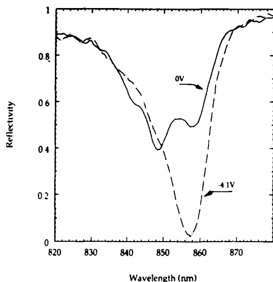
Figure 3. Reflectivity spectra for the unbiased (0V) and the maximum contrast case (4.1V reverse bias).
