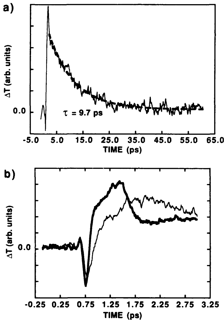
Figure 2. Single-wavelength time scans of the differential transmission \Delta T a) 65 ps scan at P = 180 \mu\text{W} , b) normalized 3.25 ps scan at P_{\text{exc}} = 110 \mu\text{W} (light solid) and P_{\text{exc}} = 180 \mu\text{W} (heavy solid). Detection energy = 1.746 eV, other experimental parameters same as in Fig. 1.
