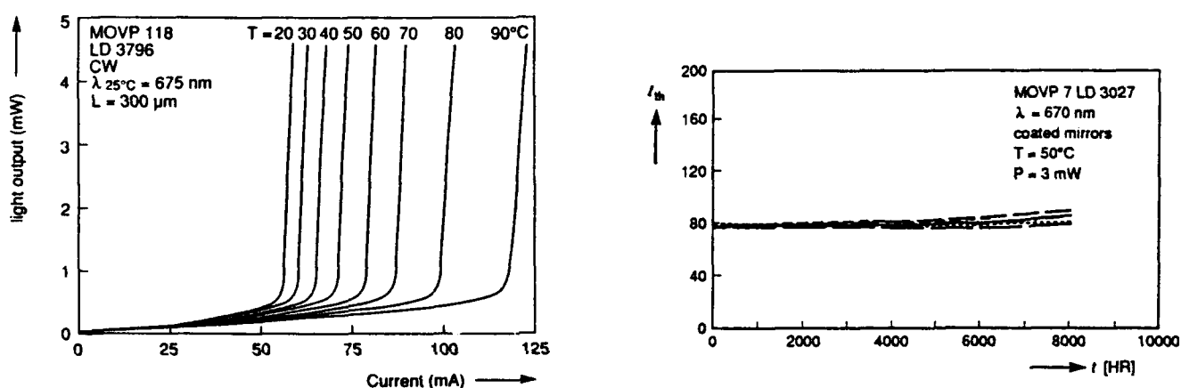
Fig. 1 Typical CW light-output vs current characteristics and APC lifetime performance of 670 nm visible lasers.
