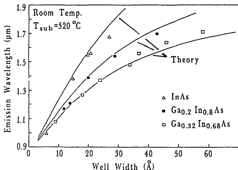
Fig. 2 Room temperature emission wavelength vs well width of strained QWs. Solid lines represent theoretical estimations (see ref.4).
