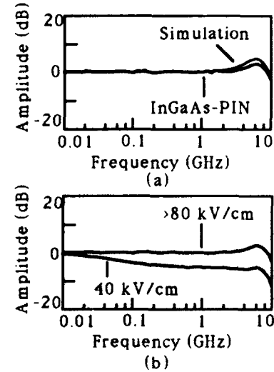
Fig. 3 Frequency responses of an InGaAs-PIN (a) and a hetero-PIN (b)
