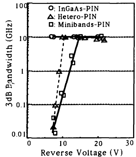
Fig.4 Bias dependence of frequency responses of the three PINs
