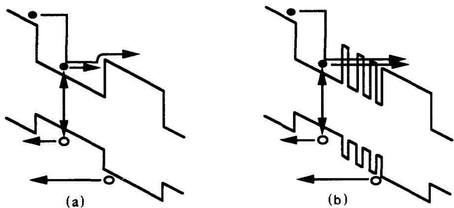
Fig.1 Energy diagrams of a conventional SL-APD (a) and a miniband SL-APD (b)
