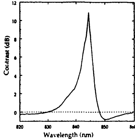
Figure 3 :- Displayed is the reflection contrast in dB of the normally-off device in Fig.2, for a voltage swing of 0V to -5V.
