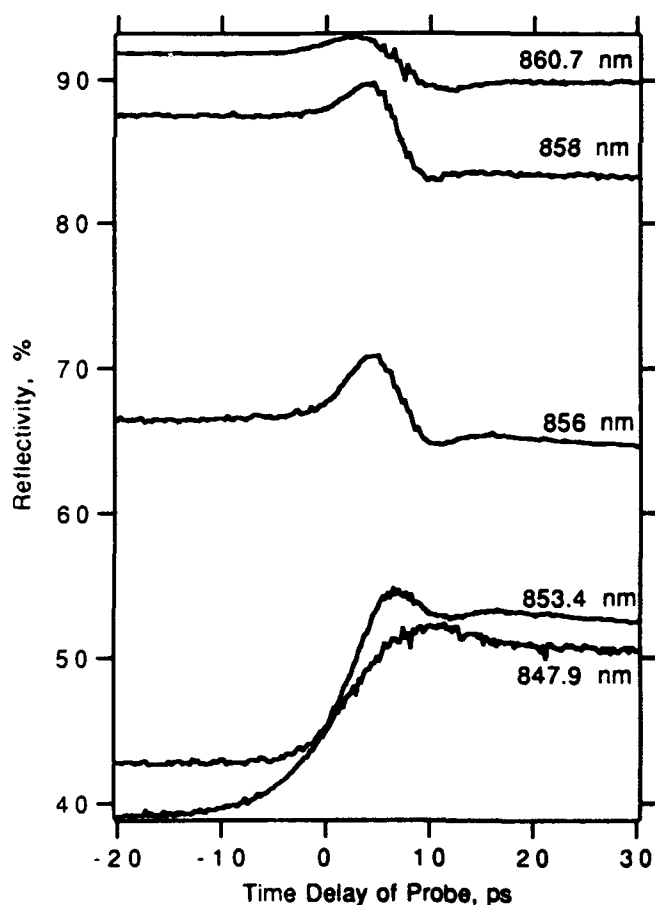
Fig. 3b: Pump-probe experiment on the GaAs/GaAlAs resonant reflector
