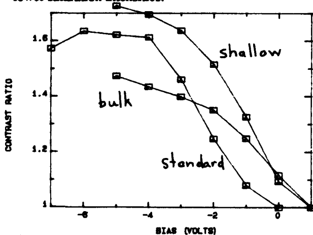
Fig. 4: Contrast ratio of bulk, shallow QW, and standard QW transmission modulators.
