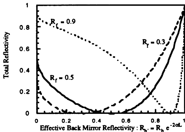
FIG. 1. Calculated total device reflectivity as a function of the effective cavity reflection for various front mirror reflectivities. Note: R_b = 1 corresponds to zero loss, while R_b = 0 corresponds to infinite absorption.
