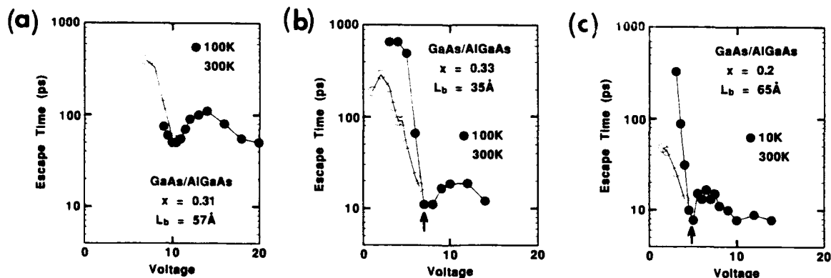
Figure 1 Measured sweep-out times for our GaAs/Al x Ga 1-x As p-i-n quantum well structures against reverse bias and temperature. The sample details are as follows: (a) 75 periods with L_w=65\text{\AA} , L_b=57\text{\AA} , x=0.31 ; (b) 80 periods with L_w=95\text{\AA} , L_b=35\text{\AA} , x=0.33 ; (c) 65 periods with L_w=95\text{\AA} , L_b=65\text{\AA} , x=0.20 . The arrows in (b) and (c) indicate the resonant tunneling voltage determined from photocurrent spectroscopy.
