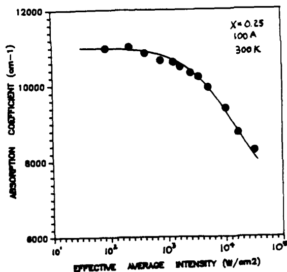
Fig. 4. Room temperature absorption coefficient as a function of optical intensity for sample with x=0.25 , Lw=100\text{\AA} . Filled circles are experimental data. Solid line is a fit with excitonic saturation intensity I_{SAT}=15\text{ kW/cm}^2 : \alpha(I) = \alpha_0 + \alpha_1 / (1 + I/I_{SAT})
