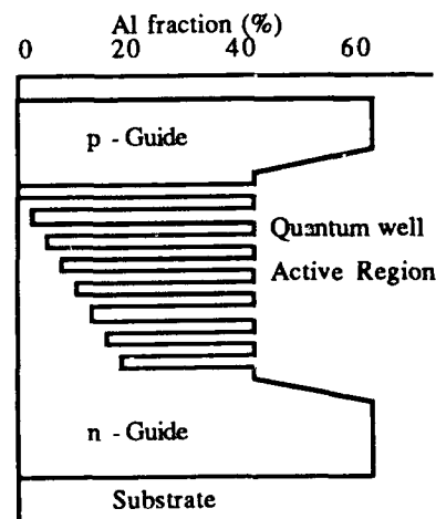
Figure 1. Typical layer structure for a broad band surface emitting LED.
