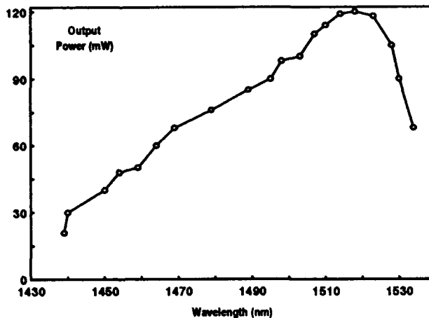
Figure 4: EX-SEL peak lasing power as a function of wavelength. Operating temperature is fixed at 77 K.
