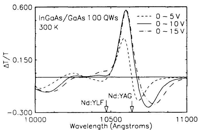
FIG. 1. \text{In}_x\text{Ga}_{1-x}\text{As} / \text{GaAs} absorption spectra and \Delta T/T data at 300 K.
