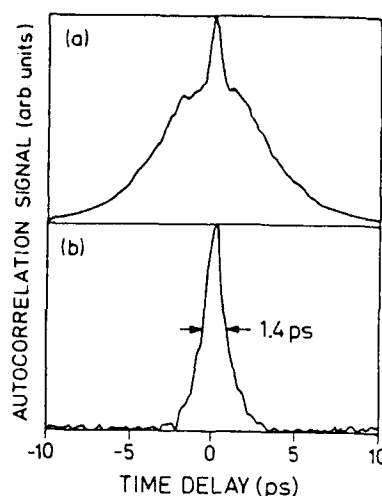
Fig.4 Intensity autocorrelation traces of the dye-laser output without (a) and with (b) the type-II absorber installed.
