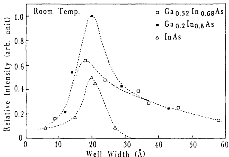
Fig. 4 Room temperature relative PL intensity vs well width of strained QWs. Intensity increased from well width of 60Å to 20Å, but decreased rapidly after 20Å. It was probably due to layer fluctuations.
