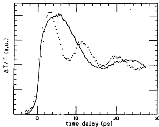
Fig. 2: Pump-probe signal at 2T (solid) and 4T (dotted).
