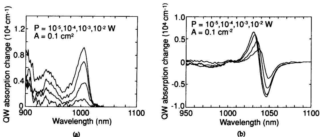
Fig.3. Spectral QW absorption change calculated from the results in fig.2. (a) Sample A, (b) Sample B.
