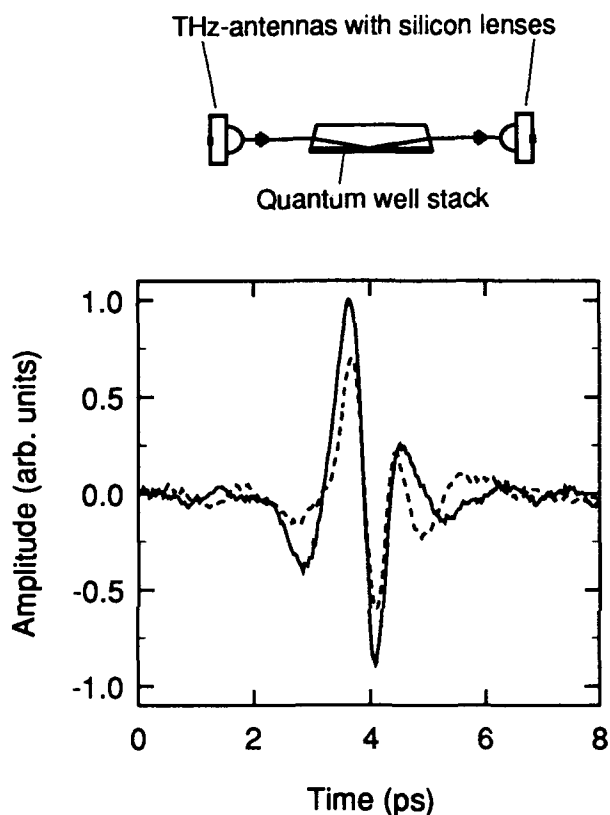
FIG. 1: Time dependence of the detected amplitude of the far-infrared light pulse after propagation through the sample. Sample temperatures: 300\text{ K} (solid line) and 7\text{ K} (dashed line). The experimental setup is shown schematically in the upper part of the figure.
