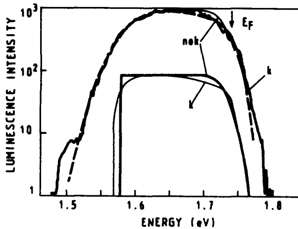
Fig.3: Luminescence spectrum of a 4.2 \times 10^{12} \text{ cm}^{-2} plasma. Fits assuming or not conservation of the k selection rule are shown. The corresponding unbroadened spectra are displaced by one decade.
