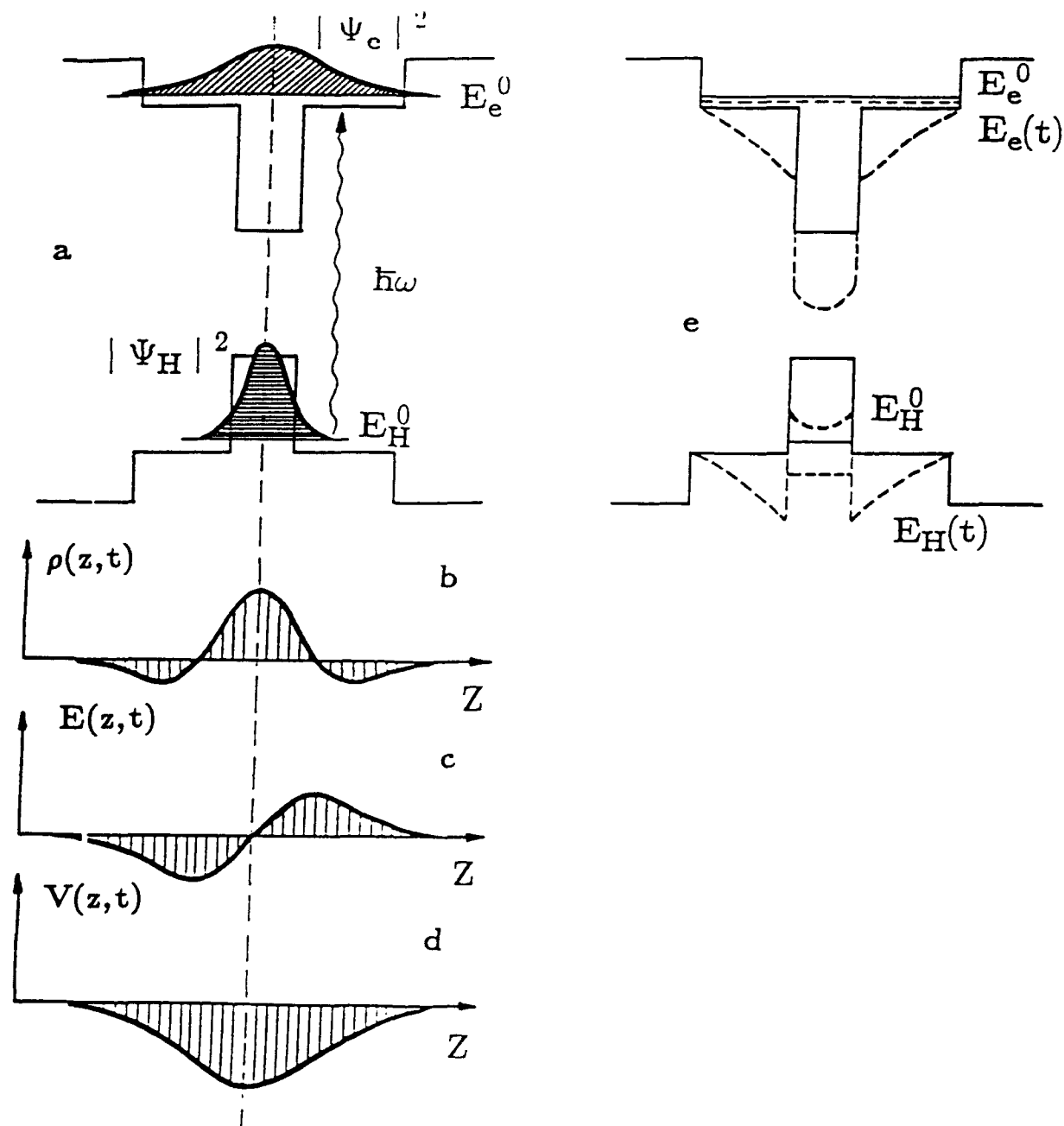
Fig.1. Coulomb-assisted energy level pulsations of excitonic transition in stepped quantum well.
