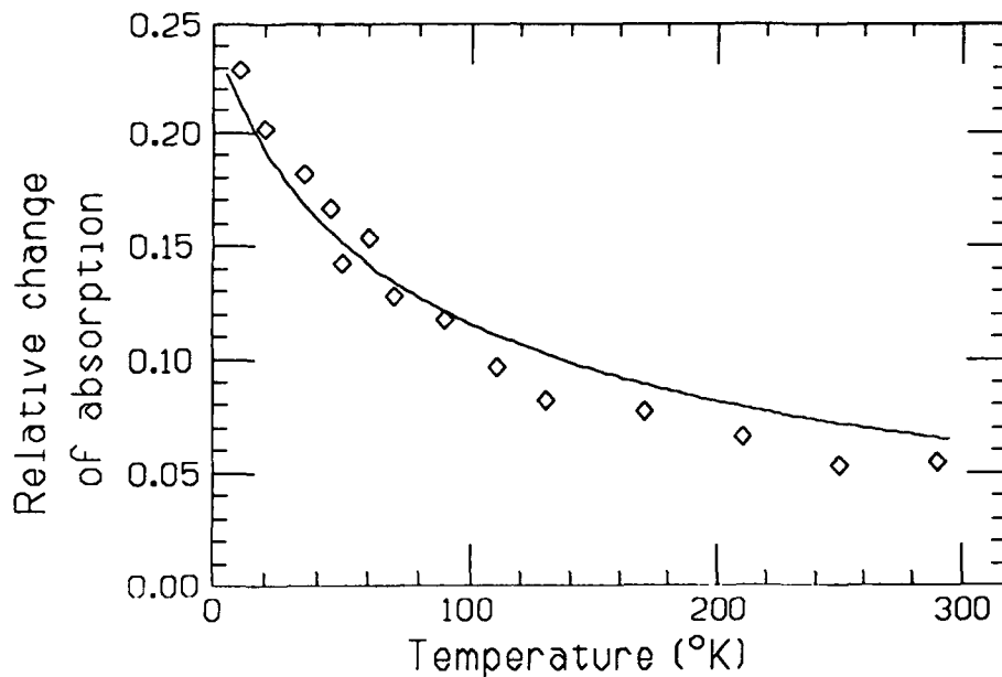
Fig. 2. The relative change of the heavy hole exciton area as a function of temperature. The solid line is the calculated N/N_s^e(T) for N = 2.5 \times 10^{10} \text{ cm}^{-2} .
