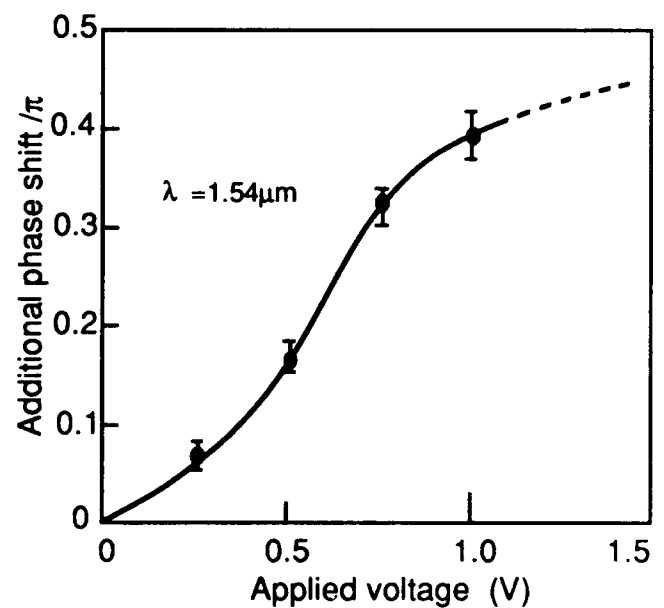
Fig.5 Phase modulation characteristics of the modulator.
