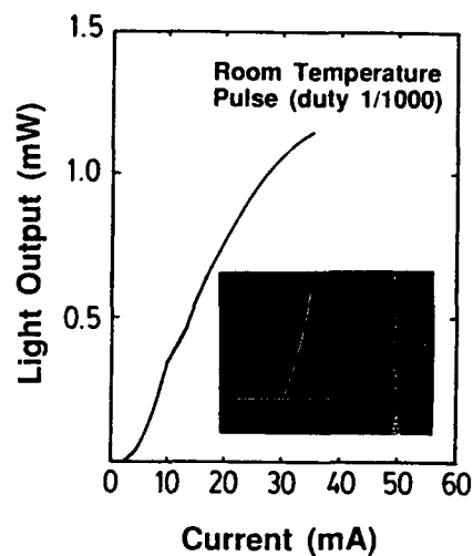
Fig.2 Current-light output/ current-voltage(inset) characteristics
