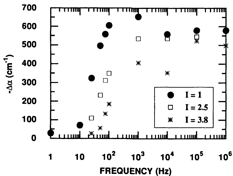
Figure 3. Electroabsorption due to the quantum confined stark effect at \lambda = 604 nm as a function of frequency of the applied ac field for several incident light intensities.
