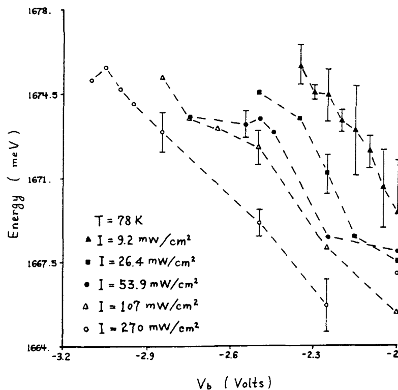
Fig. 2 The energy in the photo-current spectra at which the heavy holes in two coupled wells undergo resonance vs. reverse bias for different laser intensities.
