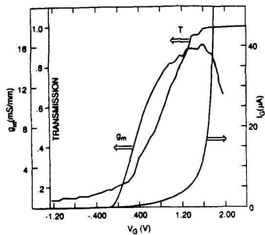
Figure 4 Transmission, transconductance, and gate leakage as a function of gate voltage.
