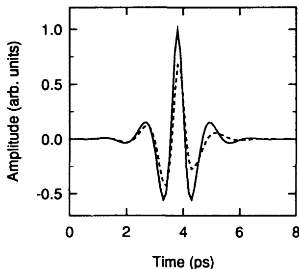
Fig. 3: Calculated temporal shape of a detected far-infrared pulse without (solid line) and with (dashed line) absorption.
