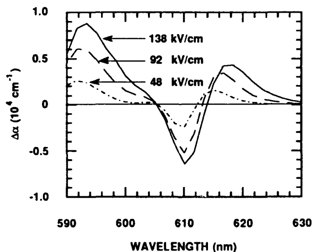
Figure 1. Change in the absorption coefficient due to the quantum confined stark effect in II-VI multiple quantum wells for several different applied fields.
