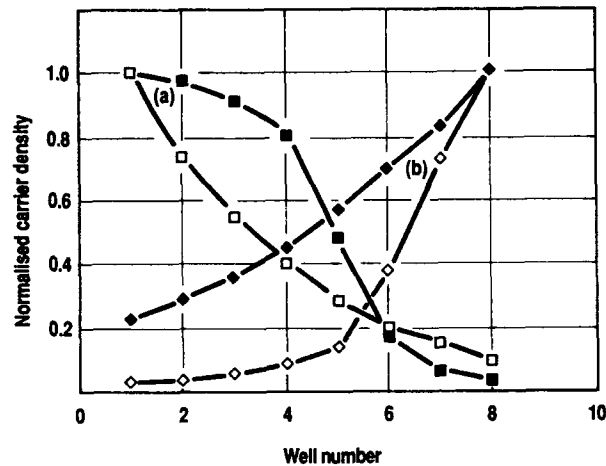
Figure 2. Modelled carrier distribution across a series of 100Å wells, a-electrons, b-holes. Solid points - high injection, open points - low injection.
