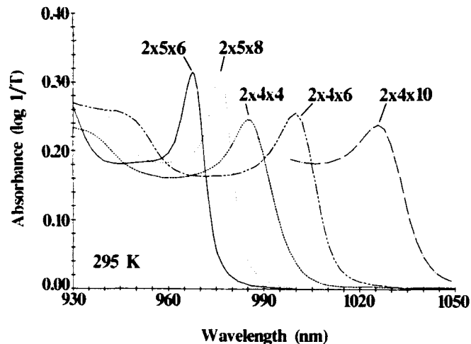
Fig.1 Room temperature absorbance of the InAs/GaAs superlattice MQW samples.
