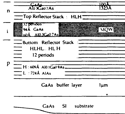
Figure 2. The epitaxial structure of the AFPM device.
