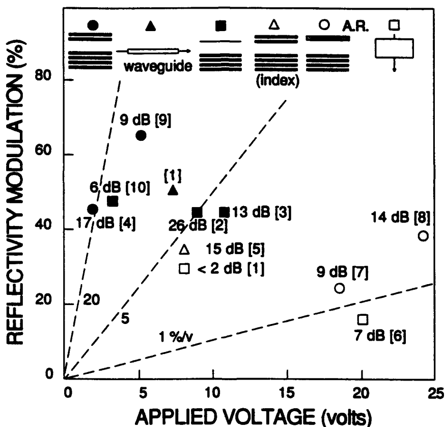
Figure 1 A performance comparison of various surface-normal optical modulators. The dash lines represent different normalized transfer functions of 1, 5 and 20 %/V. The numbers are the contrast ratios [references].
