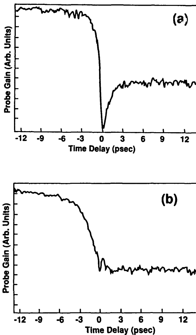
Fig. {2} Gain dynamics obtained from time resolved pump probe measurements for (a) input pulse widths of 560 fsec, and (b) input pulse widths of 2 psec.
