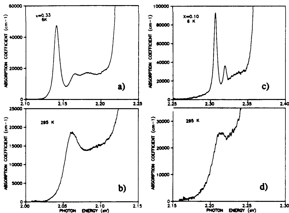
Fig. 2 Absorption spectrum of sample A (C) showing well-resolved n=1 hh excitonic feature at a)(c) 6K and b)(d) 295K. Absorption coefficients refer to the total thickness of CdZnTe wells plus ZnTe barriers.
