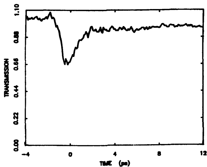
Figure 3: Gain recovery of the CSBH amplifier, measured at 1.52 \mu\text{m} and 40 mA bias. The data here is presented as time-resolved transmission.
