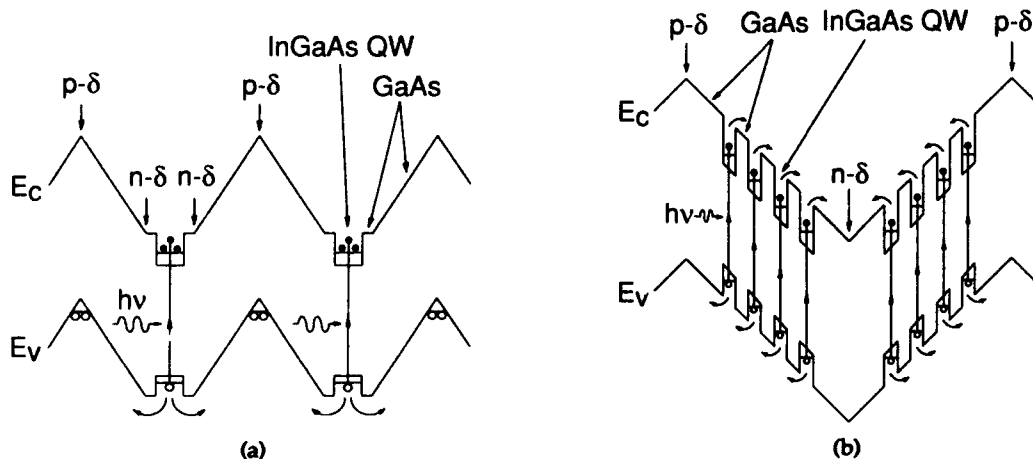
Fig.1. Energy band diagrams of (a) sample A and (b) sample B.
