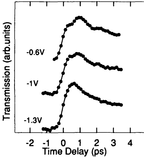
Figure 3: Transmission versus delay time for different bias fields.
