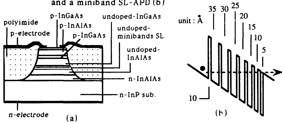
Fig.2 Cross-section of a miniband-PIN (a) and energy diagram of the fabricated minibands (b)
