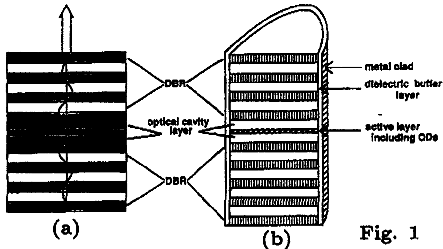
Fig. 1 (a) A planar microcavity structure for modifying the radiation pattern. (b) A metal clad waveguide microcavity structure for modifying the radiation pattern.
