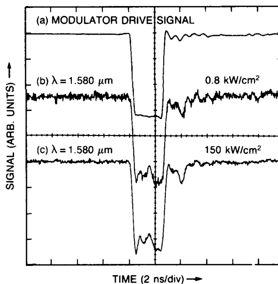
Figure 2: Sampling oscilloscope traces. Trace (a) shows the electrical pulse applied to the modulator, while traces (b) and (c) show the generated optical response at low and high optical intensities. Note that fast response is seen at both low and high intensity.
