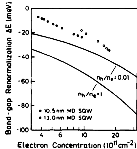
Fig. 4. Band-gap renormalization ( \Delta E ) as a function of the 2D electron concentration. The "•" and "o" represent the data of sample a with 10.5 nm well width and of b with 13.0 nm well width, respectively. The n_h/n_e represent the ratio of concentrations of holes and electrons used in the calculation.
