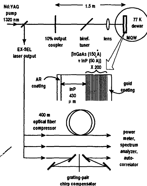
Figure 1: External-cavity surface emitting semiconductor laser (EX-SEL). A 1.5 m cavity is formed by a 10% output coupler and a gold-coated InGaAs/InP MQW at 77 K.
