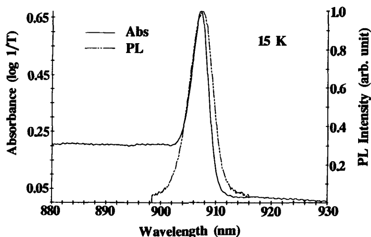
Fig.3 Excitonic absorbance and photoluminescence at 15 K for 2x5x6 sample.
