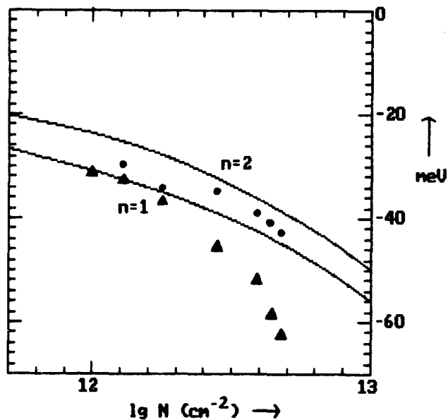
Fig.2 Density dependence of the BGR for the first (e1-HH1, triangles) and second (e2-HH2, dots) sublevel transition. Full curves - dynamical self-energy calculation, symbols - experimental data from [9] ( L_z = 10.3 nm, x = 0.37 , T = 300 K).
