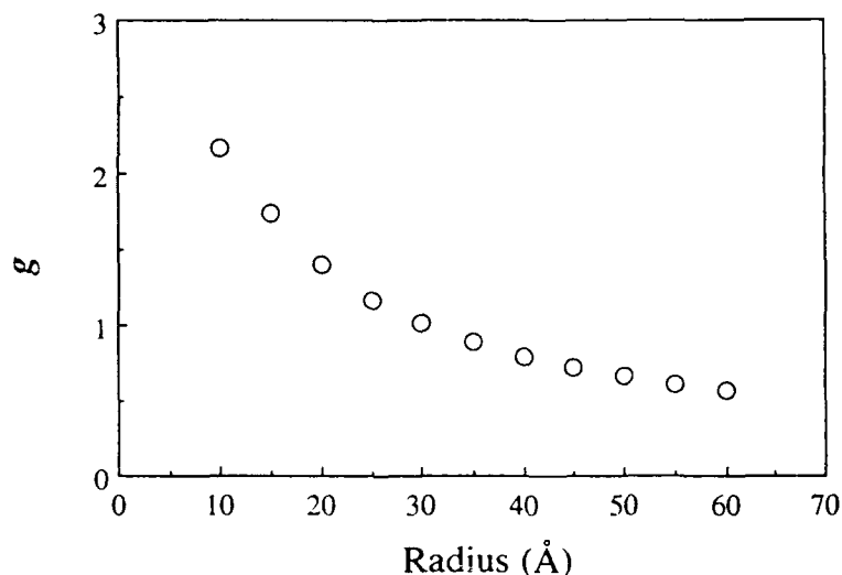
FIG. 3 The calculated size dependence of the Huang-Rhys parameter, g .
