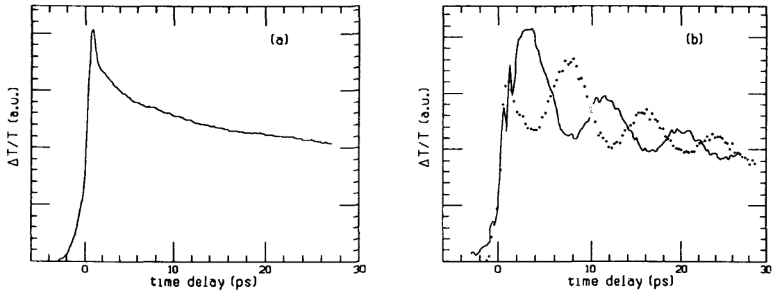
Fig. 1: Absorption change of the hh exciton for (a) B=0 and (b) B=4T . The solid line curves were measured at orthogonal pump-probe polarizations, and the dotted at parallel polarizations.
