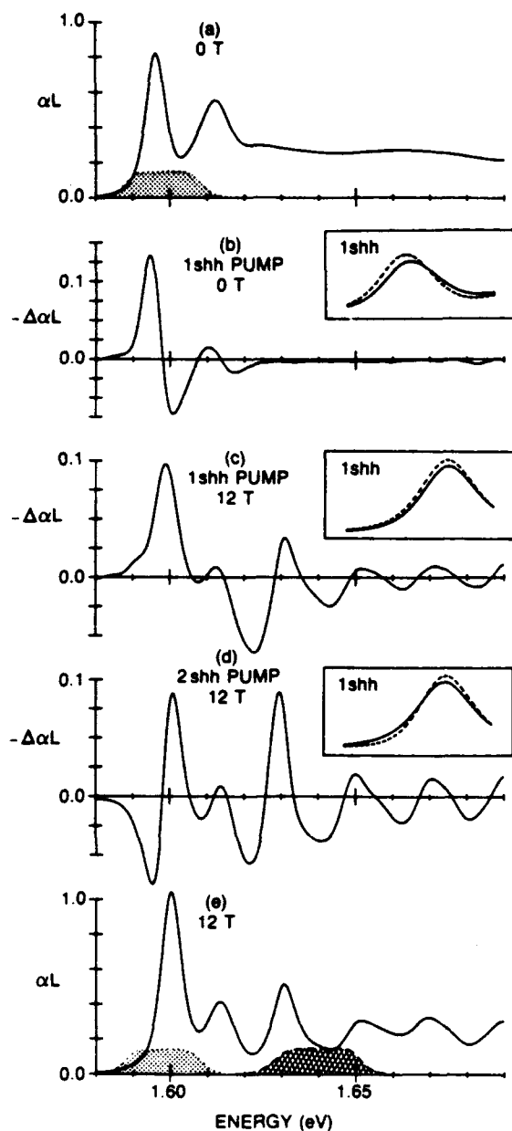
Figure 2 Linear absorption at 0 T (a) and 12 T (e). Dotted and hatched areas indicate the pump spectra for 1s and 2s hh exciton pumping, respectively. Differential transmission for 1s hh exciton pumping at 0 T (b) and 12 T (c), and for 2s hh exciton pumping at 12 T (d), all for probe 600 fs after pump. Insets show the corresponding 1s hh exciton absorption 600 fs before (dashed) and 600 fs after (solid) the arrival of the pump.
