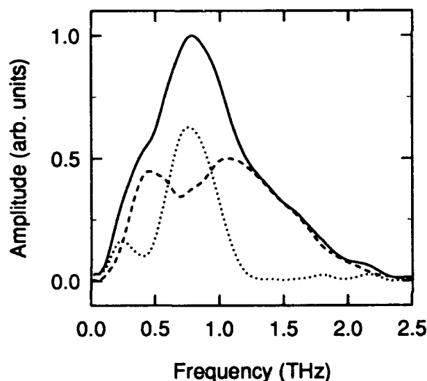
Fig. 2: Fourier spectra of the far-infrared pulses of Fig. 1 for sample temperatures of 300 K (solid line) and 7 K (dashed line). The dotted line shows the difference between the two spectra.
