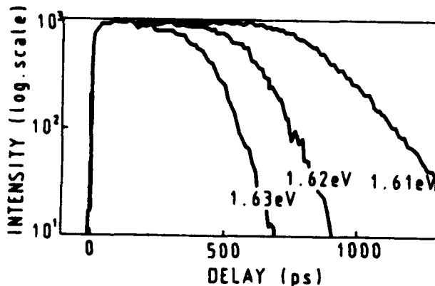
Fig.4: Decay curves of the QW luminescence at different energies above the band edge. The constancy of the signal is a direct demonstration of k -selection rule.
