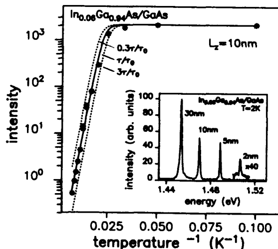
Fig.1 PL intensity versus T ( x=0.06 ; L_z=10\text{nm} ) Fits are drawn in as described in the text. The inset show the low temperature ( T=2\text{K} ) spectrum of a sample with x=0.06
