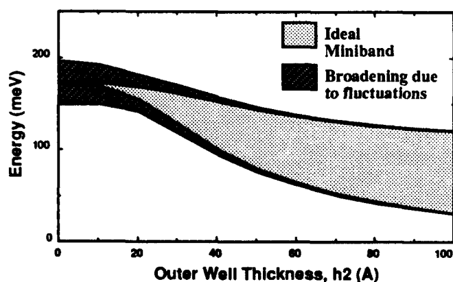
Fig.4. Miniband broadening of the lowest conduction band subband due to random wire width variations with an average of 3\text{\AA} .
