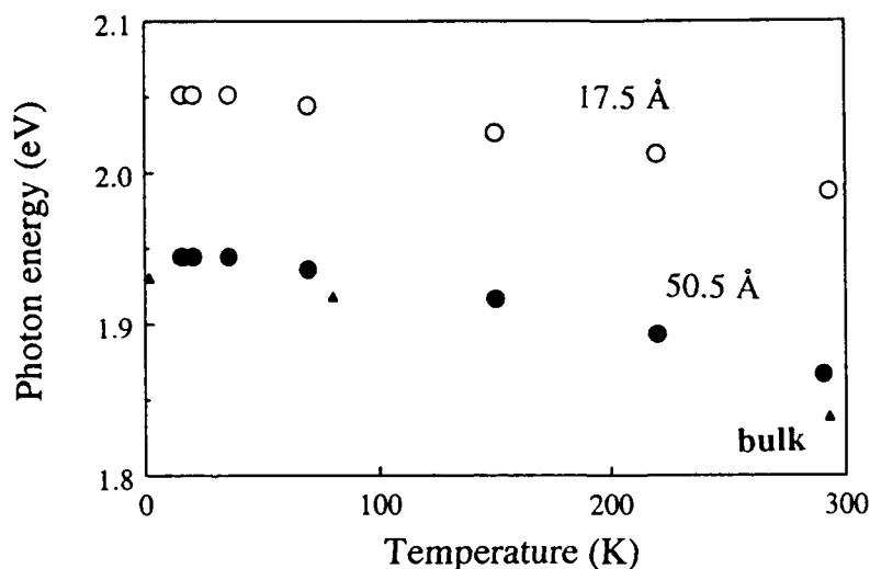
FIG. 1 The temperature dependence of the exciton energy of microcrystallites of radius of 17.5 Å (open circles) and 50.5 Å (closed circles), respectively. The bulk band gap is also depicted 5 (triangles).
