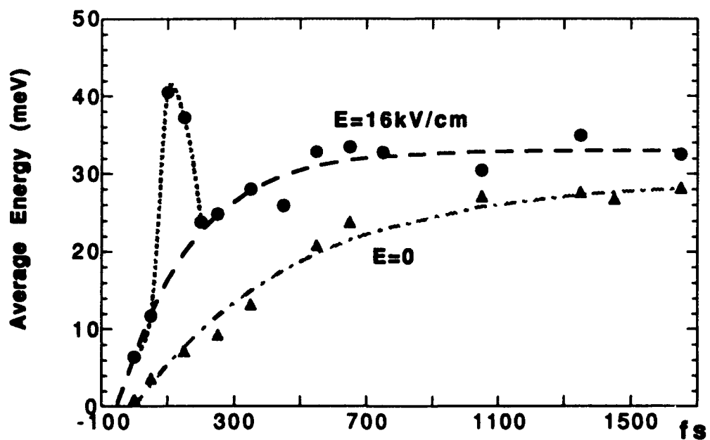
Fig.4 Average energy vs. delay time after the excitation
