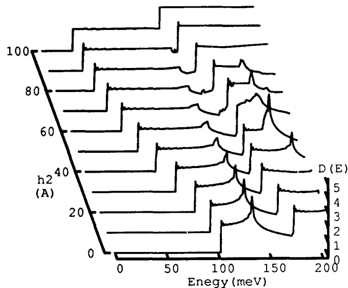
Fig.2. Conduction band density of states ( 10^9/\text{eV}\cdot\text{cm} ) of a TSL with x_b=0.25 , x_c=0.25 , W=S=40\text{\AA} , h_1=100\text{\AA} .
