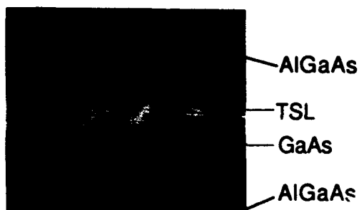
Fig.1.(a) Cross sectional TEM profile of a TSL.
