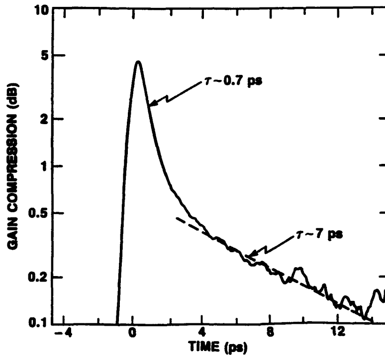
Figure 1: Gain recovery of the MQW amplifier, measured at 1.47 \mu\text{m} with 150 mA bias.
