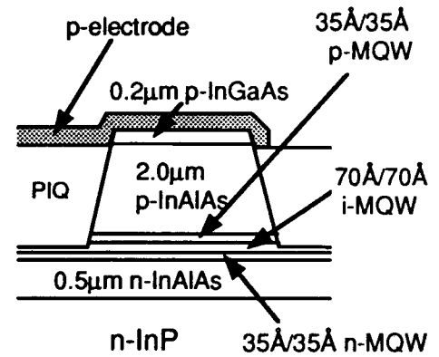
Fig.3 The cross section of the modulator with SP MQWs.
