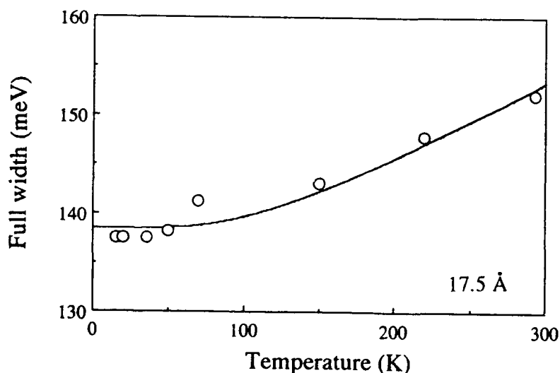
FIG. 2 The temperature dependence of the width of the exciton in 17.5 Å microcrystallites. The solid curve is the best fitted curve.
