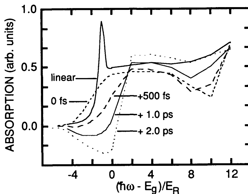
Figure 3. Calculated carrier-density-dependent absorption spectra computed for bulk GaAs at various pump probe delays. (injected density 2 \times 10^{18} \text{ cm}^{-3} , T = 15 \text{ K} ).
