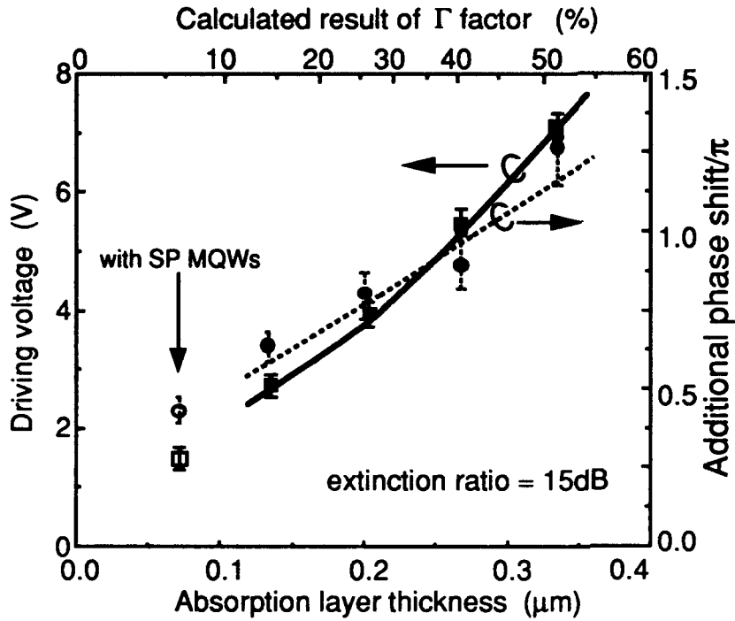
Fig.2 The driving voltage and the additional phase shift as a function of absorption layer thickness.
