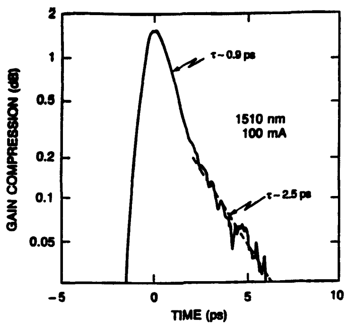
Figure 2: Gain recovery of the SLMQW amplifier, measured at 1.51 \mu\text{m} and 100 mA bias.
