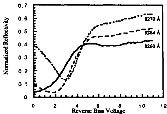
FIG. 3. Measured normalized reflectivity as a function of reverse bias voltage at 3 different wavelengths.
