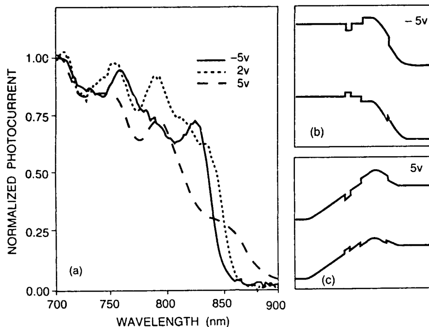
Fig. (2) (a) Photocurrent spectra for -V_{app} = -5V , 2V and 5V , normalized to the value at short wavelength. Calculated energy band diagrams for (b) V_{app} = -5V , (c) V_{app} = 5V .
