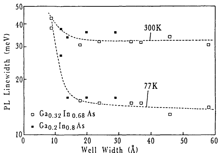
Fig. 3 PL linewidth vs well width of strained QWs at 300K and 77K. At 77K, around 15meV of linewidths were obtained for well widths of above 20Å and less than 60Å. For well width less than 20Å, linewidth increased due probably to layer fluctuations.
