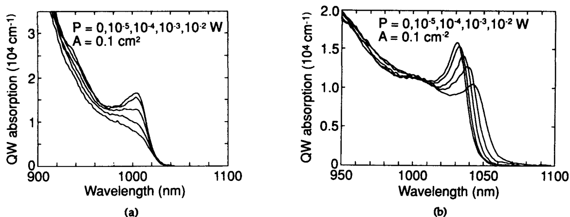
Fig.2. Optical QW absorption spectra of (a) sample A and (b) sample B recorded with various excitation intensities.
