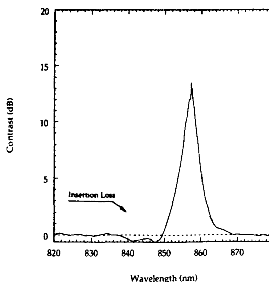
Figure 4. Contrast ( R(0V)/R(-4.1V) ) (—) and insertion loss (---) vs wavelength.
