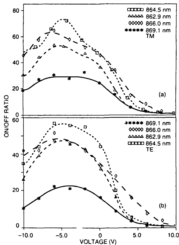
Fig. (1) ON/OFF ratio as a function of voltage at several wavelengths for (a) TM polarized light (b) TE polarized light. Lines indicate polynomial fits to the data and every tenth data point is shown with symbol.
