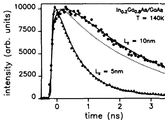
Fig.4 Time-resolved PL of \text{In}_{0.2}\text{Ga}_{0.8}\text{As}/\text{GaAs} quantum wells ( L_z=5\text{nm} and L_z=10\text{nm} ). Fits are included as described in the text
