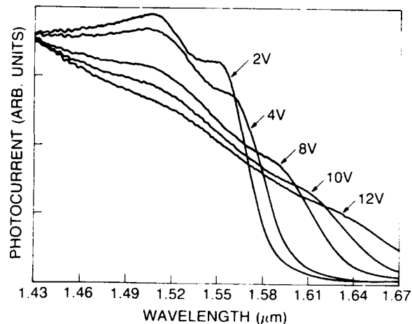
Figure 1: Photocurrent spectra of sample with 80 Å GaInAs quantum wells and 120 Å AlGaInAs barriers.
