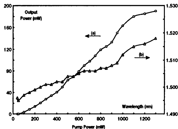
Figure 3: EX-SEL CW output power (a) and center-frequency (b) as a function of pump power (1.32 \mu\text{m} CW Nd:YAG).
