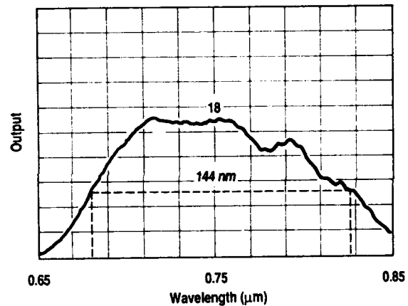
Figure 5. Electroluminescence spectrum from broadband SLED at room temperature.
