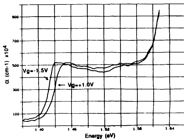
Figure 3 Absorption spectra for the two charge states of the device.
