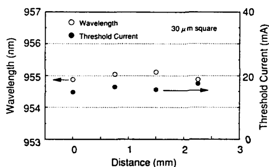
Fig.3 Wavelength and threshold current dependence on position
