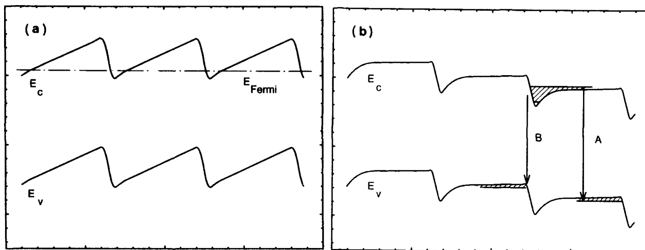
Fig. 1 - Three periods of the calculated energy band diagram of the \delta -doped superlattice. a) Structure at equilibrium. b) Band diagram after photogeneration of 5 \times 10^{12} \text{ cm}^{-2} electron-hole pairs in each well. Carriers recombine in flat band regions (A) and via tunneling assisted recombination (B).
