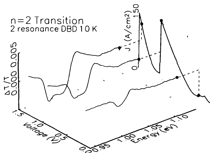
FIG. 4. DAS spectra for a two resonance sample at various modulation voltages for photon energies corresponding to the second QW resonance.
