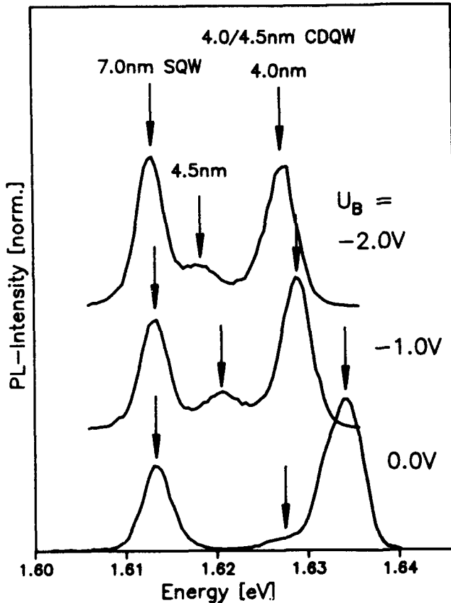
Fig. 2: Low temperature PL-spectra of a CDQW-structure at different reverse voltages V .
