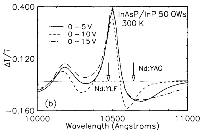
FIG. 2. \text{InAs}_y\text{P}_{1-y} / \text{InP} absorption spectra and \Delta T/T data at 300 K.
