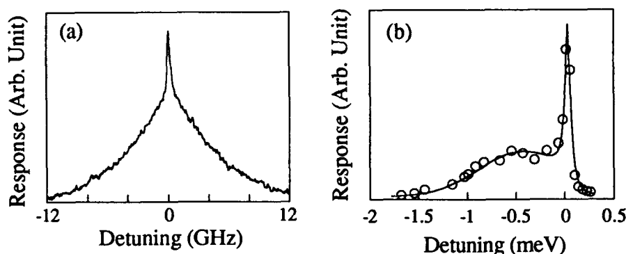
Figure 1. (a) The FDFWM response leading to a line shape determined by decay of the excitation (tuning \omega_2 ). Two components are observed at 10K due to recombination (the narrow component) and spectral diffusion (the fast component). (b) The FDFWM line shape obtained by tuning \omega_3 corresponding to the homogeneous line shape (the sharp resonance) and a low energy tail due to spectral diffusion. Zero detuning in (b) corresponds to \omega_3 = \omega_1 , \omega_1 and \omega_2 1.5 meV below absorption line center. The line shape is obtained at 5K.
