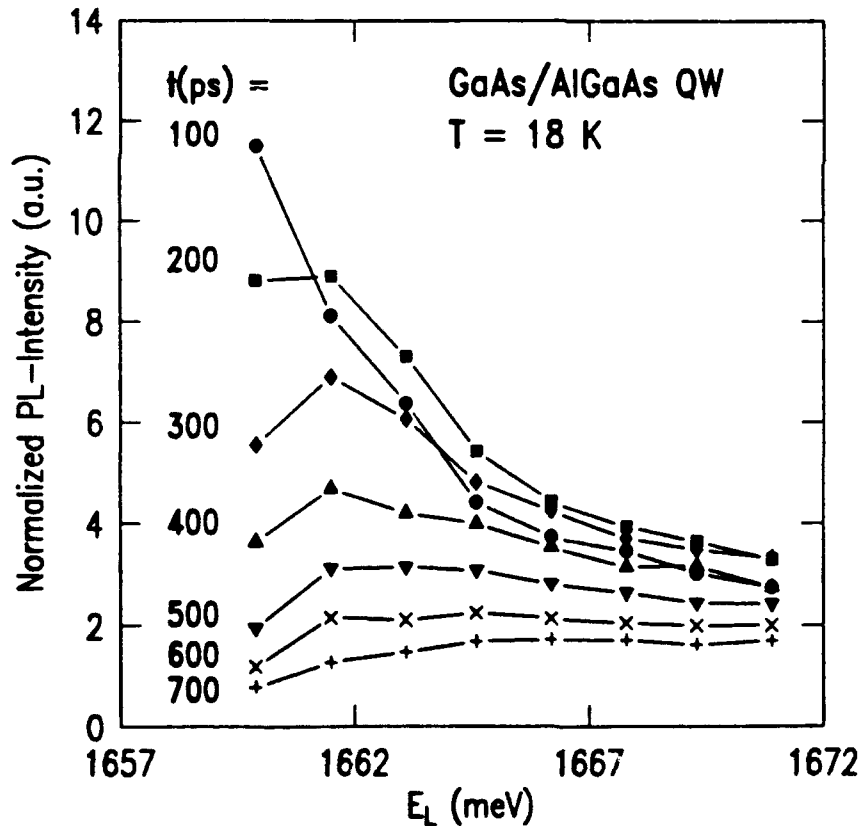
FIG. 3. Normalized photoluminescence intensity vs. excitation energy for various discrete times. The detection energy E_{det} = 1658.3 meV. The experimental conditions are the same as in FIG. 1.
