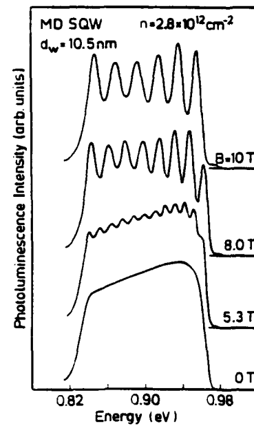
Fig. 2. Magnetoluminescence spectra of sample c of different magnetic fields, showing that the electrons at different occupied Landau levels recombine with localized holes.
