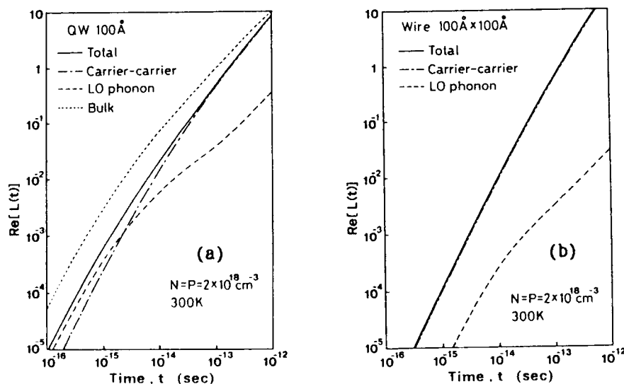
Fig. 1 Real part of phase damping factor L(t) at carrier density of 2 \times 10^{18} \text{ cm}^{-3} . (a) 100Å QW, (b) 100Åx100Å quantum wire.
