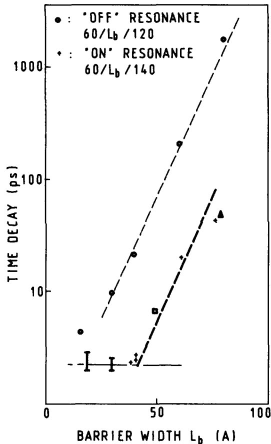
Fig.1: Decay time of the NW luminescence as a function of the barrier thickness for two series of samples: (o) "off resonance", and (+) on resonance". On resonance decay times observed by Oberli et al [3] ( \sigma ) and by Alexander et al [4] ( \Delta ) are also plotted.
