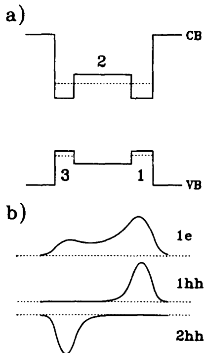
Fig. 1: Eigen states (a) and wave functions (b) of a coupled double quantum well system with slightly different wells.
