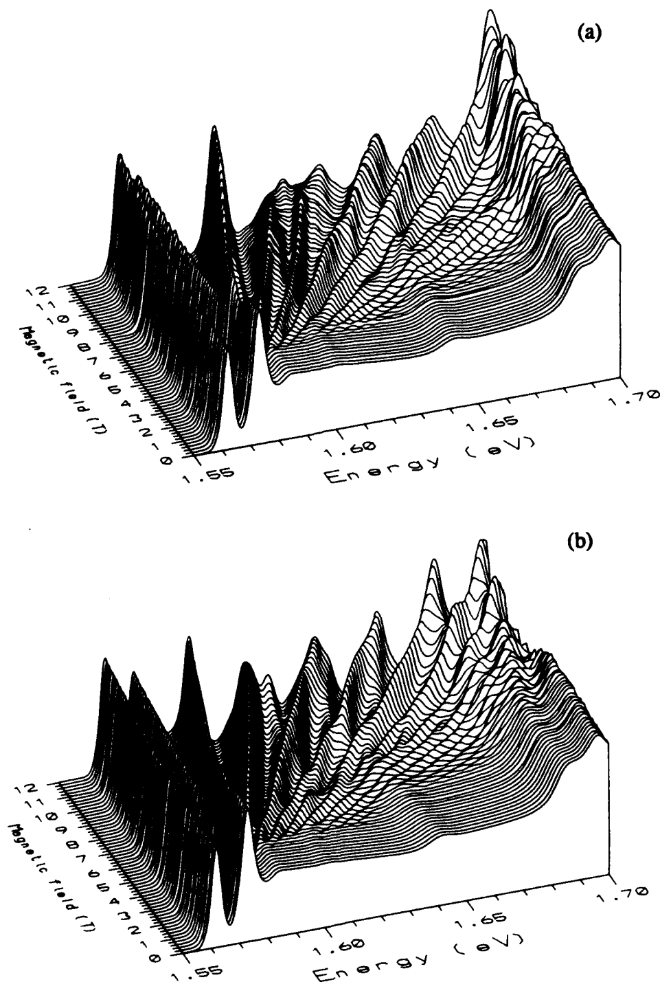
Figure 1 Linear absorption spectra for (a) \sigma^- and (b) \sigma^+ circularly polarized light.
