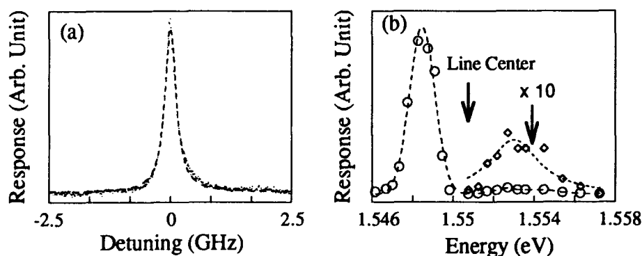
Figure 2. The FDFWM response obtained 2 meV above absorption line center. (a) Tuning \omega_2 shows a single resonance due to recombination. (b) Tuning \omega_3 , we see two resonances. The upper resonance is the homogeneously broadened resonance from delocalized excitons. The lower resonance is due to excitons which have localized. The energy of the lower resonance corresponds to the luminescence maximum.
