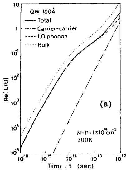
Fig. 4 Real part of phase damping factor L(t) at carrier density of 1 \times 10^{14} \text{ cm}^{-3} . (a) 100 \text{ \AA} QW, (b) 100 \text{ \AA} \times 100 \text{ \AA} quantum wire.
