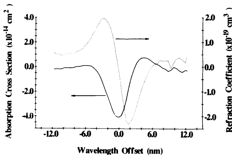
Fig.2 Spectral dependence of nonlinear optical coefficients for 2x5x8 sample.
