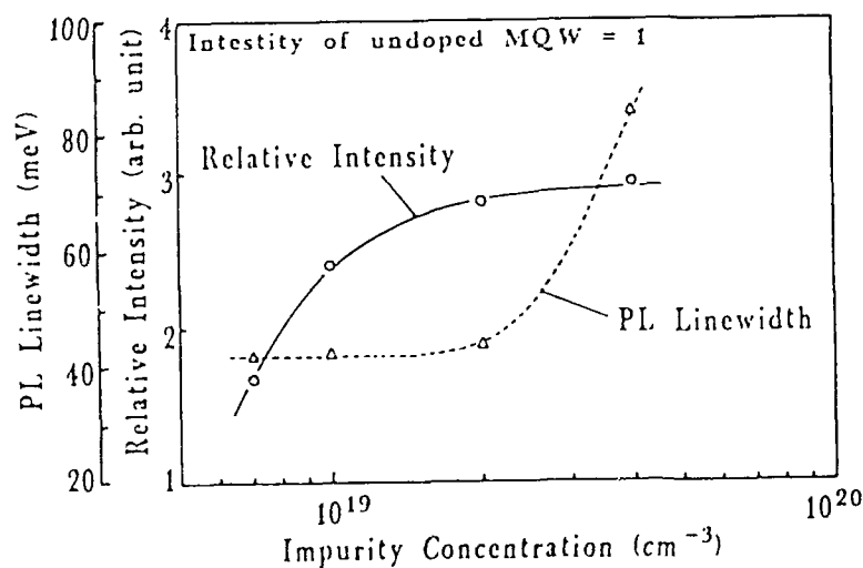
Fig. 1 PL intensity and linewidth of modulation doped QWs vs impurity level in InP barriers at room temperature. Well width was about 80Å and intensities were relative to an undoped QW of the same structure.
