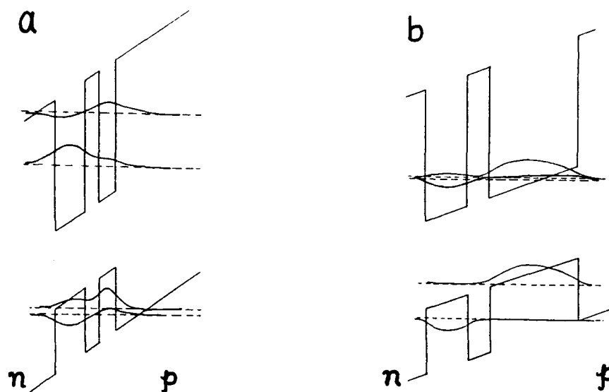
Fig. 1 (a) reverse-biased ACQW structure with wider well closer to the n-type region, which was designed and used for this experiment. (b) reverse-biased ACQW structure with wider well closer to the p-type region.
