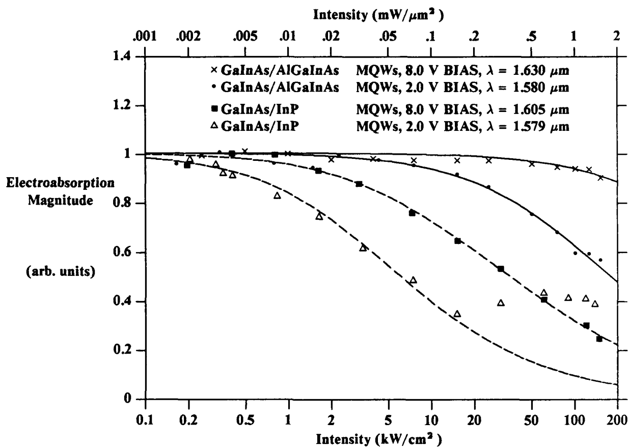
Figure 3: Electroabsorption saturation of GaInAs quantum well samples. The figure shows that samples with AlGaInAs barriers have approximately 30 times higher saturation intensities than similar samples with InP barriers.
