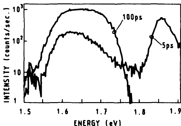
Fig.1: Luminescence spectra of a P-GRINSCH at different time delays: 5 and 100 ps.
