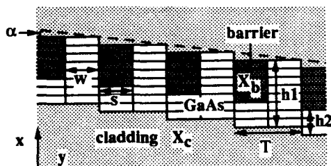
Fig.1.(b) Schematic cross sectional profile of a TSL.
