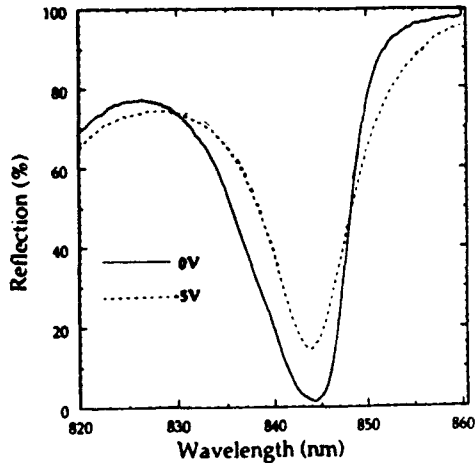
Figure 2 :- Shows the reflection spectra for the sample annealed at 930°C for 120s for different biases. We can clearly see that the heavy hole has been blue-shifted by 31meV into the resonance to enable normally-off operation of the device.
