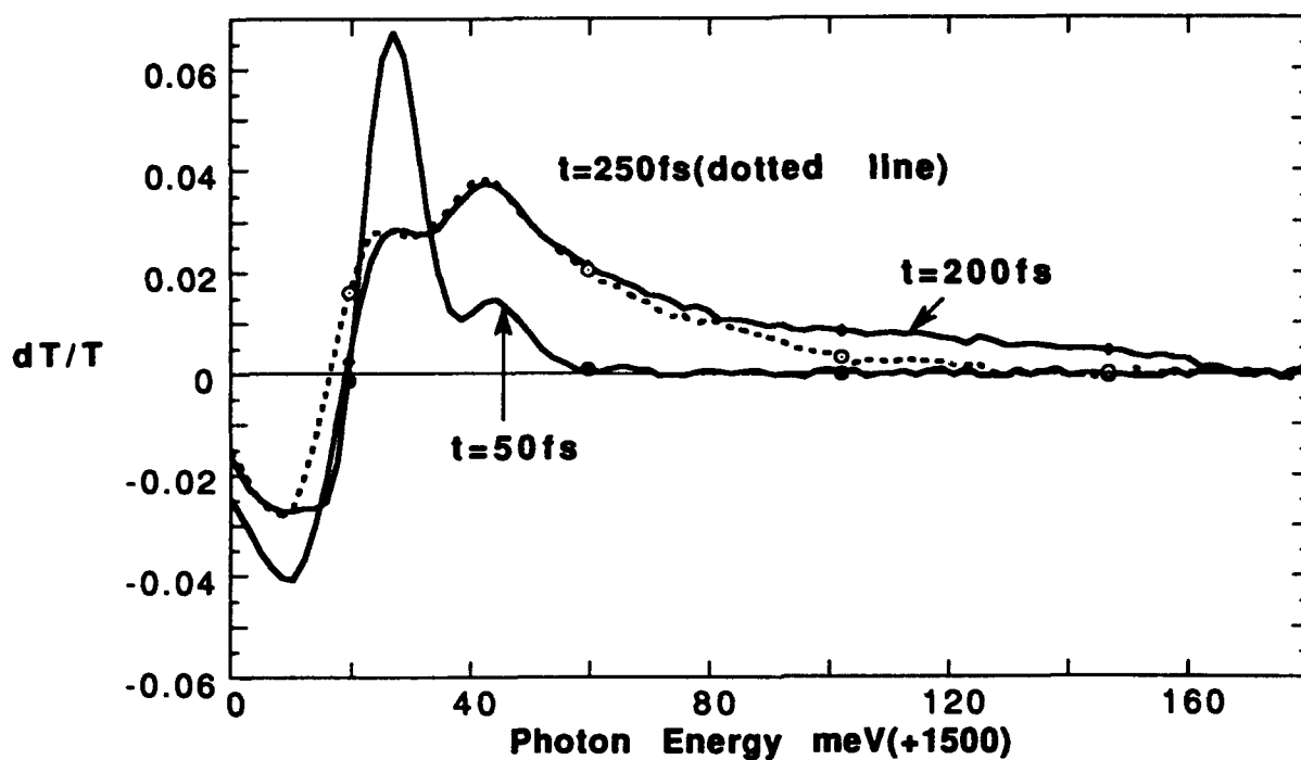
Fig.1 Differential transmission spectra, (T_E - T)/T where T_E is transmissivity with E=16\text{ kV/cm} , T is without the field. Pump is always on.
