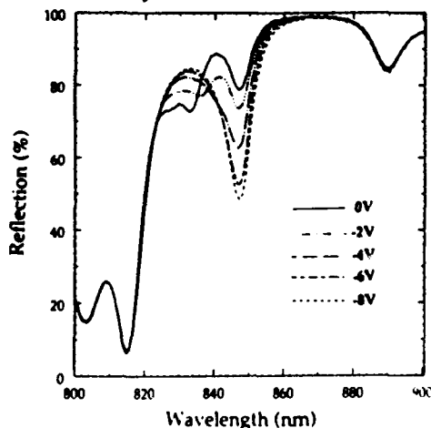
Figure 5 :- This shows the reflectivity spectra for the device of Fig 4. We can clearly see, that as a bias is applied it behaves as a normally-on AFPM.
