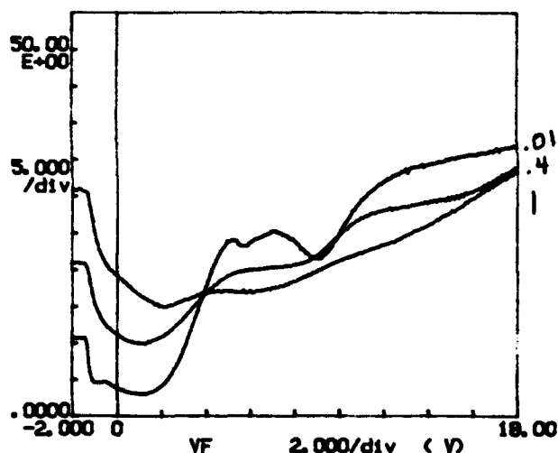
Fig. 7: Reflectivity vs. voltage for 0.01, 0.4 and 1 mW for a x=0.3 sample with 35 angstrom barriers. This sample has more periods resulting in higher contrast but larger insertion loss.
