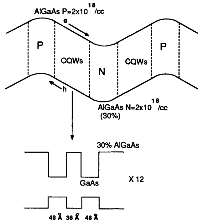
Fig 1. The energy band diagram for a multiple quantum well hetero n-i-p-i structure with coupled quantum wells.
