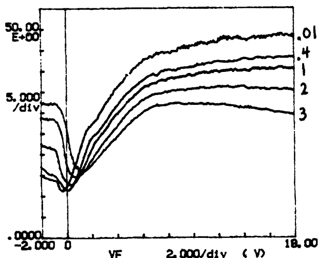
Fig. 6: Reflectivity vs. voltage for 0.01, 0.4, 1, 2, 3 mW (3 \mu m spot) for the x=0.02 sample.
