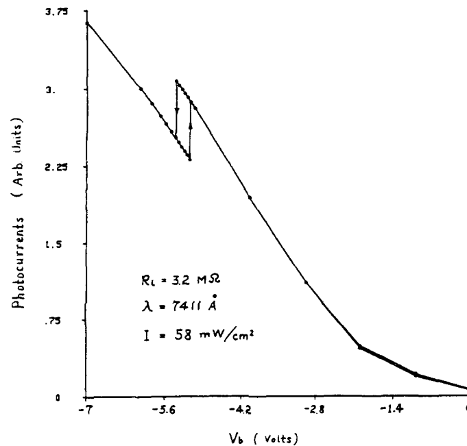
Fig. 4 Optical bistability is observed at the laser intensity \sim 58 \text{ mW/cm}^2 , external resistance \sim 3.2 \text{ M}\Omega , and laser wavelength \sim 7411 \text{ \AA} (heavy-hole excitonic transition).
