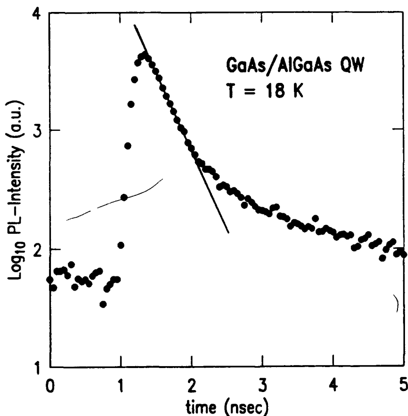
FIG. 1. Photoluminescence intensity as a function of time for a nominally 25Å thick GaAs/AlGaAs quantum well. The excitation energy E_L = 1666.2 meV, the detection energy E_{\text{det}} = 1662.8 meV. The straight line indicates how \tau_{\text{PL}} is obtained from the inverse of the steepest slope.
