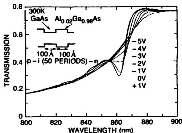
Fig. 2: Transmission of x=0.02 sample.
