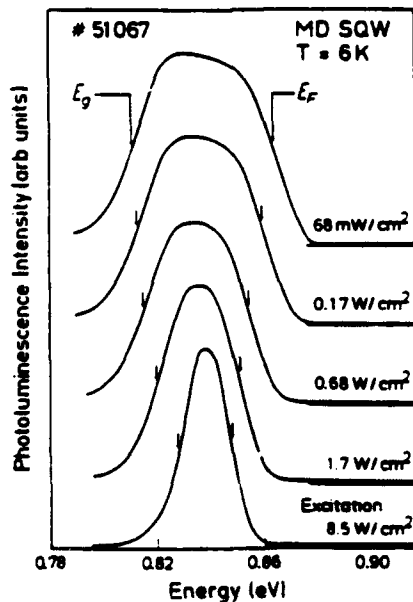
Fig. 3. Excitation dependent photoluminescence spectra of sample a with a well width of 10.5 nm. The band gap and Fermi edge are given by the middle points of the high- and low-energy edges, respectively.
