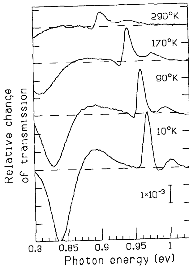
Fig. 1. Differential absorption spectra at 4 different temperatures measured at V_{peak} .
