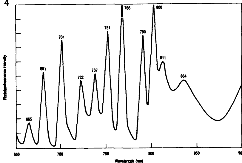
Figure 4. Photoluminescence spectrum at 10K showing the emission from each of the ten wells in the active region.
