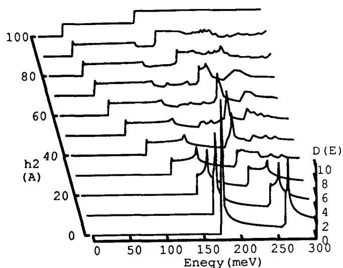
Fig.3. Conduction band density of states ( 10^9/\text{eV}\cdot\text{cm} ) of a TSL with x_b=1.0 , x_c=0.40 , W=S=40\text{\AA} , h_1=100\text{\AA} .
