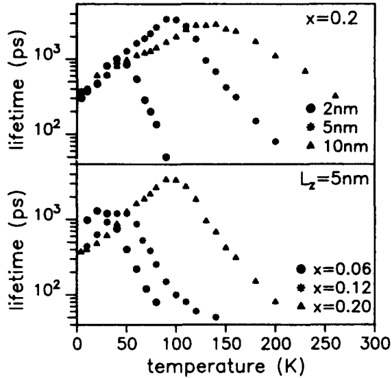
Fig.2 PL lifetime versus temperature for different well widths L_z ( x=0.2 ; top) and for different In-contents x ( L_z=5\text{nm} ; bottom)
