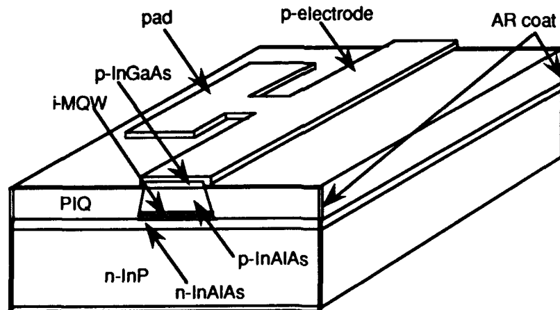
Fig.1 Schematic view of the InGaAs/InAlAs MQW EA modulator.
