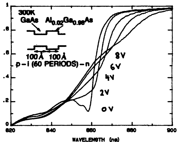
Fig. 5: Reflection of x=0.02 sample with integral mirror.
