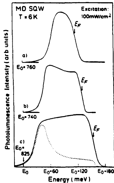
Fig. 1. Photoluminescence spectra of \text{Ga}_{0.47}\text{In}_{0.53}\text{As}/\text{Al}_{0.48}\text{In}_{0.52}\text{As} MD SQWs with different electron sheet concentrations under low excitation at 6K. The energy bandwidths are 52.2 meV, 85.0 meV and 129 meV for samples a, b and c, respectively. The dashed line shows schematically the luminescence line-shape of MD SQWs without Be doping in the well.
