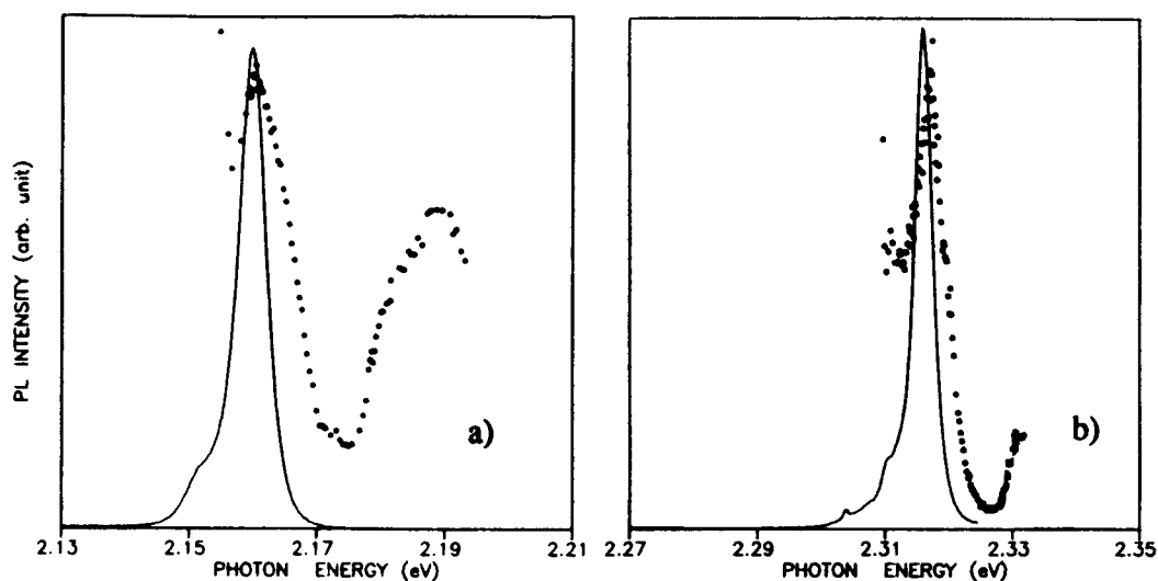
Fig. 1 PL and PLE spectra at 6K for a) sample A ( x=0.33, L_w=67\text{\AA} ) b) sample C ( x=0.10, L_w=40\text{\AA} ). Solid curves are for PL and filled circles are for PLE
