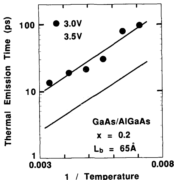
Figure 2 Thermal emission time for the sample of Fig. 1(c) against 1/T at 3.0V and 3.5V. The straight lines are fits assuming an activation energy of 49meV at 3.0 V and 47meV at 3.5V.
