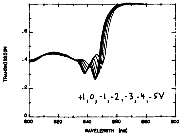
Fig. 3: Transmission of x=0.3 sample.
