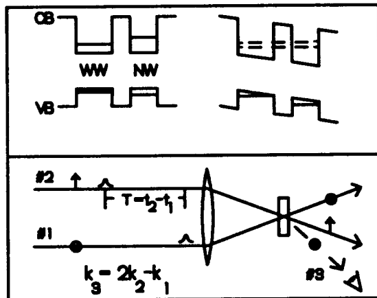
Figure 1: Top: schematic of the double well structure at resonance, for fields where the electronic levels are out of (left) and in resonance (right). Bottom: geometry of the experiment.
