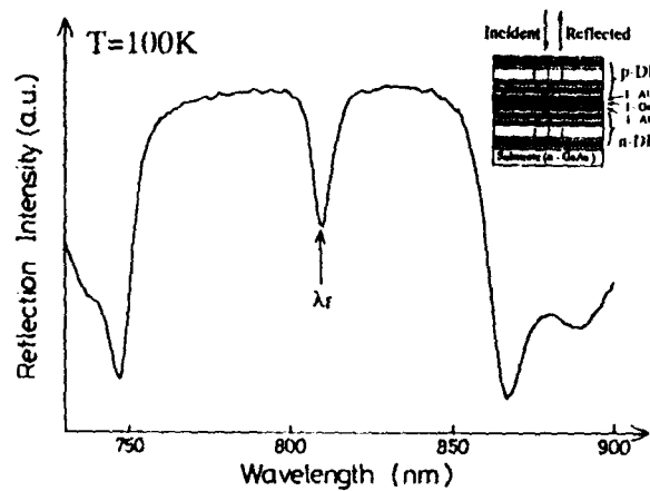
Fig.2 Experimental reflection coefficient R of a \lambda/2 -cavity as a function of probe wavelength at T=100K .
