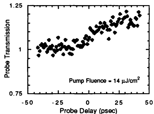
Fig. 4. At low fluences, a persistent change in transmission can be seen at 809 \text{ nm} as photocarriers swept to doped layers screen the built-in fields.
