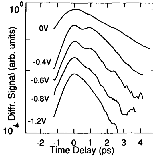
Figure 4: Diffracted signal in the DFWM experiment for various electric fields.
