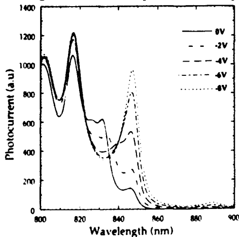
Figure 4 :- The photocurrent spectra is plotted for the sample annealed at 930°C for 180s. The heavy and light hole can both be resolved at 832nm and 827nm respectively. This means the heavy hole has been blue shifted by 52meV.
