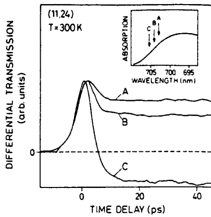
Fig.1 Differential transmission vs time delay between pump and probe pulses for the type-II (GaAs) 11 (AlAs) 24 MQW.
