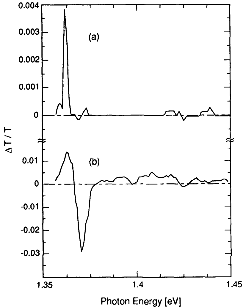
Differential transmission spectra for (a) the (100) sample and (b) the (211) sample. Both sets of data were taken with I_p = 26 \text{ W/cm}^2 and I_t = 2.9 \text{ W/cm}^2 in the samples.
