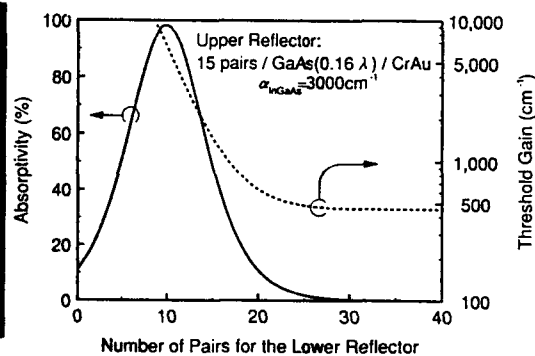
Fig.5 Calculated absorptivity and threshold gain
