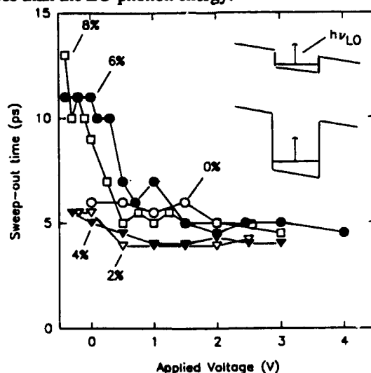
Fig.1: Experimentally determined sweep-out times versus applied reverse bias voltage for all 5 shallow quantum well samples at room-temperature. As an inset we schematically illustrate the situations when the effective barrier height is smaller or larger than the LO-phonon energy.
