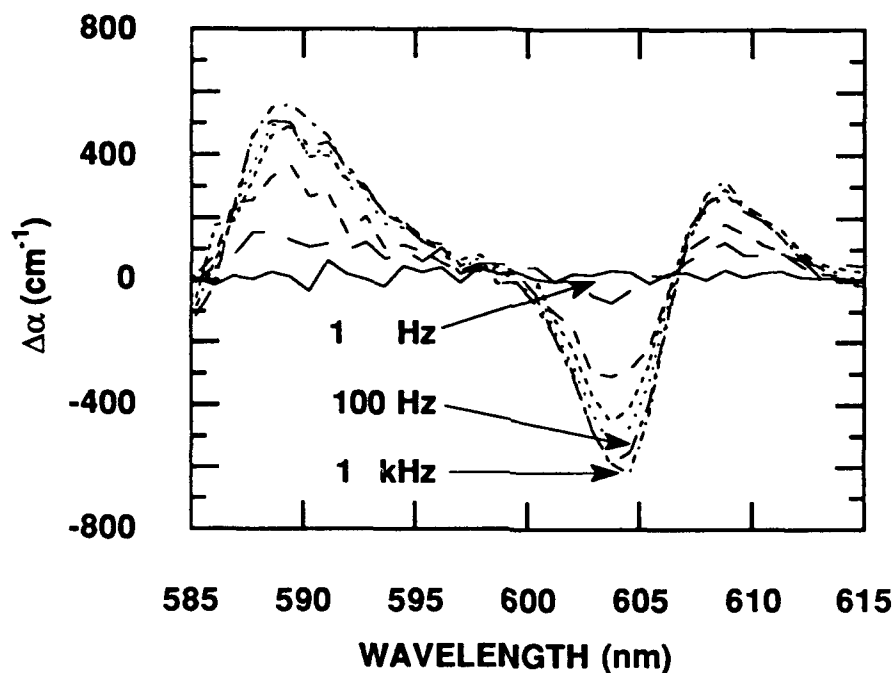
Figure 2. Change in the absorption coefficient as a function of the frequency of the applied ac field for a multiple quantum well sandwiched between dielectric layers.
