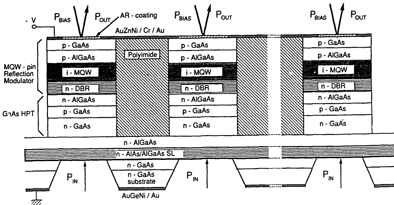
Fig.1. Cross-sectional view of photonic gate arrays.
