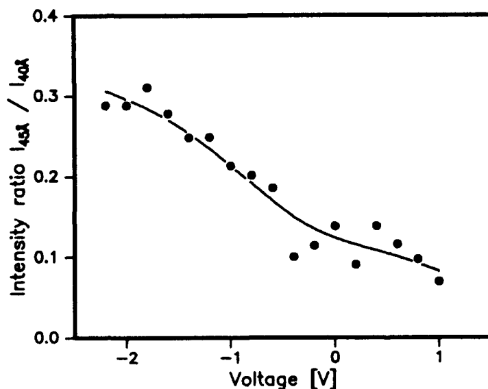
Fig. 3: Ratio of the PL-intensity of the 45\text{\AA} -well and the 40\text{\AA} -well as a function of the applied voltage.
