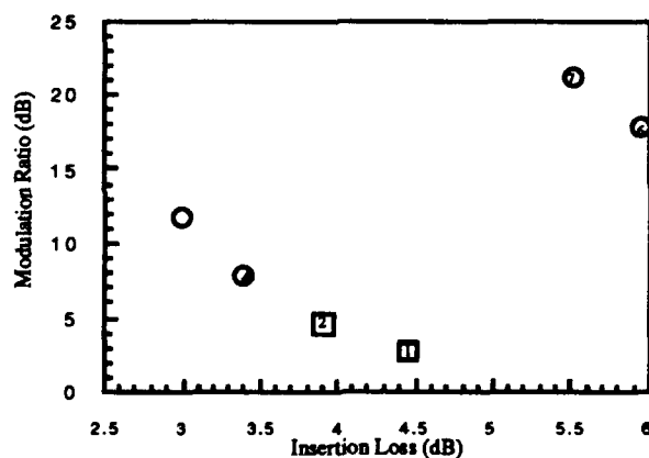
Fig. 5 Modulation ratio vs. insertion loss for previously reported normally-off reflection (circles) and transmission (squares) modulators. The numbers correspond to references. Our device is the open circle.
