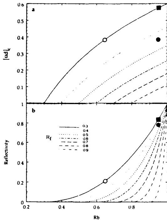
Figure 1. a) The critical amount of absorber [\alpha d]_c required to zero the overall reflectivity and b) reflectivity of a cavity with no absorption, as a function of the reflectivity of the back mirror R_b , for different front reflectivities R_f .
