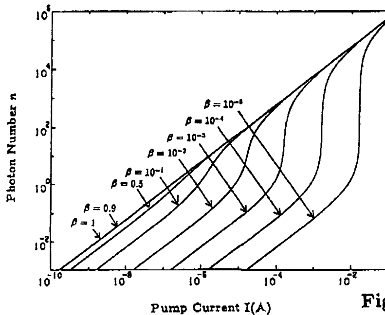
Fig. 2 Internal photon number n_0 vs. pump current I as a function of spontaneous emission coefficient \beta . n_{sp} = 1 and \omega = 10^{12} \text{ s}^{-1}
