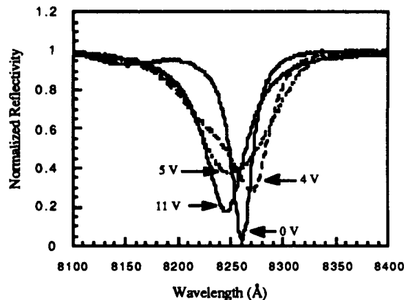
FIG. 2. Normalized reflection versus wavelength at various reverse bias voltages.
