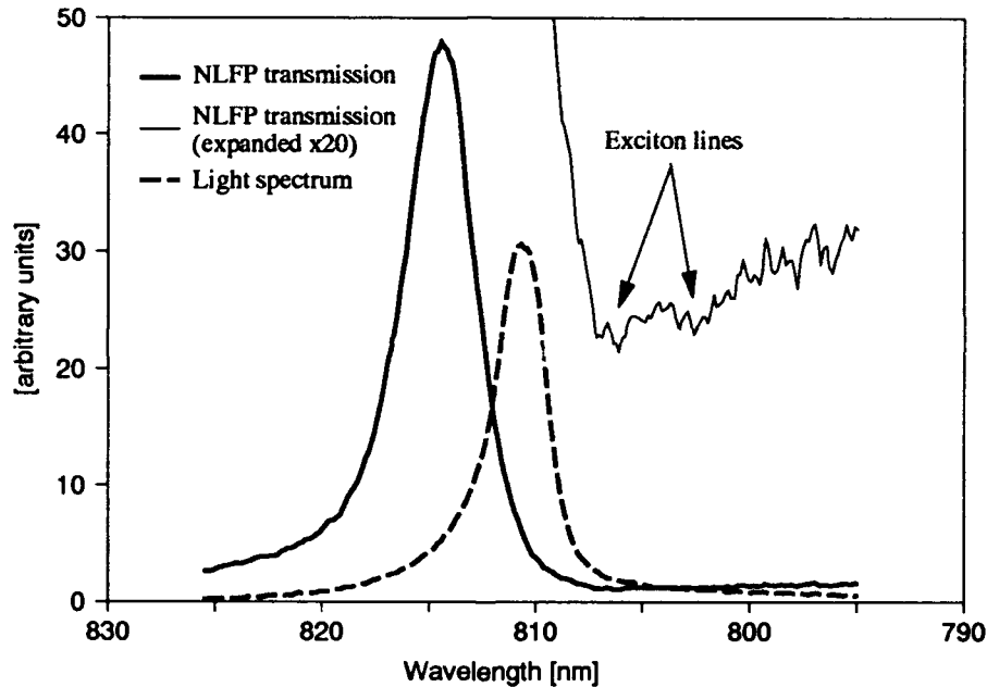
Figure 2: Transmission of the NLFP (thick solid line), expansion of this curve (thin solid line), spectrum of the light pulses (dashed line).
