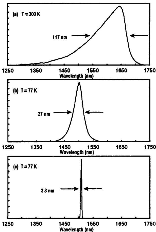
Figure 2: InGaAs/InP MQW luminescence spectra at 300 K (a) and 77 K (b), EX-SEL lasing spectrum at 77 K (c).
