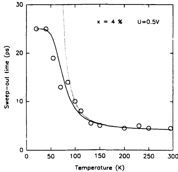
Fig.2: Temperature dependence of the sweep-out times for the x = 4\% sample at an applied voltage of 0.5 Volt. The dotted and solid curves represent calculated sweep-out times \tau_{so} according to our simple model ( for details see text ).
