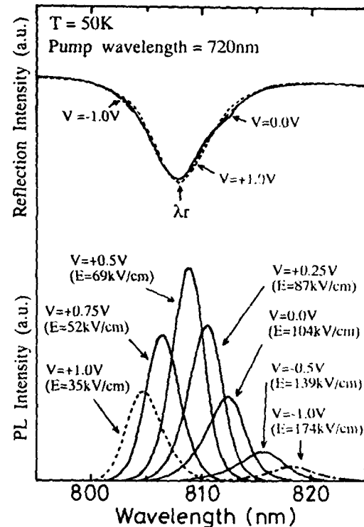
Fig.3 The spontaneous emission and reflection spectra for different voltages (different electric fields) in the (\lambda/2) -cavity diode at T=50K .
