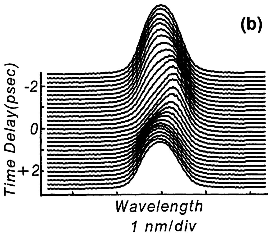
Fig.(3) Time resolved spectra of the probe pulse for (a) input pulses of 560 fsec, and (b) input pulses of 2 psec.
