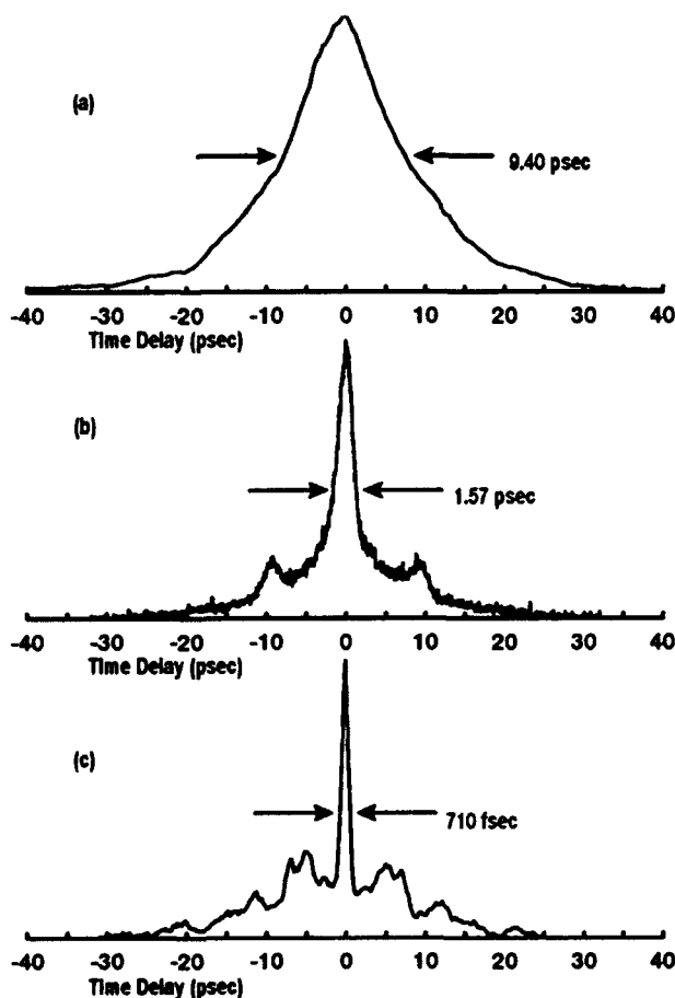
Figure 5: EX-SEL autocorrelation traces. FWHM pulse widths are (a) 9.4 psec directly, (b) 1.57 psec when compressed by a grating-pair, and (c) 710 fsec when compressed by a fiber.
