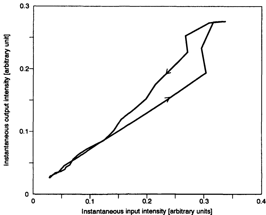
Figure 4: Instantaneous input intensity versus instantaneous output intensity. The output is previously shifted by 56 fs to cancel the linear NLFP response time.
