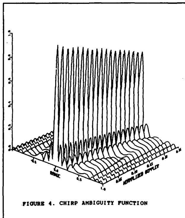
Figure 4 provides a specific example of the ambiguity function associated with Chirp pulse compression, computed for a time duration (T)-swept bandwidth (Δf) product of 15. Only the upper
