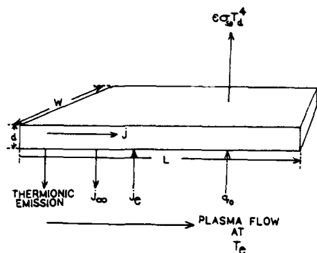
Fig. 1 The hollow cylindrical anode is shown in this idealization as a long thin slab of length L , width W , and thickness d .
