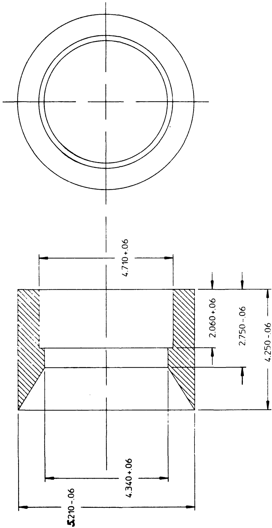
Figure 7. Case cap support drawing
