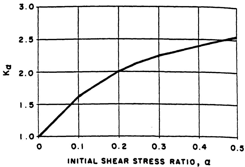
Figure 34. Folsom gravel K_\alpha (Reference 17)
