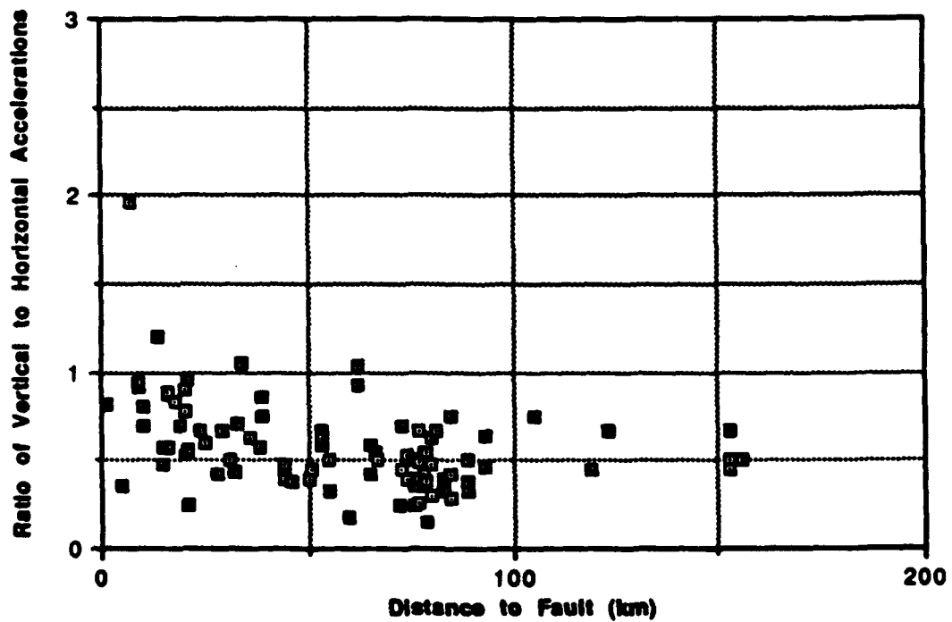
Figure 4. Ratio of vertical to horizontal acceleration, average of horizontal components. ( Reference 1)
