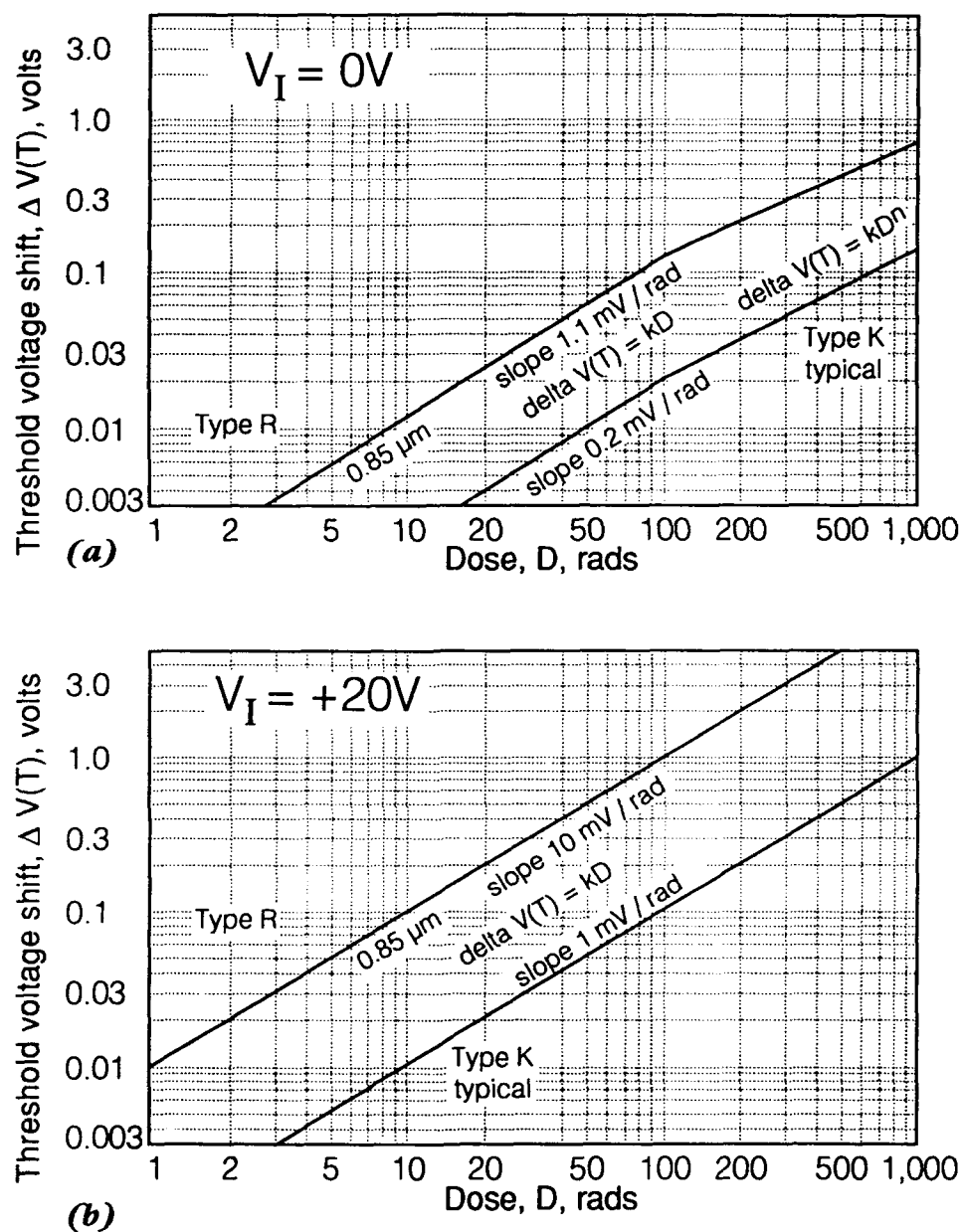
Fig. 5.1 Nominal response curves for the TOT500 RADFET, in two modes (a) Zero bias during irradiation ( V_I = 0 ) (b) Positive bias during irradiation ( V_I = +20V )
