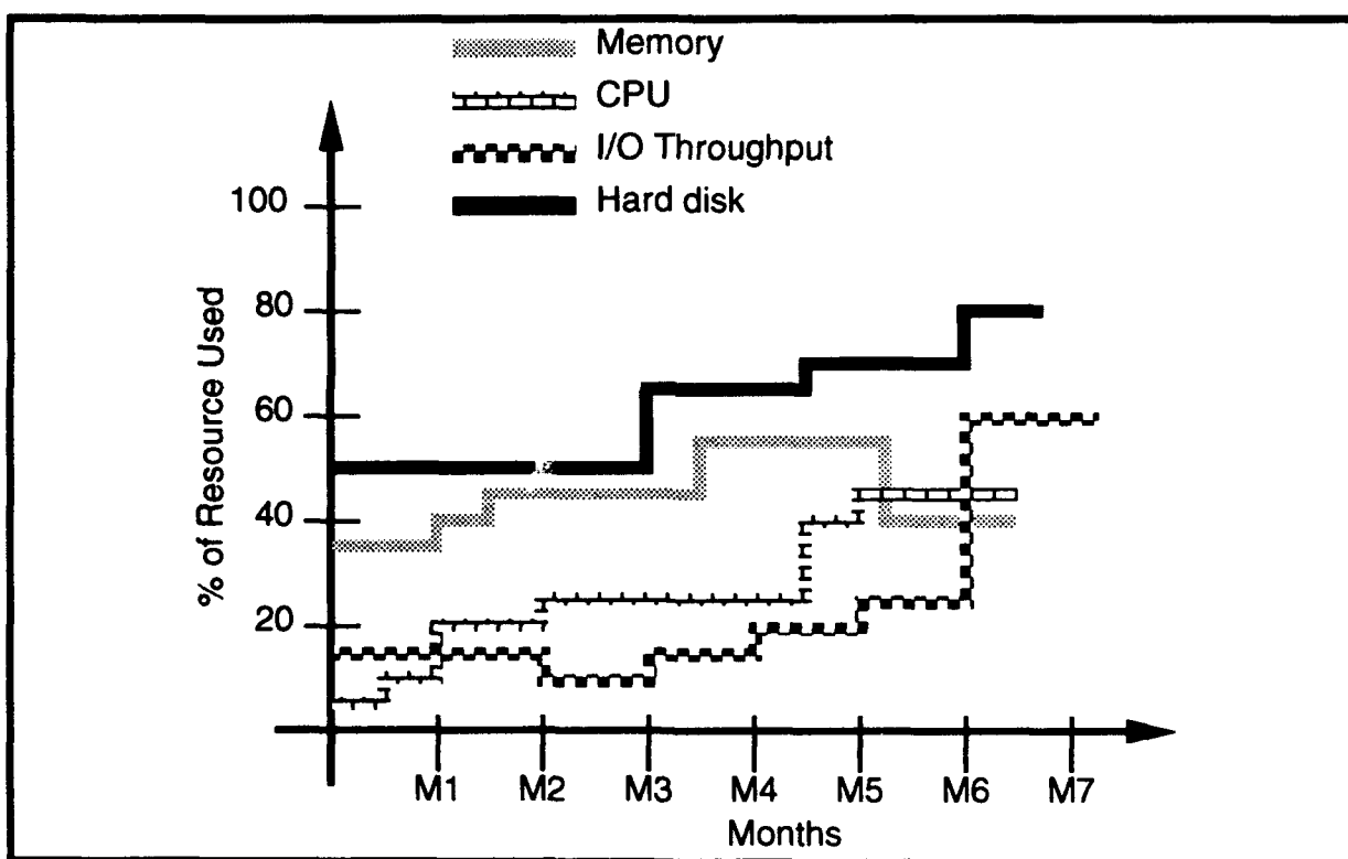
Figure 3-17 Sample Computer Resource Utilization Measure
