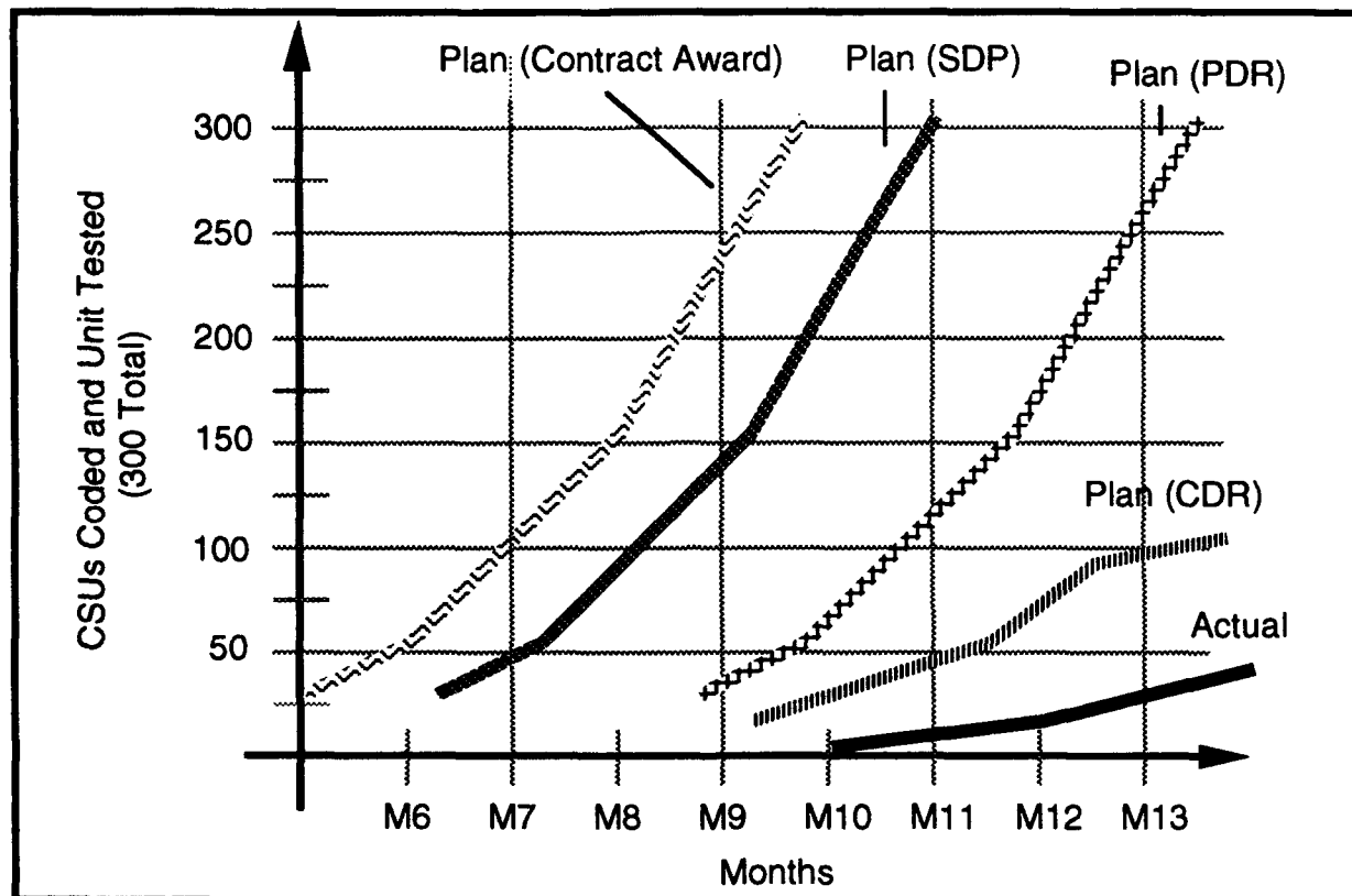
Figure 2-2 Example Showing How to Track Multiple Plans
