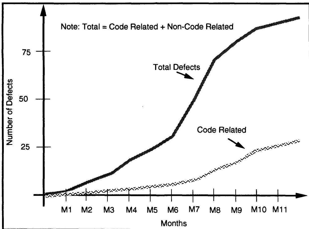
Figure 3-13 Example Illustrating the Need for Understanding Software Defects Discovered
