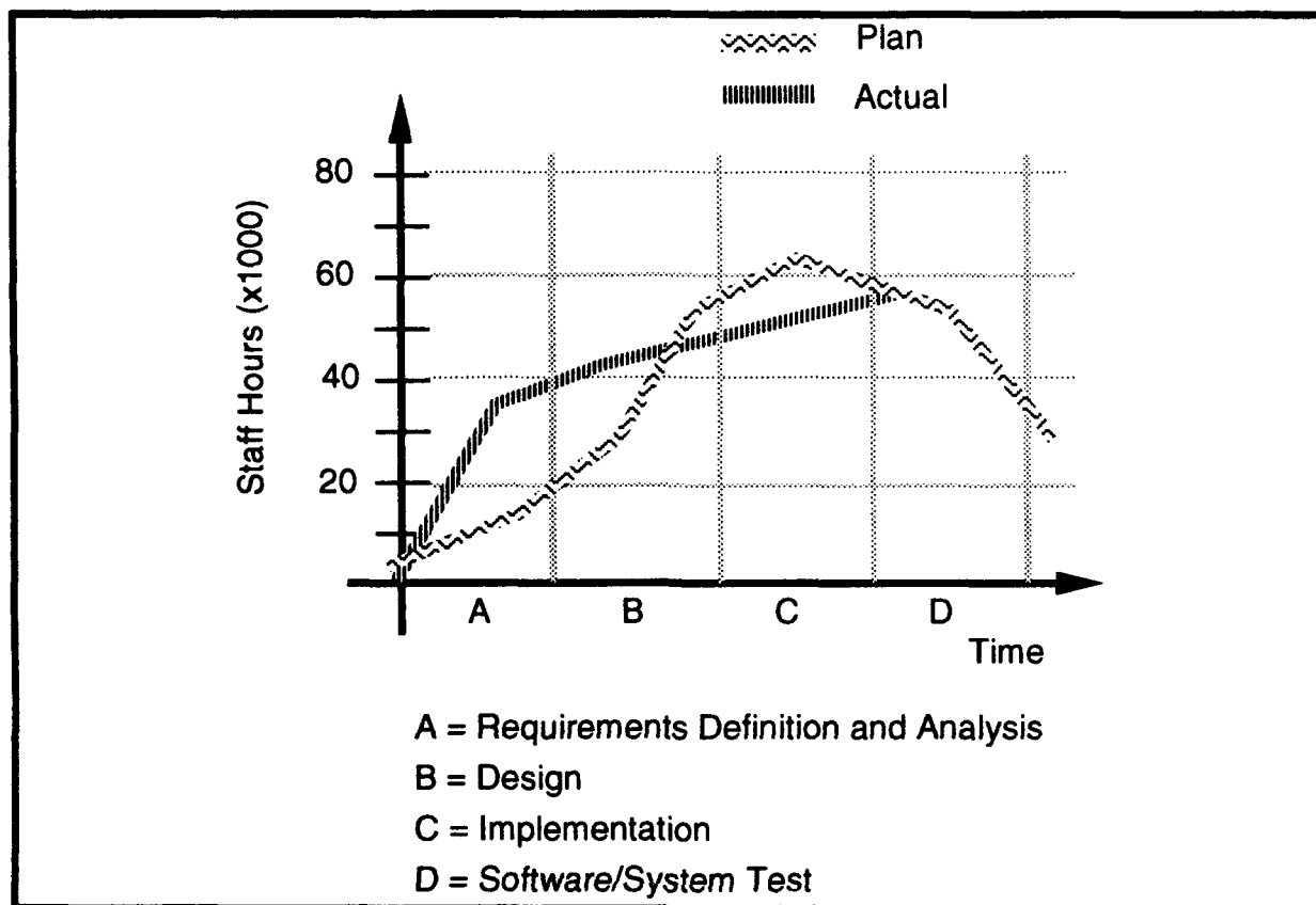
Figure 3-5 Sample Monthly Staff Effort Measure
