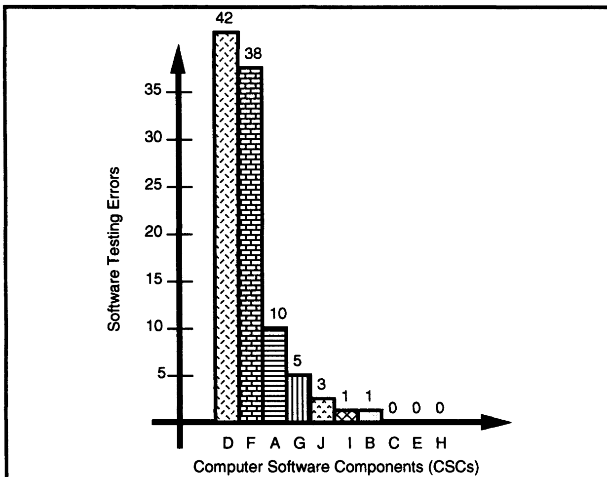
Figure 3-16 Example of Pareto Analysis Showing Defects Per CSC
