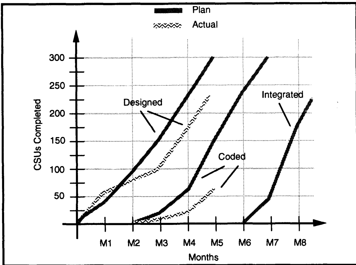
Figure 3-10 Sample Development Progress Measure
