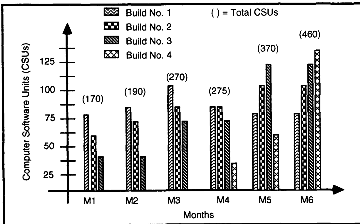
Figure 3-2 Sample Software Size Measure - CSU Per Build
