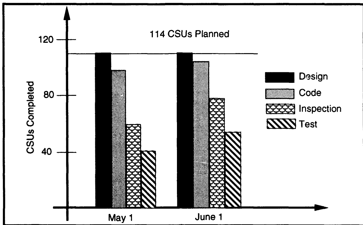
Figure 3-11 Example Showing CSUs That Have Completed Key Process Steps
