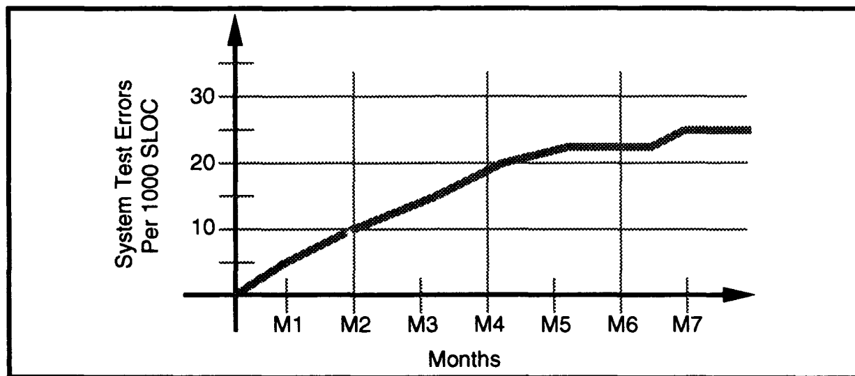
Figure 3-14 Sample Defect Density Measure
