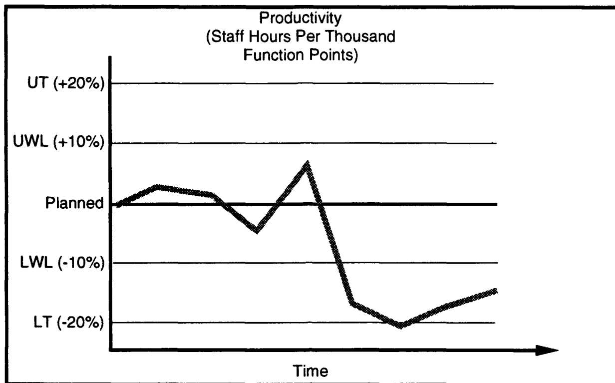
Figure 4-6 Example of Statistical Analysis Using Productivity
