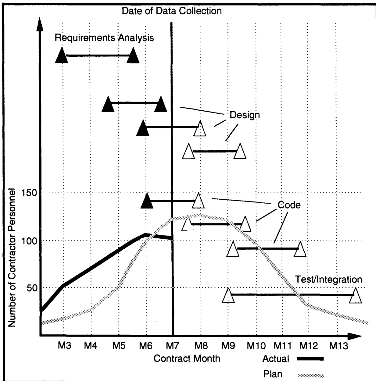
Figure 4-3 Example of Multi-Metric Relationship Analysis
