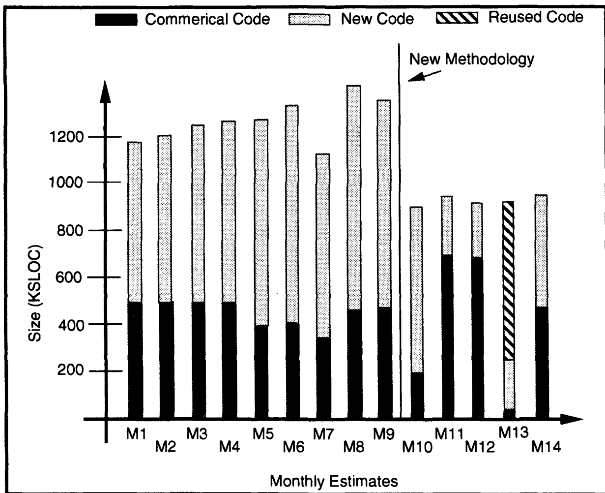
Figure 2-1 Example Illustrating the Need for Understanding Data
