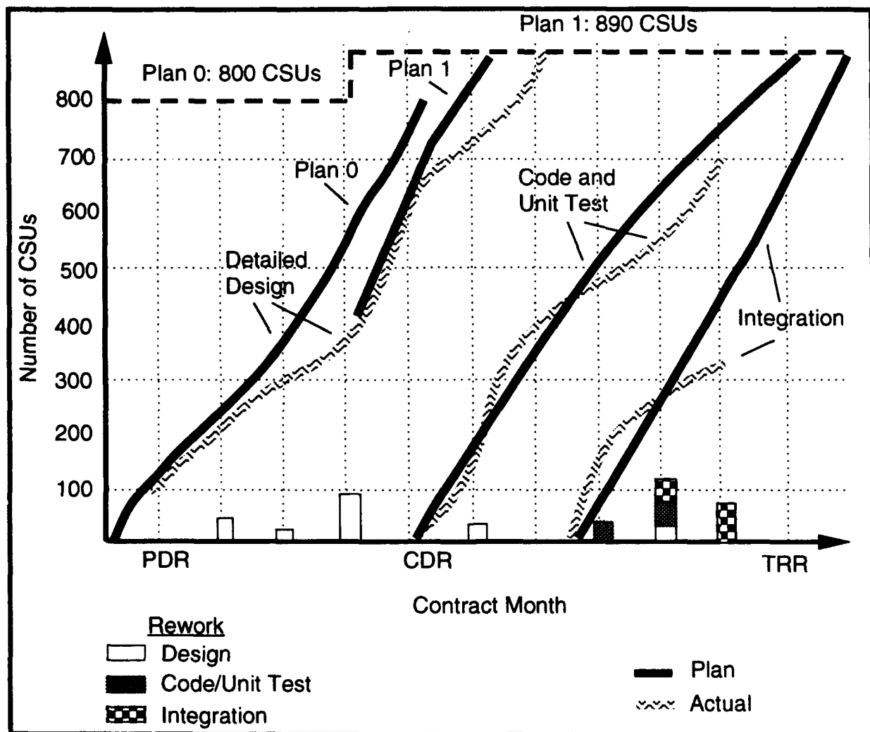
Figure 4-2 Example of Multiple Parameter Trend Analysis
