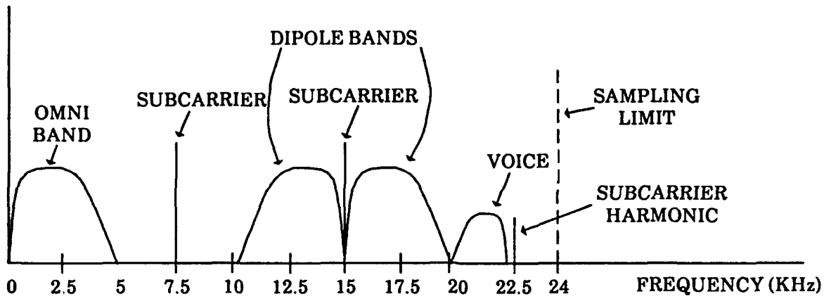
FIGURE 1. FREQUENCY SPECTRUM
