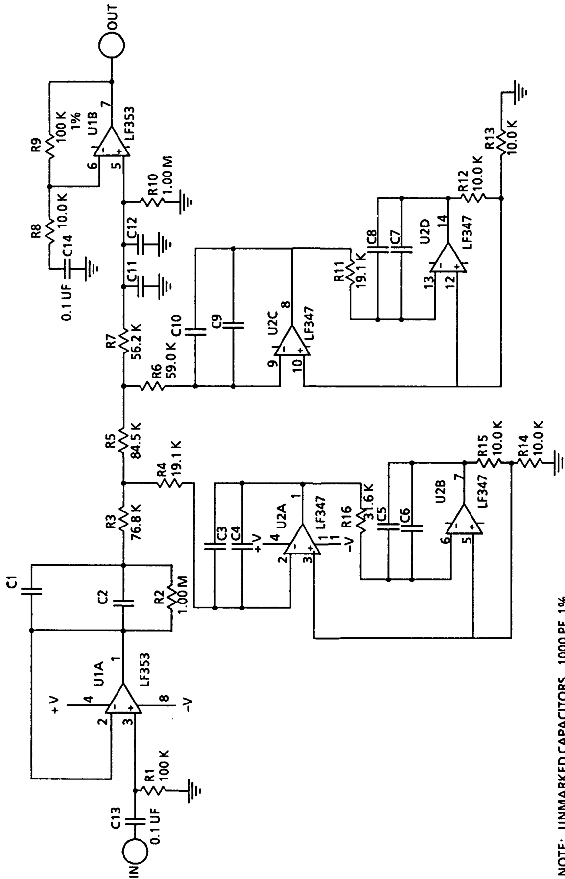
FIGURE 5. LOW-PASS FILTER
