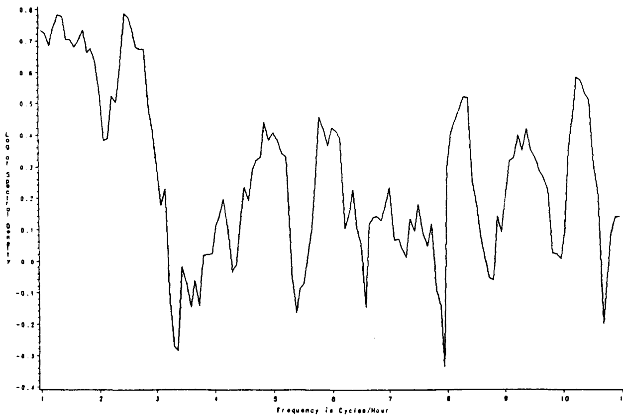
Figure 12. Power spectrum of Shemya wind speeds, 5 Oct 91, (1 < freq < 11).
