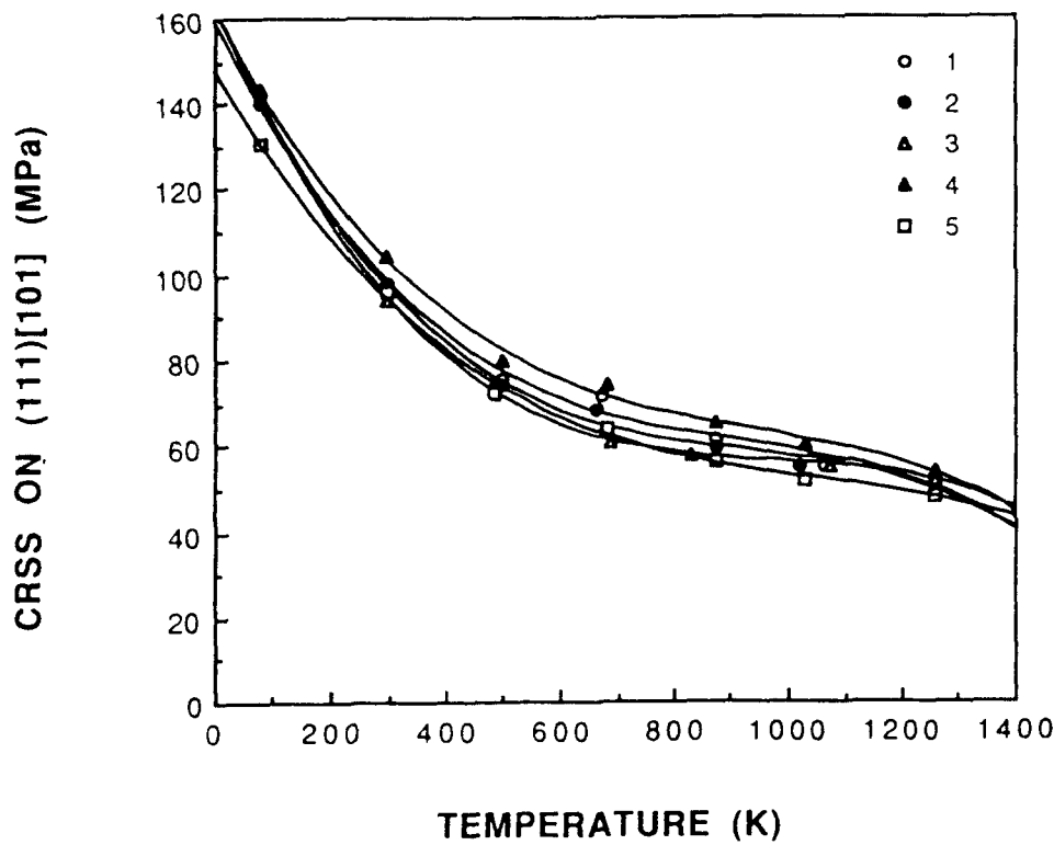
Fig. 3. (a) Stress-strain curves at room temperature and (b) temperature dependence of the CRSS for {111}<110> slip in \text{Al}_{67}\text{Ti}_{25}\text{Cr}_8 single crystals.
