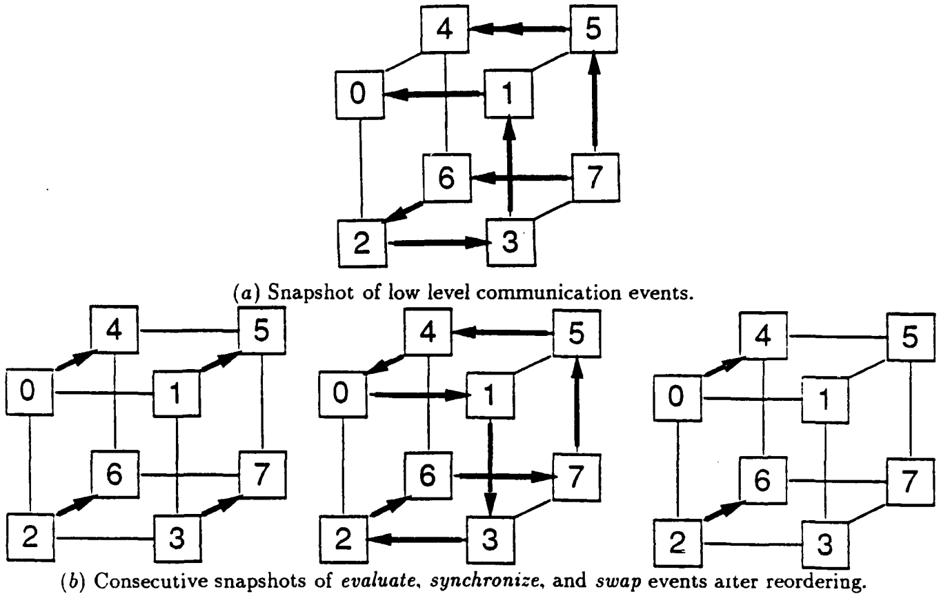
Figure 2: Traveling Salesman.
