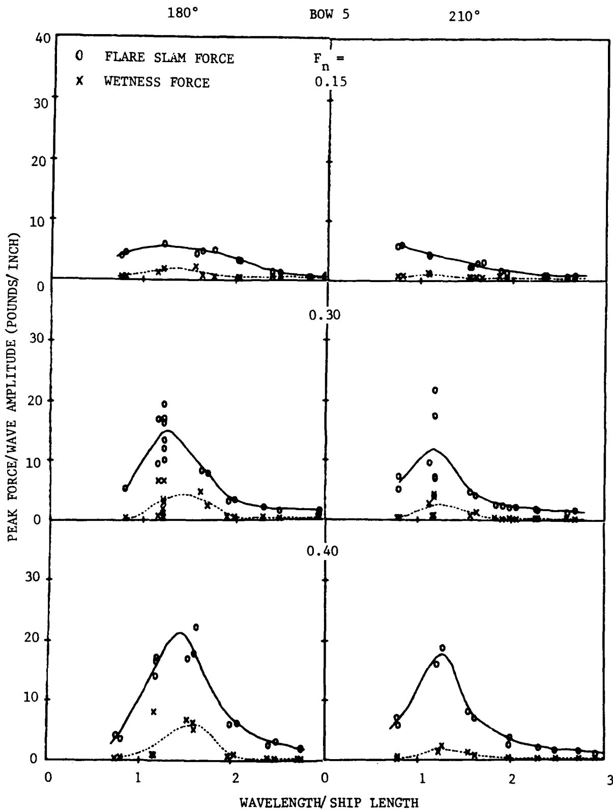
Figure 18 - Peak Flare Slam and Deck Wetness Forces Acting on Bow 5 Normalized by Wave Amplitude
