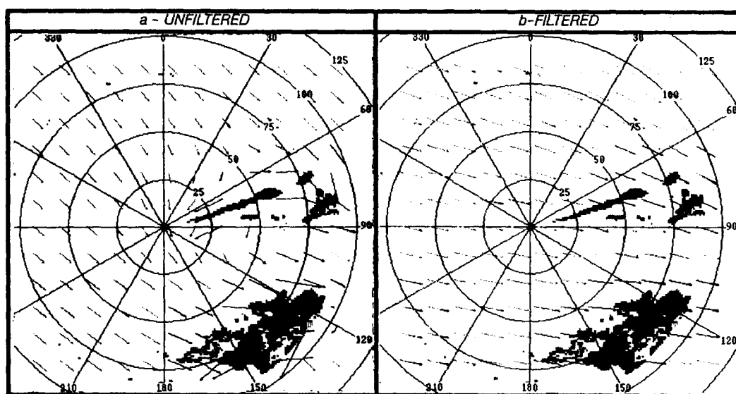
Figure 4. Storm motion internal velocity grids: a. unfiltered, b. filtered.
