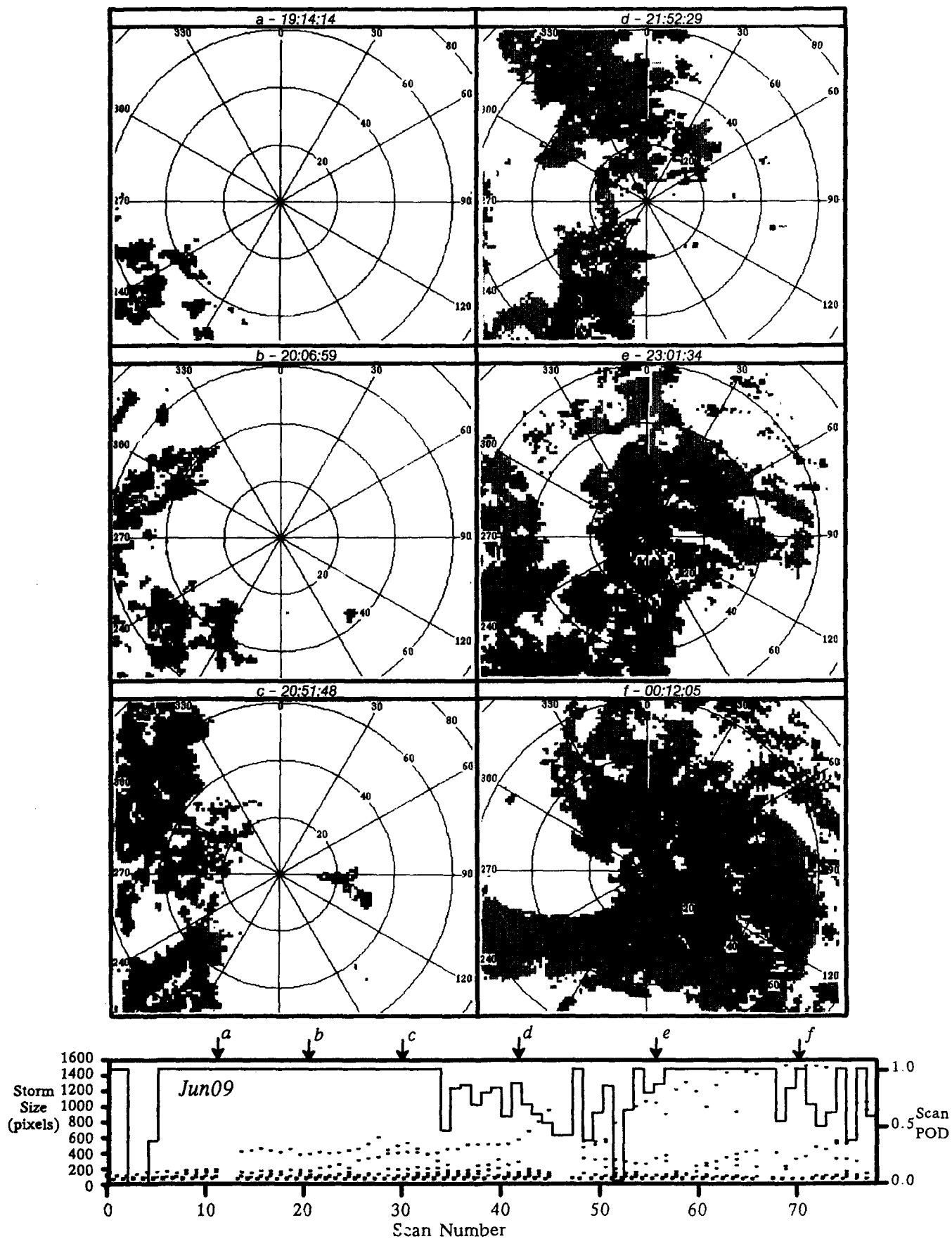
Figure 15. Tracking performance and storm evolution: Jun09.
