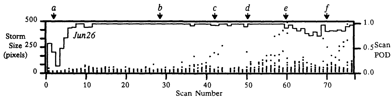
Figure 24. Tracking performance and storm evolution: Jun26.
