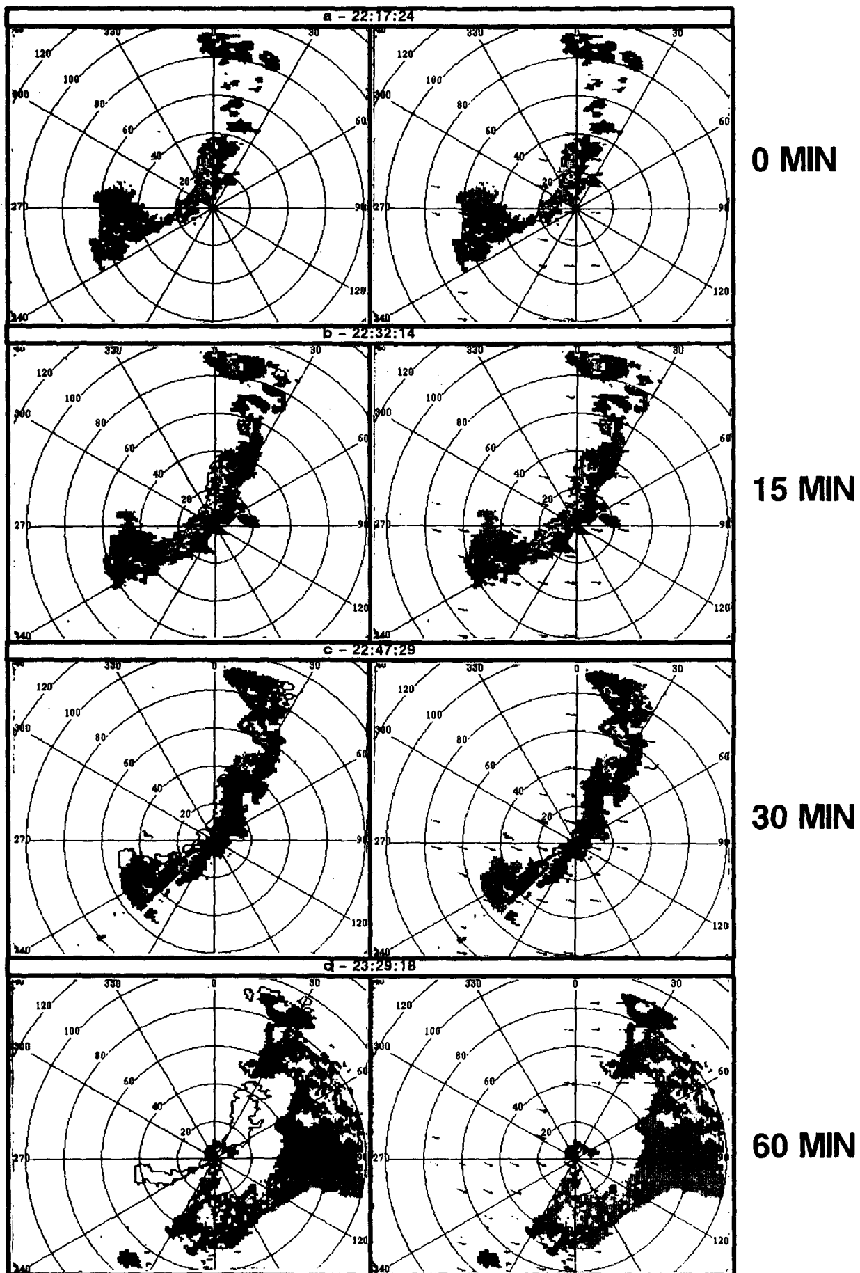
Figure 29. Extrapolation analysis: Jun15.
