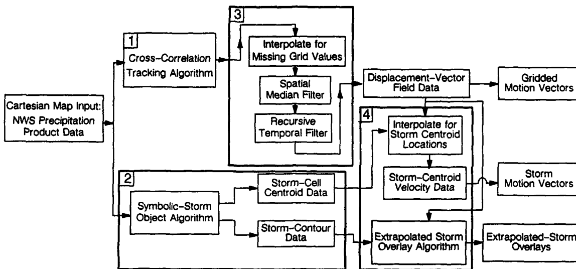
Figure 3. Storm Movement Prediction: functional organization.
