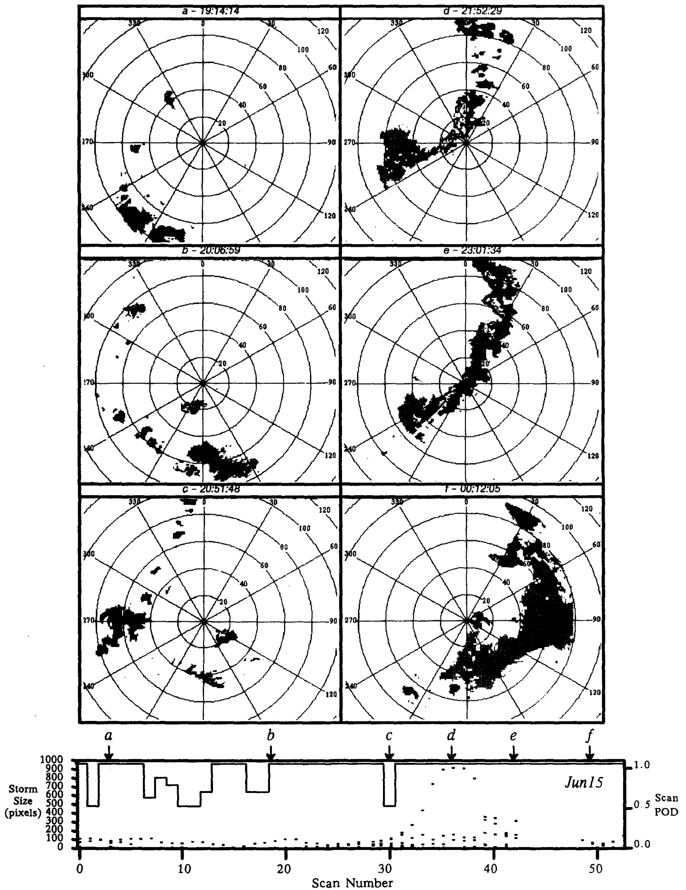
Figure 19. Tracking performance and storm evolution: Jun15.
