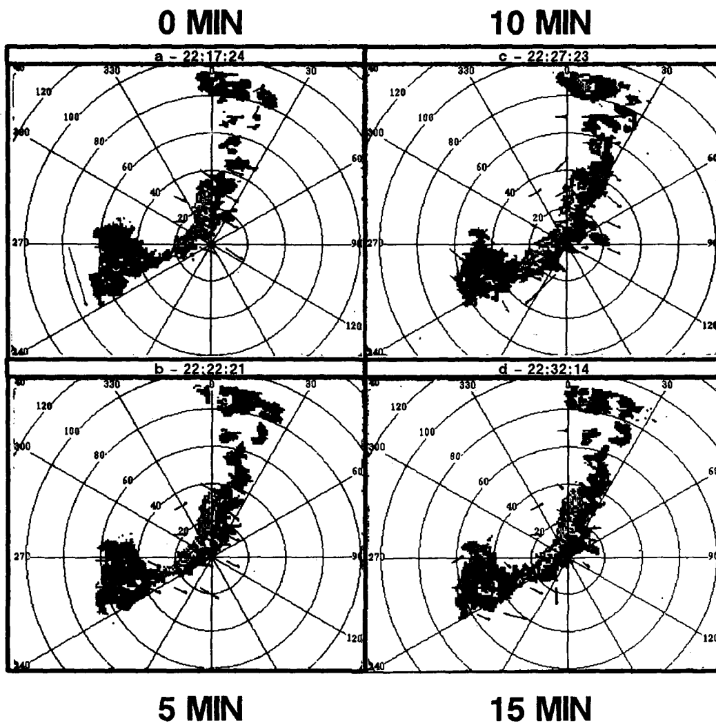
Figure 90. Extrapolation analysis: Jun15, unfiltered vectors.
