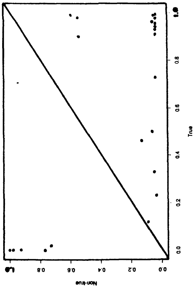
TDNN
