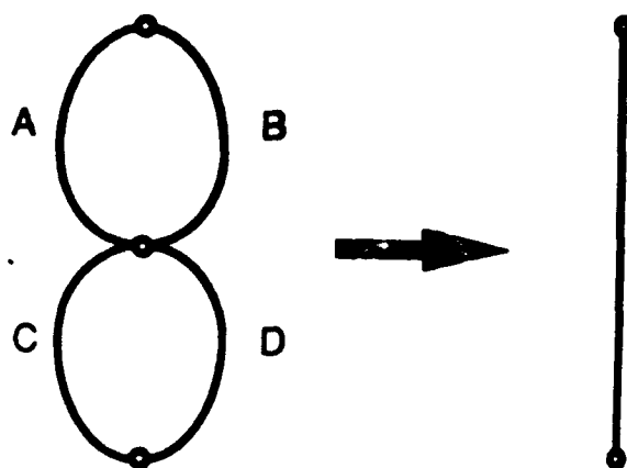
Figure 2.3 Reduction to an equivalent edge
