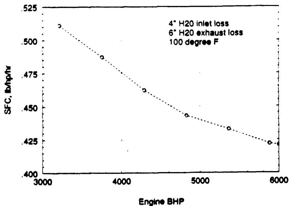
Figure 11 571-KF Engine SFC for Cubic Loading
