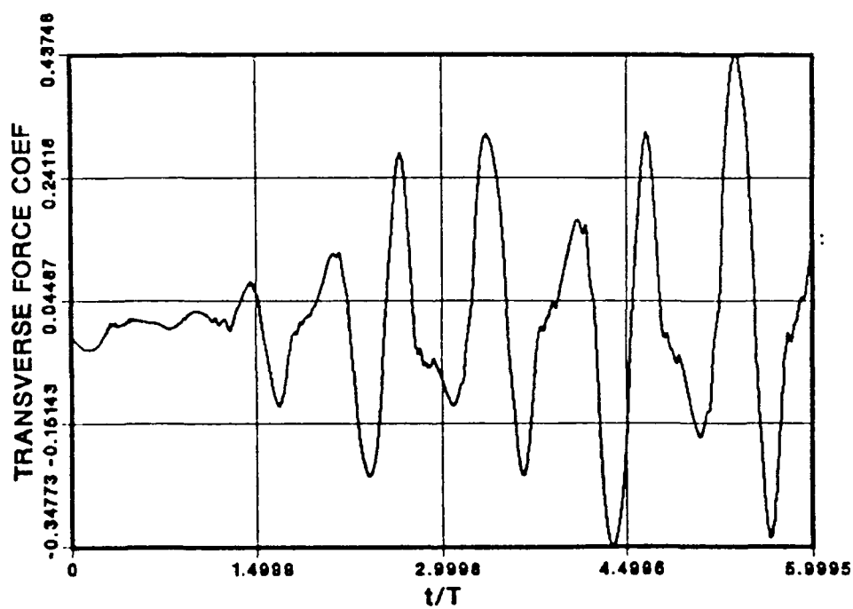
Figure 40. Transverse Force Coefficient, K = 4 , Re = 800 , V_r = 0.65
