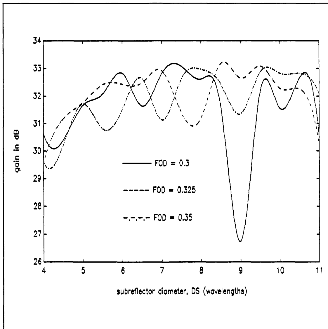
Figure 15: Relative effects of changing some parameters to the antenna performance ( DM=20\lambda ).
