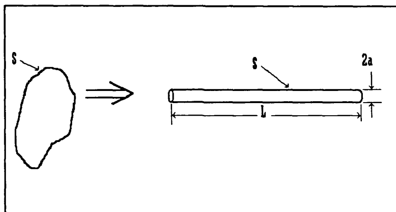
Figure 6: Thin wire approximation.
