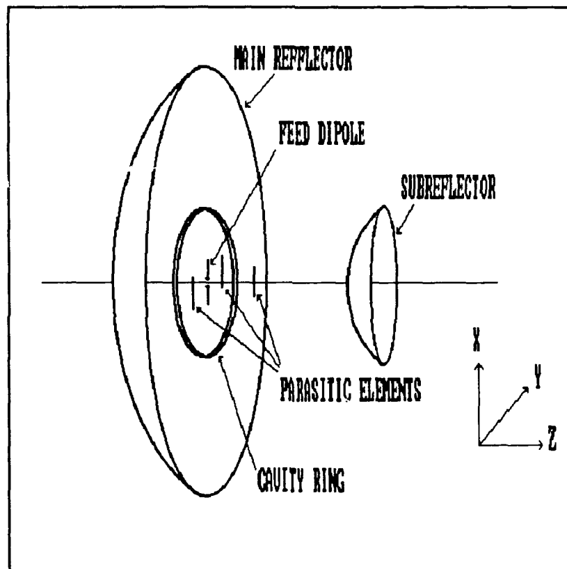
Figure 3: Cassegrain showing designed feed.
