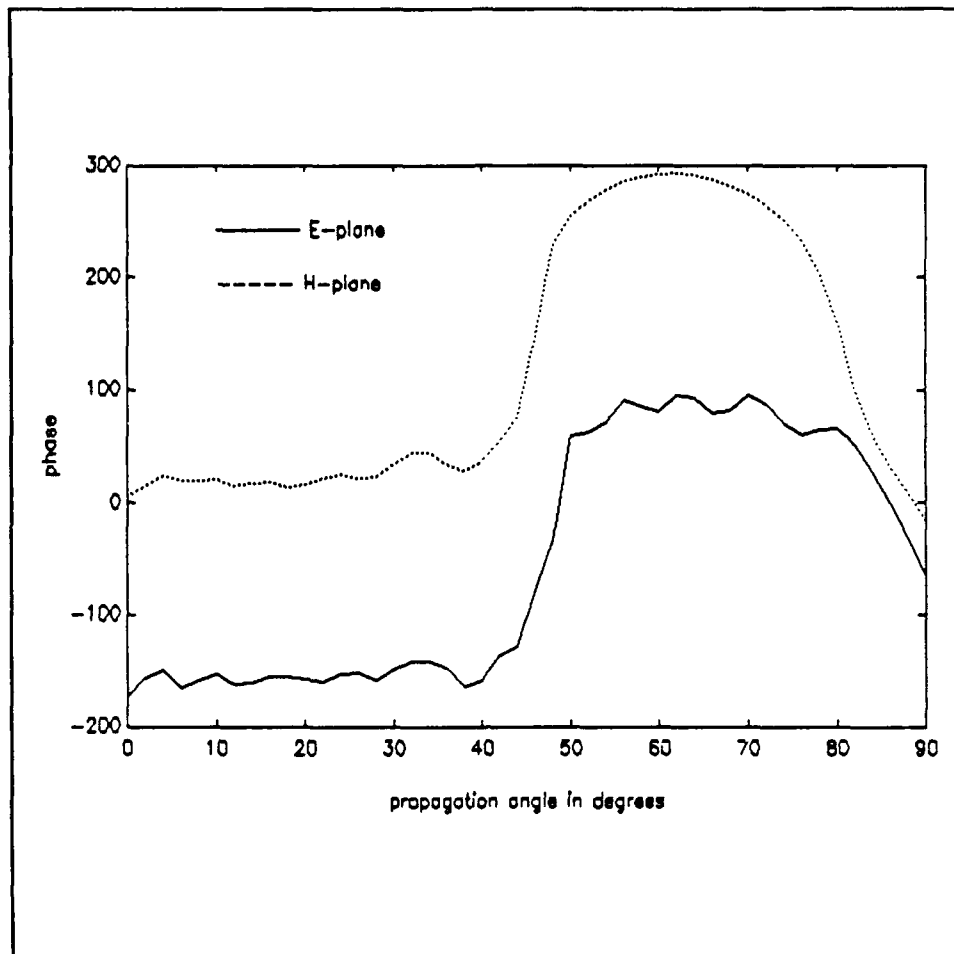
Figure 14: Phase of the feed radiation pattern.
