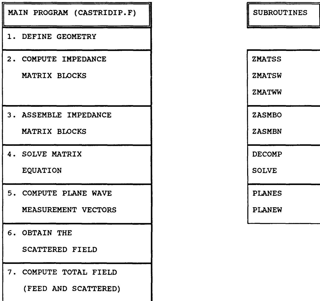
Figure 7: Main program flow chart.
