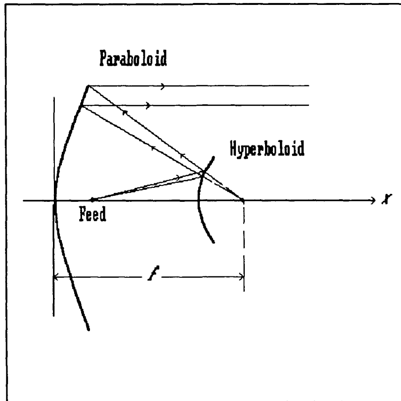
Figure 1: Cassegrain antenna system.
