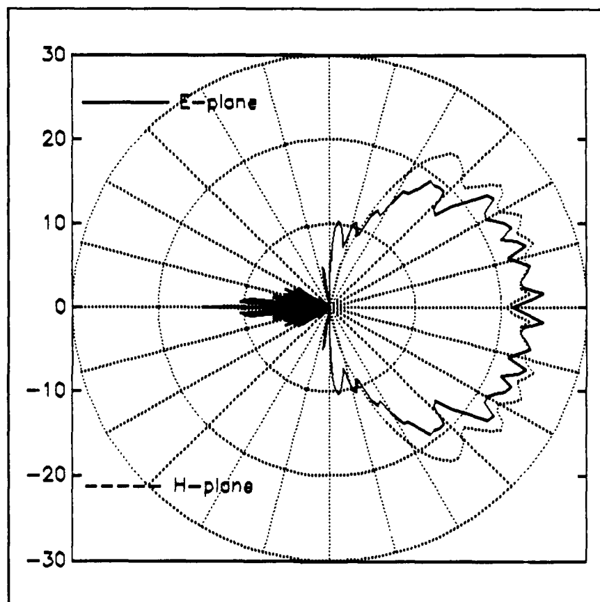
Figure 10: Feed pattern with ring and no parasitic dipoles.
