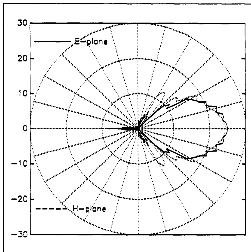
Figure 12: Pattern from fed dipole surrounded by ring and a parasitic director element.
