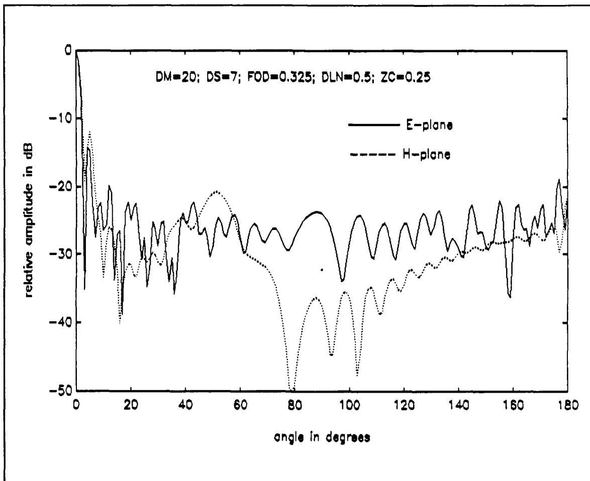
Figure 16: Antenna pattern without parasitic dipole and ring on feed.
