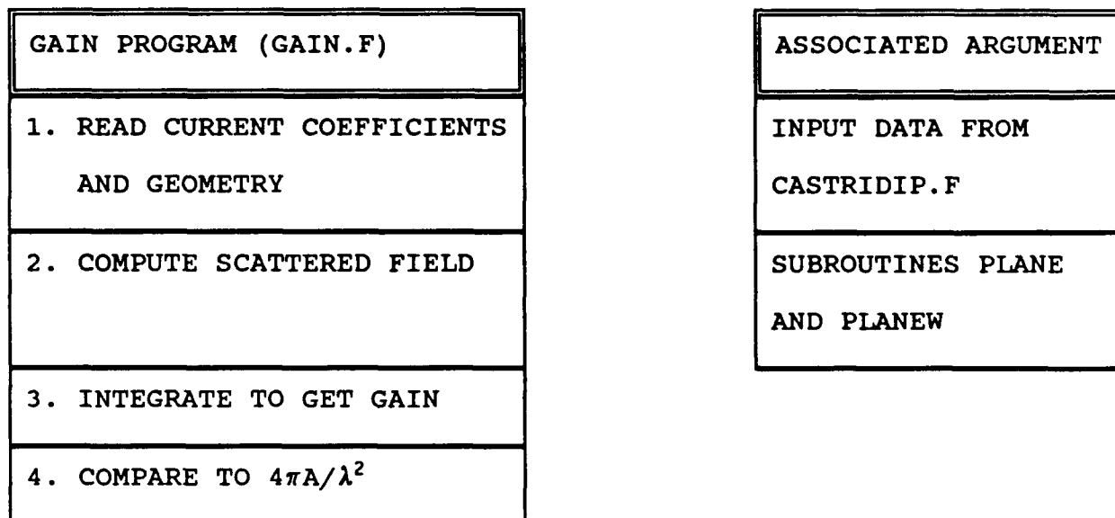
Figure 9: Gain program flow chart.
