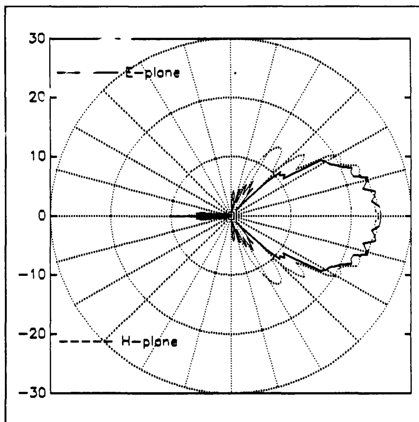
Figure 11: Feed pattern with one parasitic element in front of the fed dipole.
