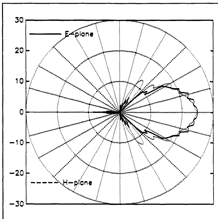
Figure 13: Feed pattern with H-plane dipoles added.
