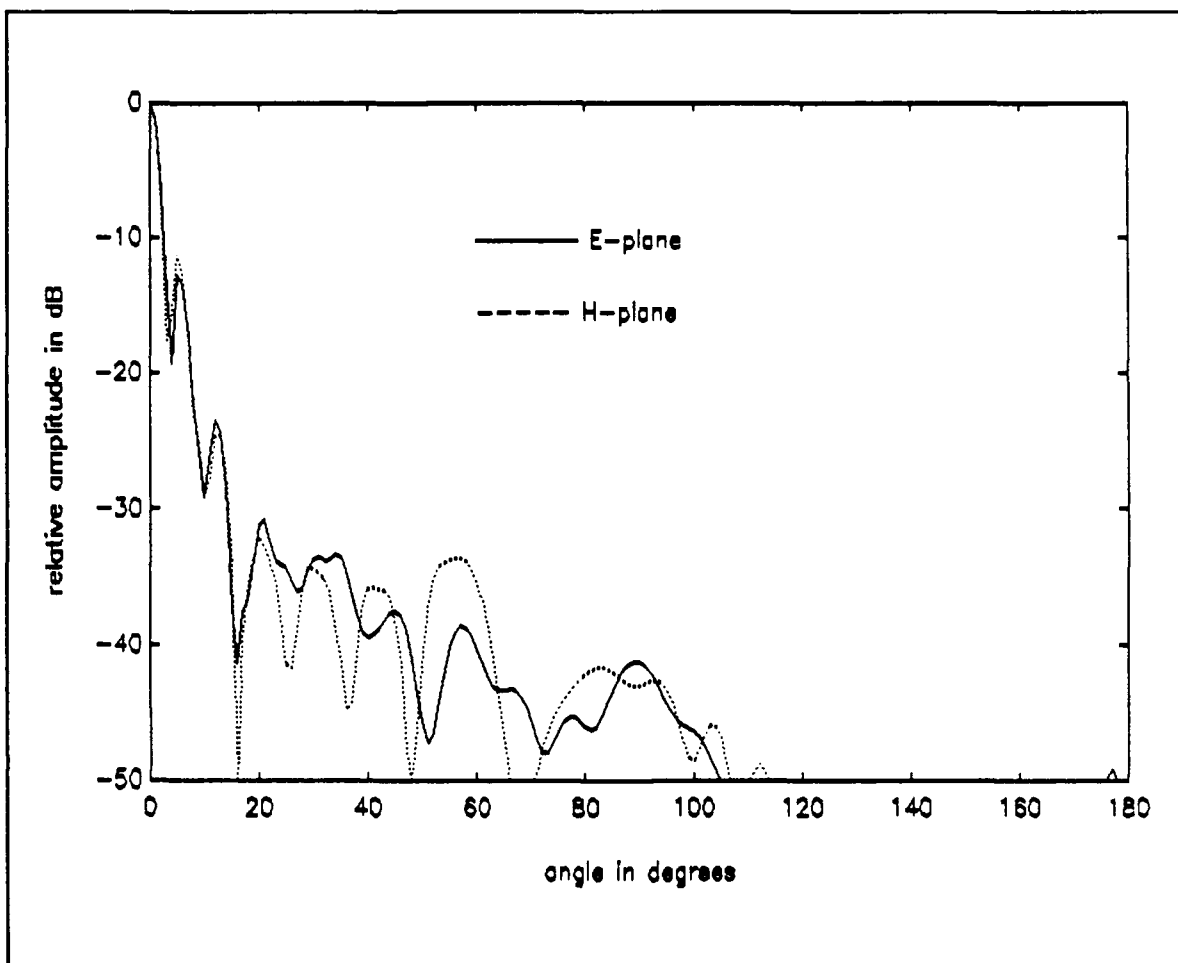
Figure 17: Field pattern for parameters of Table 3.
