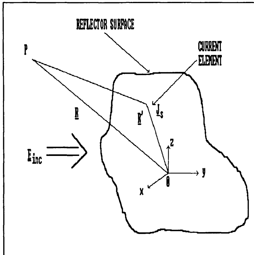
Figure 5: Incident field on perfect conductor.
