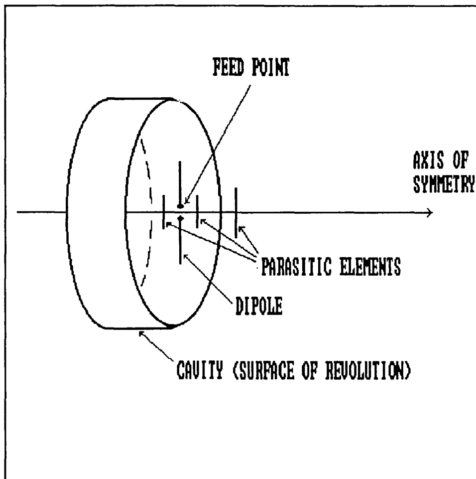
Figure 2: Antenna feed configuration.
