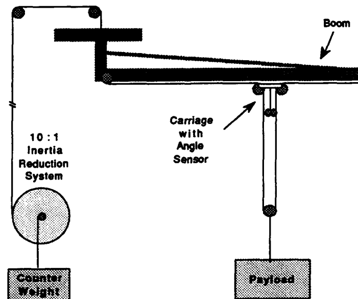
Fig. 1: CMU Gravity Compensation System (GCII)
