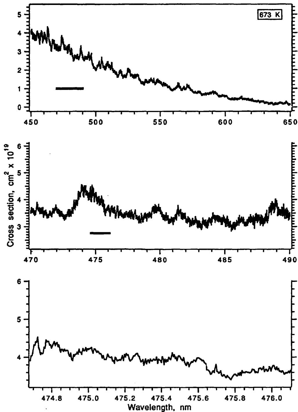
Figure 3. Absolute absorption cross sections at 673K. These data are plotted on the same axes as those in Figure 2, and were recorded at the same resolution. Note the great reduction in sharp features in the spectra.
