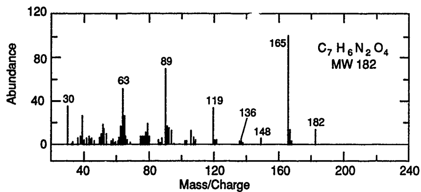
Figure A24. 2,5-DNT.
