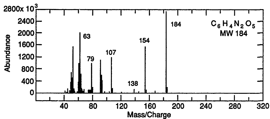
Figure A17. 2,4-Dinitrophenol.
