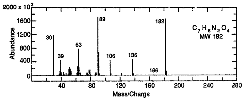
Figure A26. 3,5-DNT.
