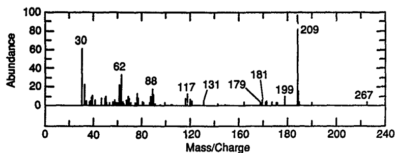
Figure 6. Mass spectrum of compound identified as 2,4-dinitroanthranil.
