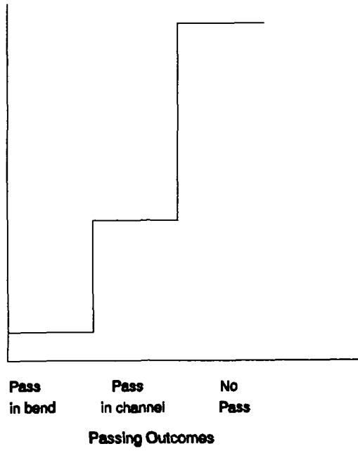
Figure H-2: Graphical Transformation of Random Numbers to Random Values
