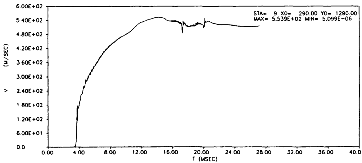
Figure 6. Velocity Histories at Several Lagrangian Stations for a Representative Magazine Simulation Computation.
