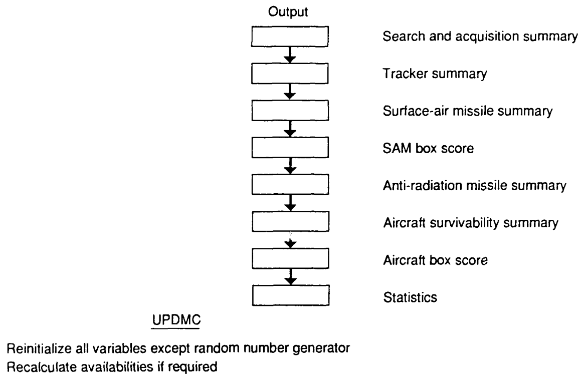
Fig. A.13—Output and Monte Carlo (UPDMC) flow chart
