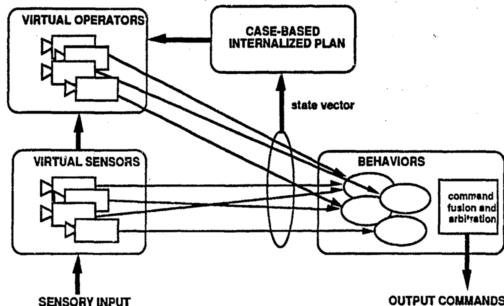
Figure 6: CBIP Architecture
