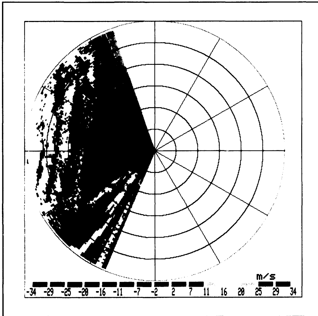
Fig. 5. Same as Fig. 2 except for the 0.5^\circ tilt at 1612 UTC 22 June 1987. Gust front detections are in black.
