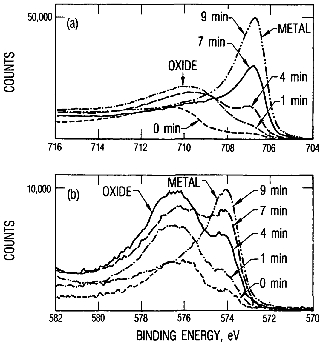
Figure 3. The (a) Fe 2p 3/2 and (b) Cr 2p 3/2 XPS peaks as a function of the sputter times listed on the figure. Note the different scales given for the Fe and Cr spectra, reflecting the differences in peak intensities related to surface concentrations. The oxide and metal peaks are labeled in the figure.
