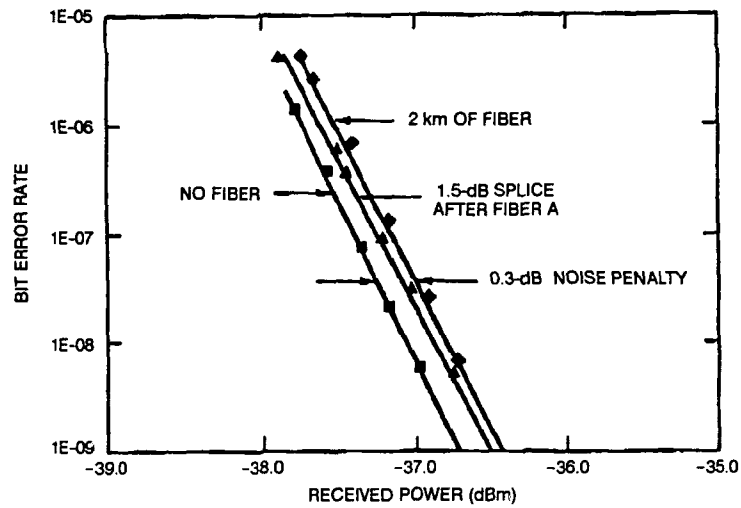
Figure 4. Bit-error-rate measurements for fiber A at a data rate of 200 Mbps and 2^{20}-1 pseudorandom pattern.
