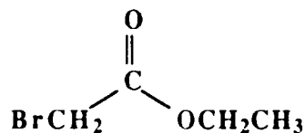
Ethyl bromoacetate (EBA)
