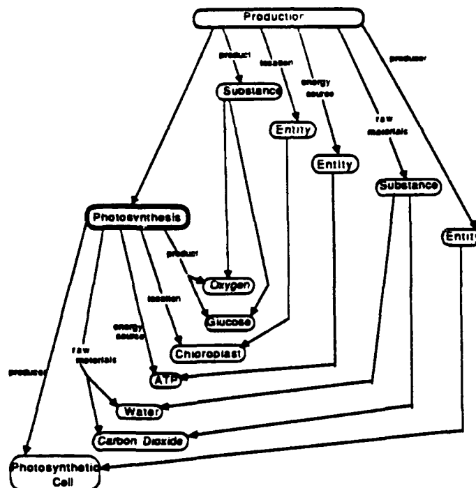
Figure 1: The viewpoint of "photosynthesis as-kind-of production" as extracted from the Botany Knowledge Base by the View Retriever.
