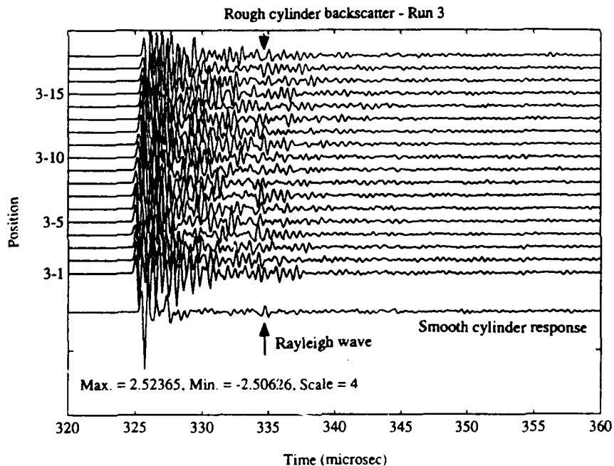
Figure 4-21: Time series for rough cylinder measurements in run 3. A smooth cylinder time series is shown to compare the Rayleigh wave arrival times.
