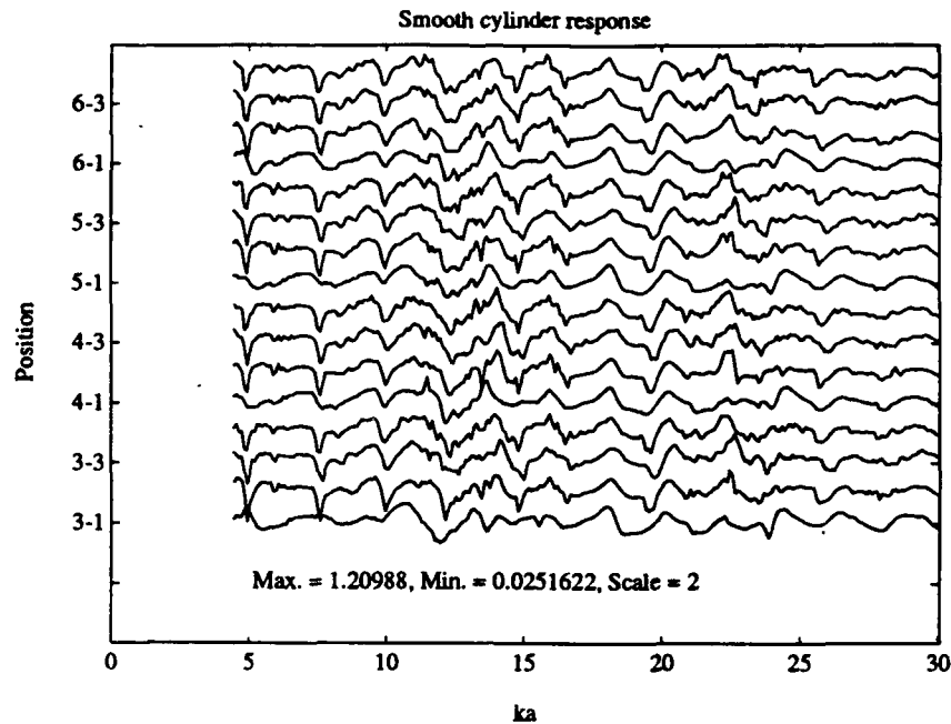
Figure 4-25: Normalized smooth cylinder frequency response measurements. Note missing nulls at ka = 5.0, 8.0, and 10.0 in positions 3-1, 4-1, 5-1, and 6-1 corresponding to measurements taken at a joint between subsections.
