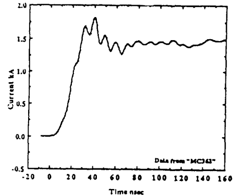
Figure 10 b. BLT current in 6.5 ohm PFN showing <18nsec risetime.
