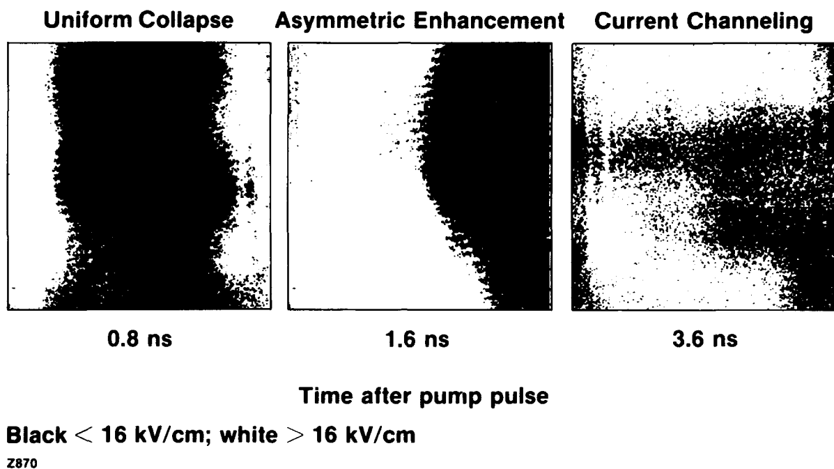
Fig. 8 The time evolution of the electric field in a photoconductive switch showing the development of low field channels within the switch.
