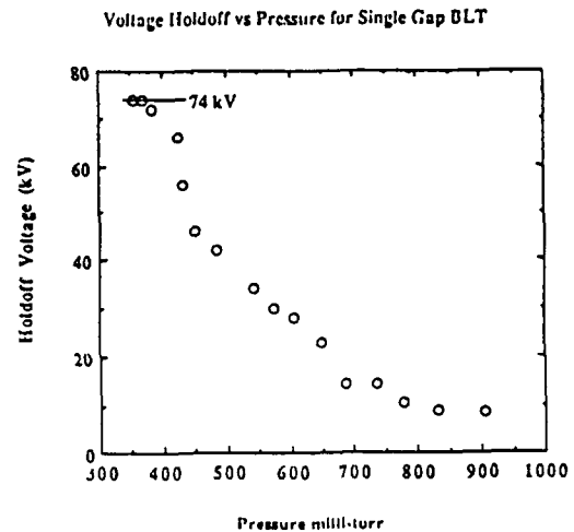
Figure 4. Voltage holdoff vs gas pressure in a pulse charged single gap BLT switch.
