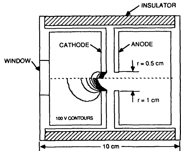
Figure 2. Schematic of the optically triggered pseudospark switch which consists of an opposing cylindrical hollow cathode and anode with central holes. The device is triggered by UV illumination through the window and typically operates at gas pressures of < 1 Torr. Two views are shown having cathode hole radii of 0.5 cm and 1 cm. Electric potential contours (0 - 1 kV, 100 V spacing) are shown for a holdoff voltage of 10 kV. More potential penetration into the cathode occurs with the larger hole.
