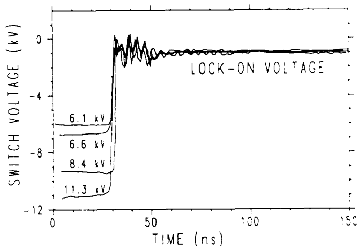
Fig. 4. High field switching of a 2 mm long GaAs switch. This plot shows a constant lock-on voltage for various initial charging voltages. The switch was triggered into this lock-on state with a 10 ns wide laser pulse at 26 ns. The switch continues to conduct until the energy is dumped from the circuit and a 5 kV/cm lock-on field can no longer be maintained.
