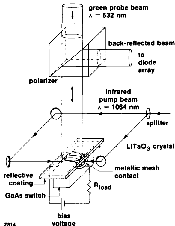
Fig. 2 Bulk switch configuration.
