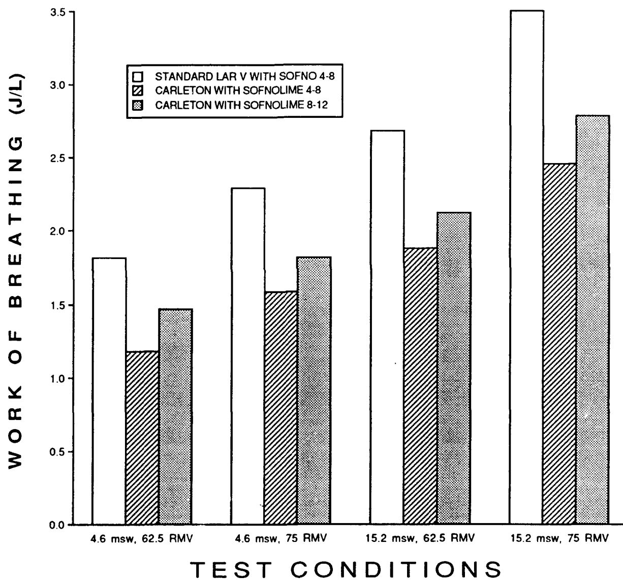
Figure 2. Work of Breathing in LAR V Using Standard LAR V Mouthpiece, Compared to the Carleton Mouthpiece Using 4-8 and 8-12 Sofnolime
